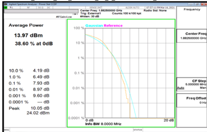
Band25_15MHz_DFT_256QAM_75_0_MidCH376500_MidCH376500
