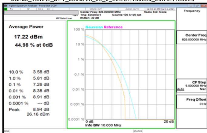
Band5_10MHz_DFT_256QAM_50_0_MidCH167300_MidCH167300
