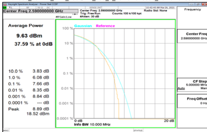
Band38_40MHz_DFT_256QAM_100_0_LowCH518000_LowCH518000
