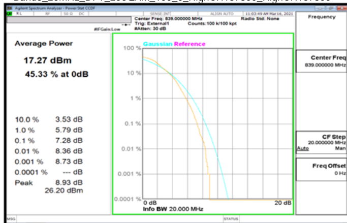
Band5_20MHz_DFT_256QAM_100_0_HighCH167800_HighCH167800
