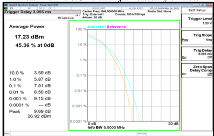
Band5_5MHz_DFT_256QAM_25_0_HighCH169300_HighCH169300
