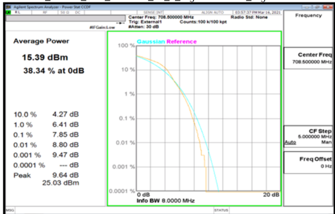
Band12_15MHz_DFT_256QAM_75_0_HighCH141700_HighCH141700
