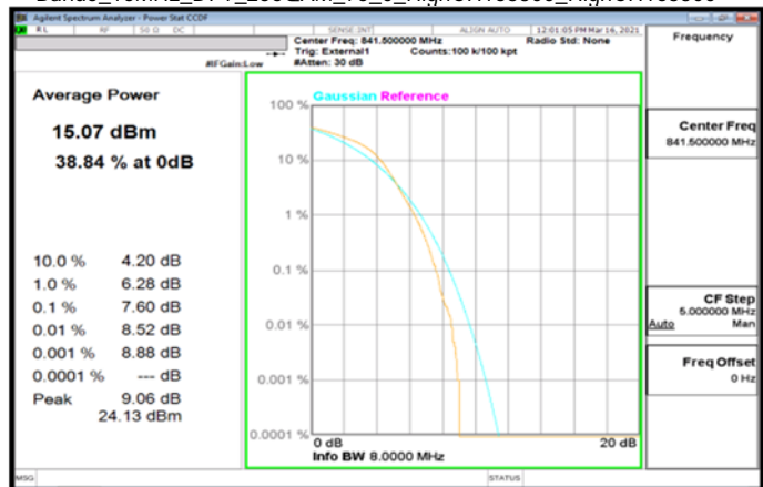
Band5_15MHz_DFT_256QAM_75_0_HighCH168300_HighCH168300
