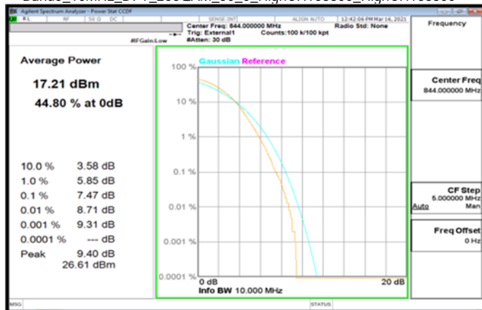
Band5_10MHz_DFT_256QAM_50_0_HighCH168800_HighCH168800
