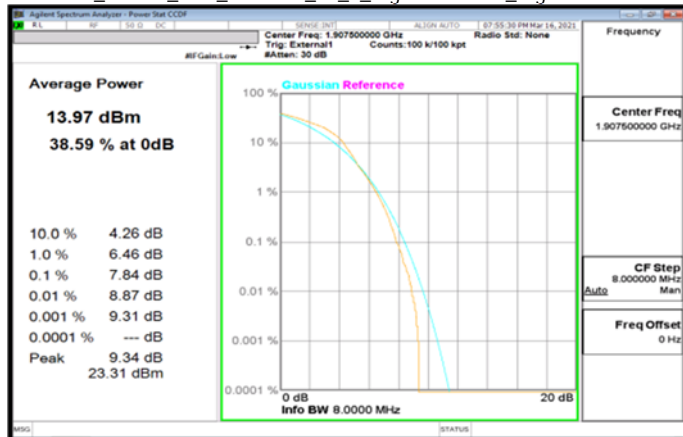
Band25_15MHz_DFT_256QAM_75_0_HighCH381500_HighCH381500
