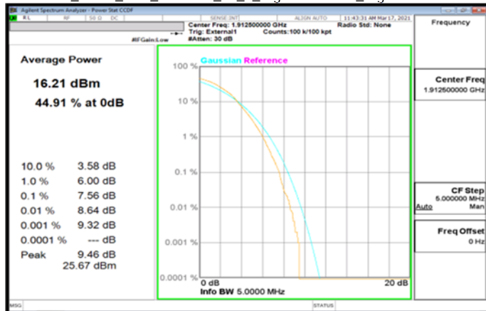
Band25_5MHz_DFT_256QAM_25_0_HighCH382500_HighCH382500
