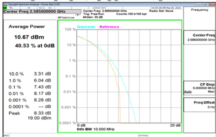
Band38_30MHz_DFT_256QAM_75_0_LowCH517000_LowCH517000
