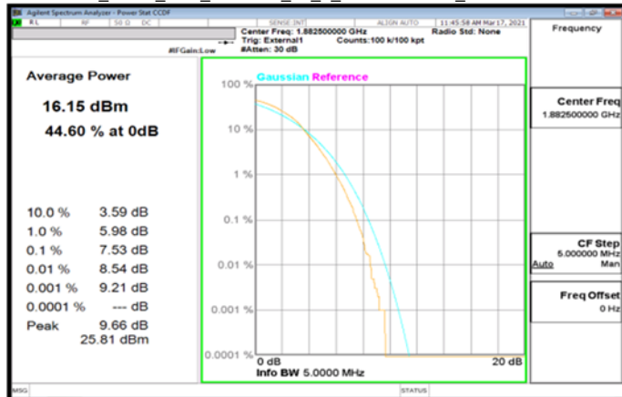
Band25_5MHz_DFT_256QAM_25_0_MidCH376500_MidCH376500
