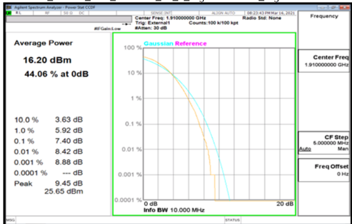
Band25_10MHz_DFT_256QAM_50_0_HighCH382000_HighCH382000
