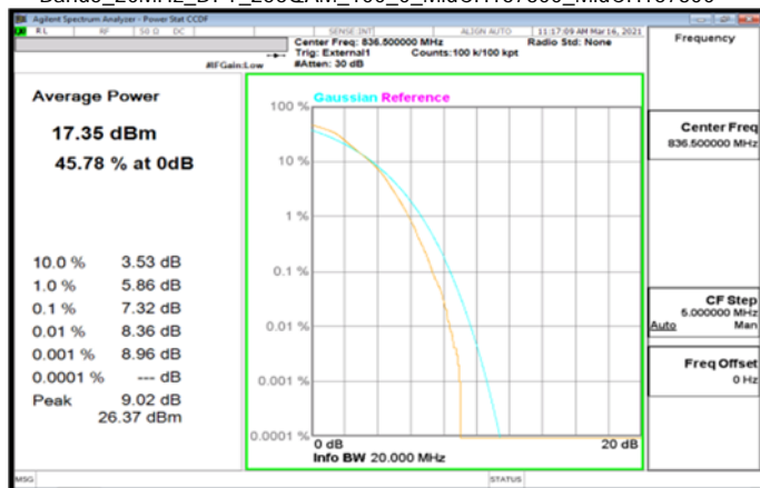
Band5_20MHz_DFT_256QAM_100_0_MidCH167300_MidCH167300
