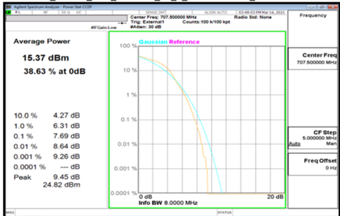
Band12_15MHz_DFT_256QAM_75_0_MidCH141500_MidCH141500
