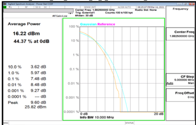
Band25_10MHz_DFT_256QAM_50_0_MidCH376500_MidCH376500
