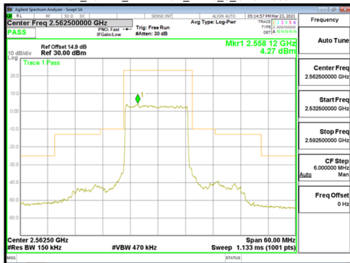
Band7_15MHz_DFT-BPSK_RB75_0_CH512500
