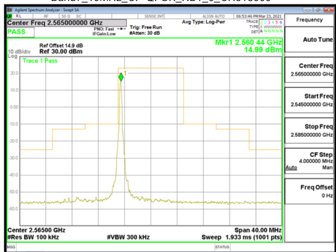
Band7_10MHz_CP-QPSK_RB1_0_CH513000
