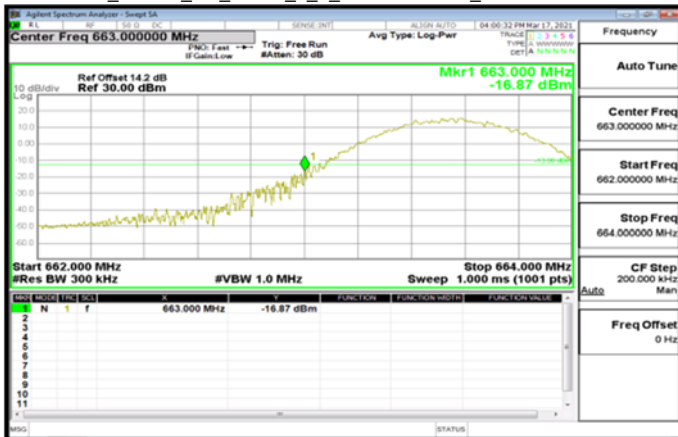
Band71_20MHz_CP_QPSK_1_0_LowCH134600_LowCH134600
