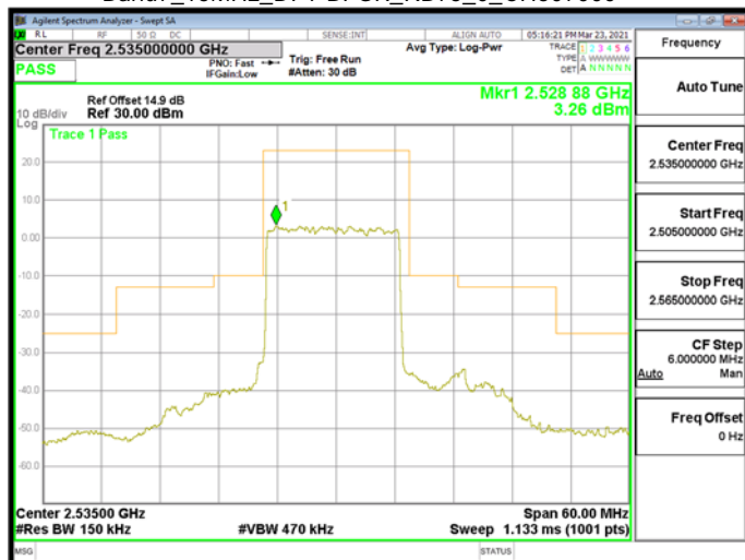
Band7_15MHz_DFT-BPSK_RB75_0_CH507000
