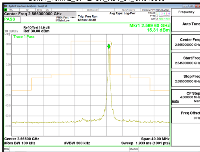
Band7_10MHz_CP-QPSK_RB1_51_CH513000
