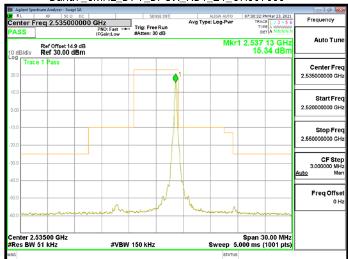
Band7_5MHz_DFT_BPSK_RB1_24_CH513500
