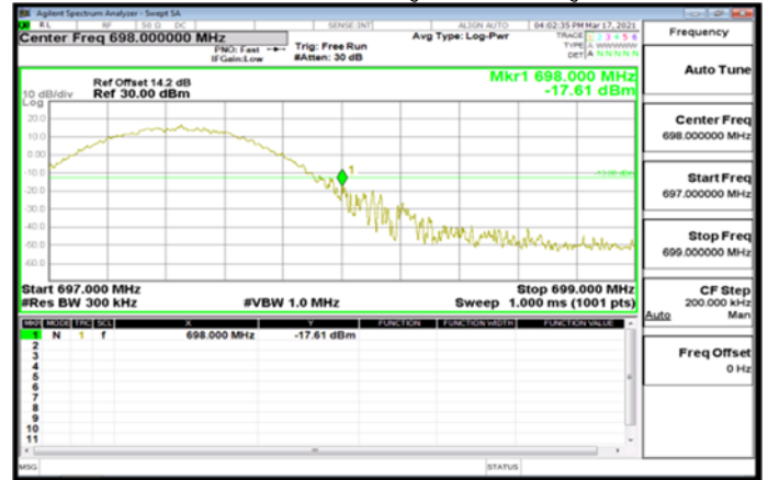
Band71_20MHz_CP_QPSK_1_105_HighCH137600_HighCH137600
