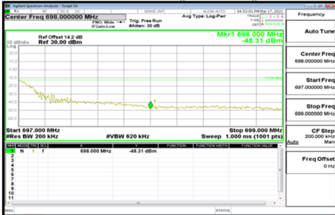
Band71_15MHz_DFT_BPSK_75_0_HighCH138100_HighCH138100
