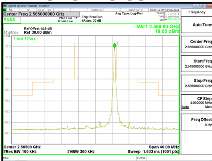
Band7_10MHz_DFT-BPSK_RB1_51_CH513000
