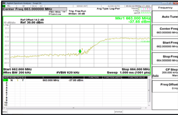
Band71_15MHz_DFT_BPSK_75_0_LowCH134100_LowCH134100
