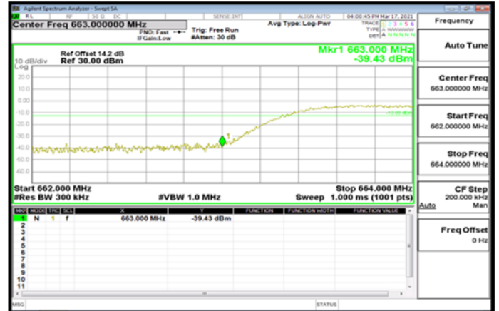
Band71_20MHz_CP_QPSK_106_0_LowCH134600_LowCH134600
