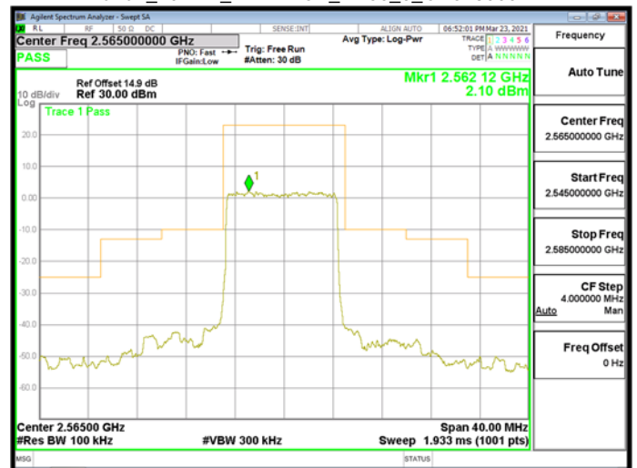
Band7_10MHz_DFT-BPSK_RB50_0_CH513000
