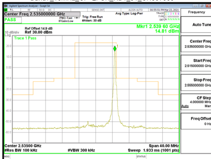
Band7_10MHz_CP-QPSK_RB1_51_CH507000
