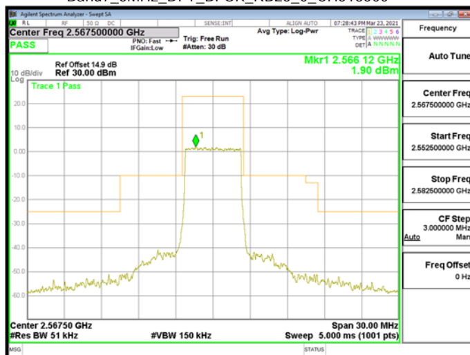
Band7_5MHz_DFT_BPSK_RB25_0_CH513500
