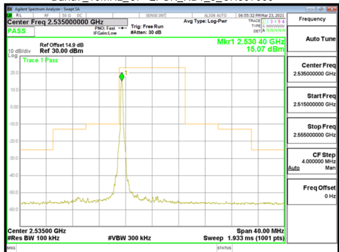
Band7_10MHz_CP-QPSK_RB1_0_CH507000
