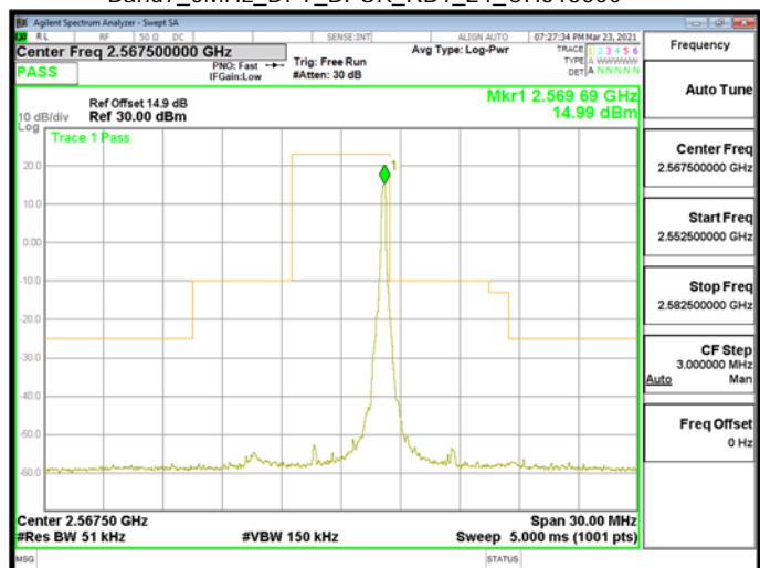
Band7_5MHz_DFT_BPSK_RB1_24_CH513500
