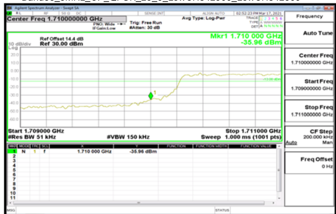
Band66_5MHz_CP_QPSK_25_0_LowCH342500_LowCH342500
