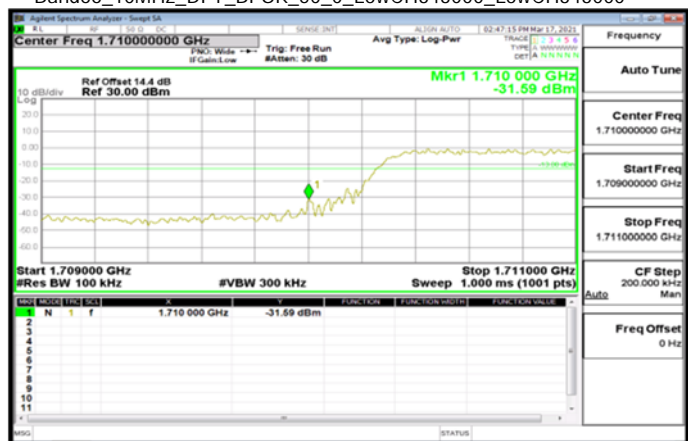
Band66_10MHz_DFT_BPSK_50_0_LowCH343000_LowCH343000
