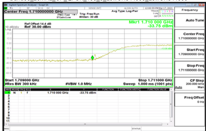
Band66_20MHz_CP_QPSK_106_0_LowCH344000_LowCH344000
