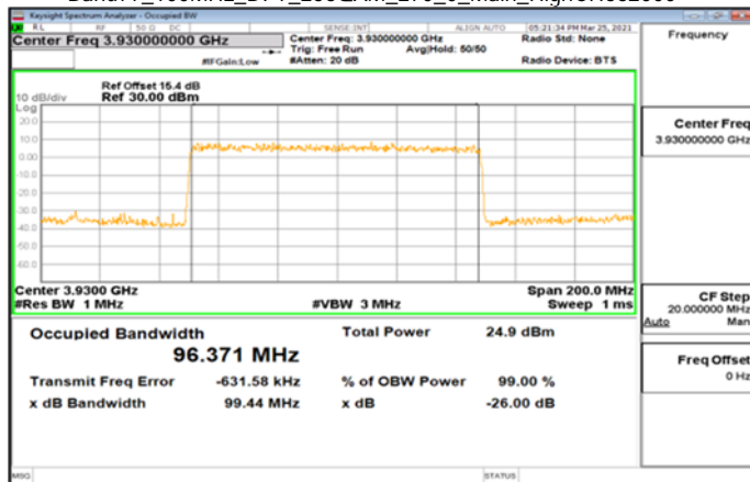
Band77_100MHz_DFT_256QAM_270_0_Main_HighCH662000
