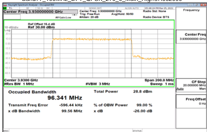
Band77_100MHz_DFT_QPSK_270_0_Main_HighCH662000
