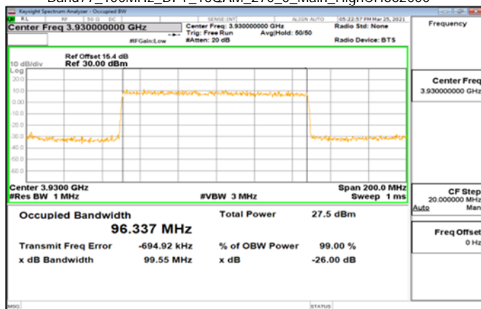
Band77_100MHz_DFT_16QAM_270_0_Main_HighCH662000
