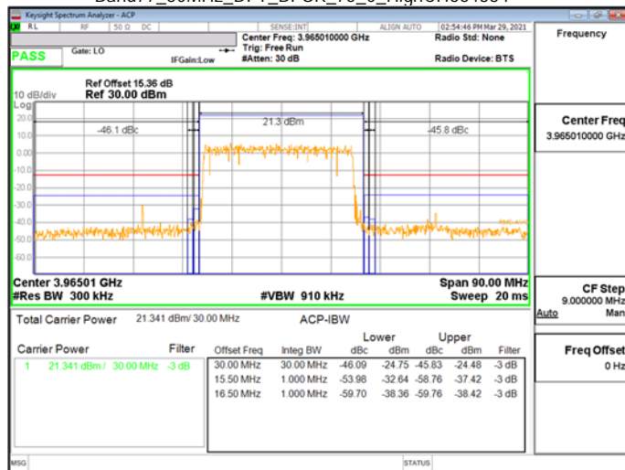
Band77_30MHz_DFT_BPSK_75_0_HighCH664334
