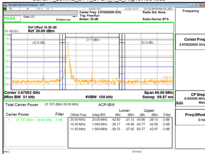
Band77_20MHz_DFT_BPSK_1_0_HighCH664668
