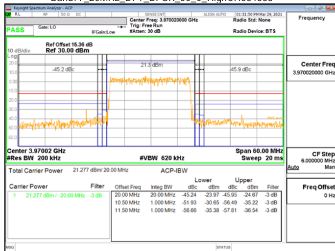
Band77_20MHz_DFT_BPSK_50_0_HighCH664668
