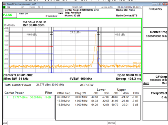
Band77_30MHz_DFT_BPSK_1_77_HighCH664334
