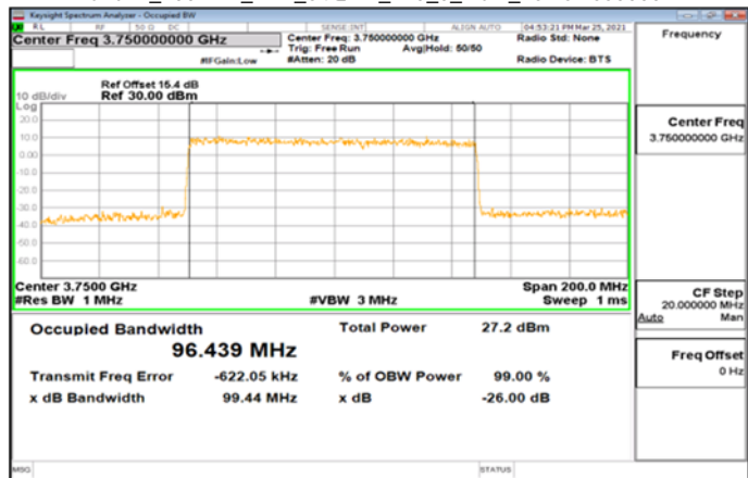
Band77 100MHz DFT 64QAM 270 0 Main MidCH656000
