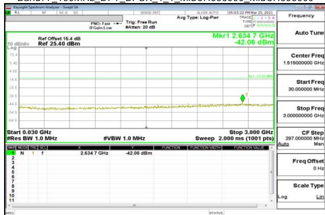
Band77_100MHz_DFT_BPSK_1_1_MidCH656000_MidCH656000
