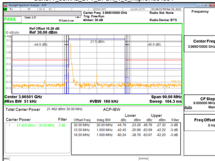
Band77_30MHz_DFT_BPSK_1_0_HighCH664334
