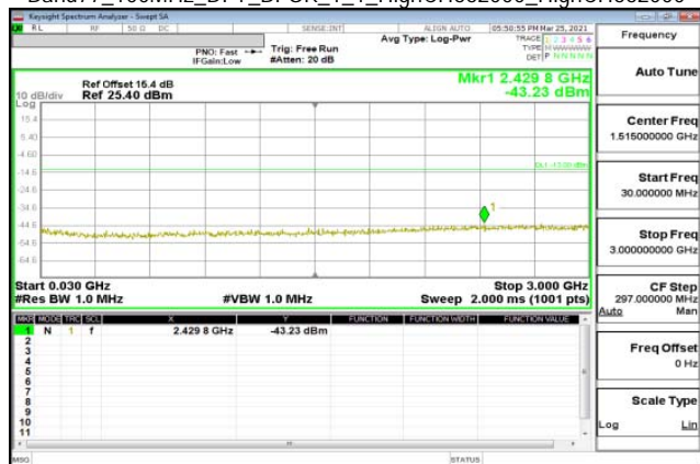
Band77_100MHz_DFT_BPSK_1_1_HighCH662000_HighCH662000
