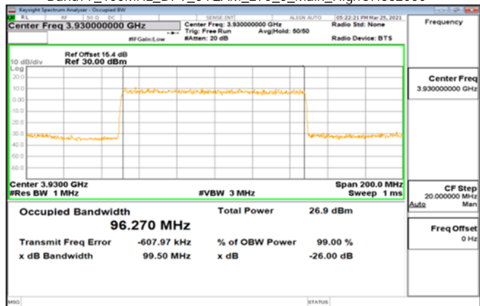
Band77_100MHz_DFT_64QAM_270_0_Main_HighCH662000
