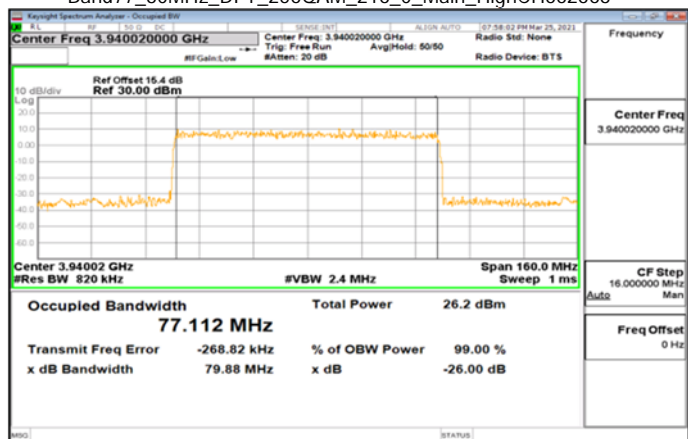
Band77_80MHz_DFT_256QAM_216_0_Main_HighCH662668
