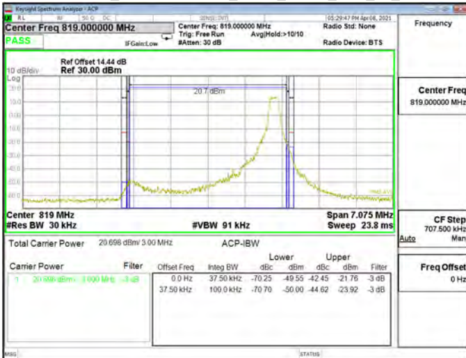
Emission Mask_Band26-Part90s_3MHz_QPSK_RB1_14_CH26775
