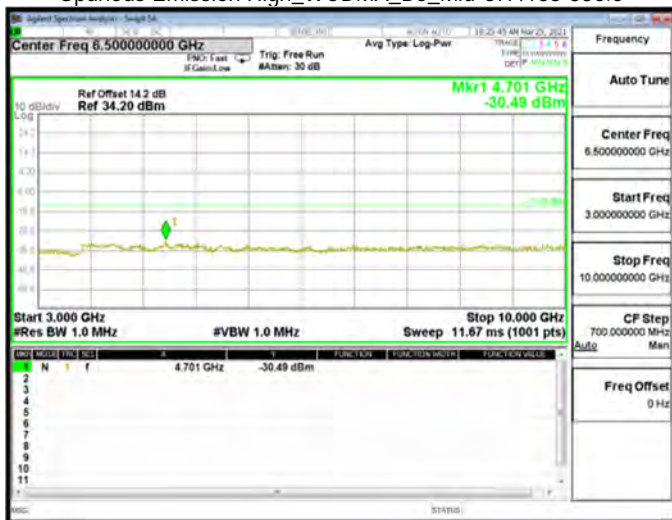
Spurious Emission High_WCDMA_B5_Mid CH4183-836.6
