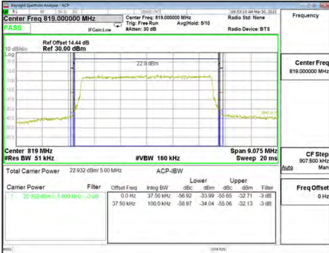
Emission Mask_Band26-Part90s_5MHz_QPSK_RB25_0_CH26765
