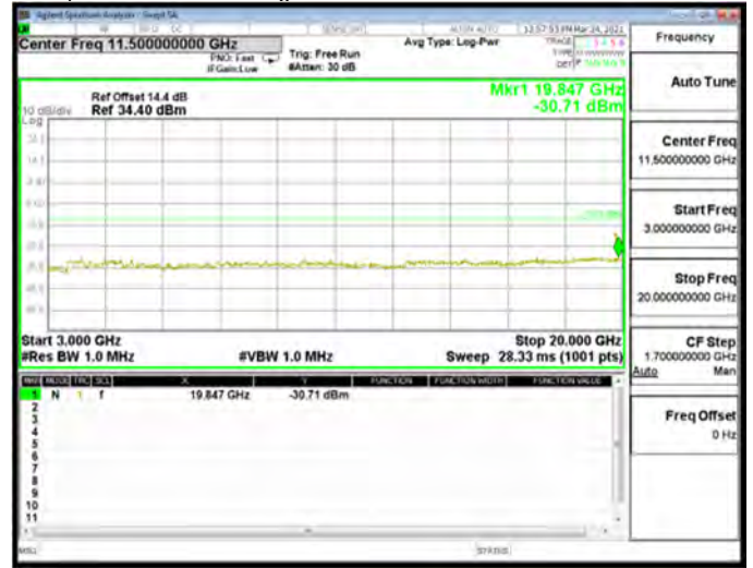
Spurious Emission High_GSM_1900MHz_Mid CH661-1880
