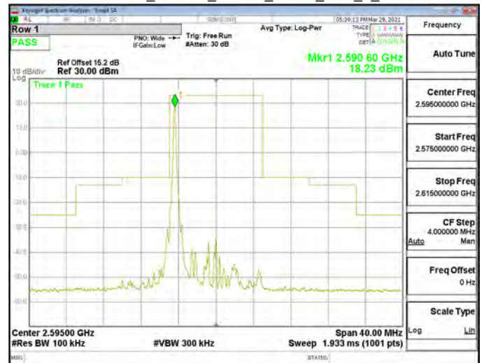
Emission Mask_Band38_10MHz_QPSK_RB1_0_CH38200
