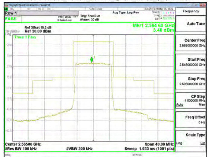
Emission Mask_Band7_10MHz_QPSK_RB50_0_CH21400
