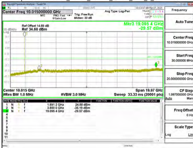
Spurious Emission_Band2_20MHz_QPSK_RB1_0_CH19100
