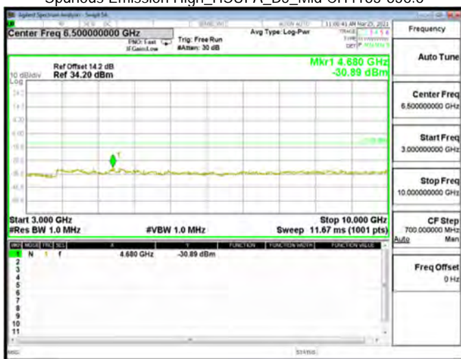
Spurious Emission High_HSUPA_B5_Mid CH4183-836.6
