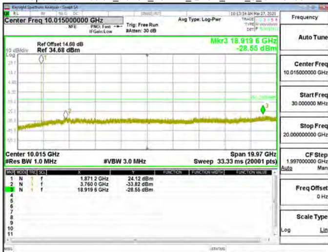
Spurious Emission_Band2_20MHz_QPSK_RB1_0_CH19100
