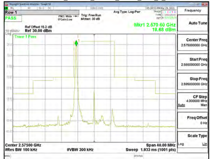
Emission Mask_Band38_10MHz_QPSK_RB1_0_CH38000
