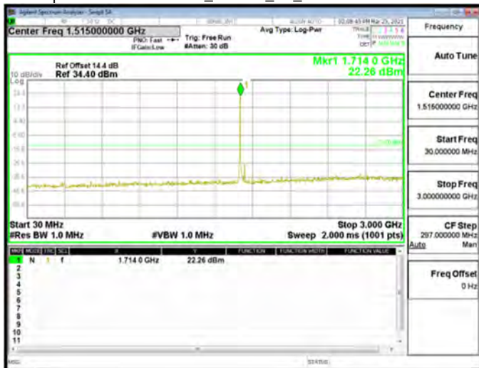
Spurious Emission Low_HSDPA_B4_Mid CH1413-1732.6
