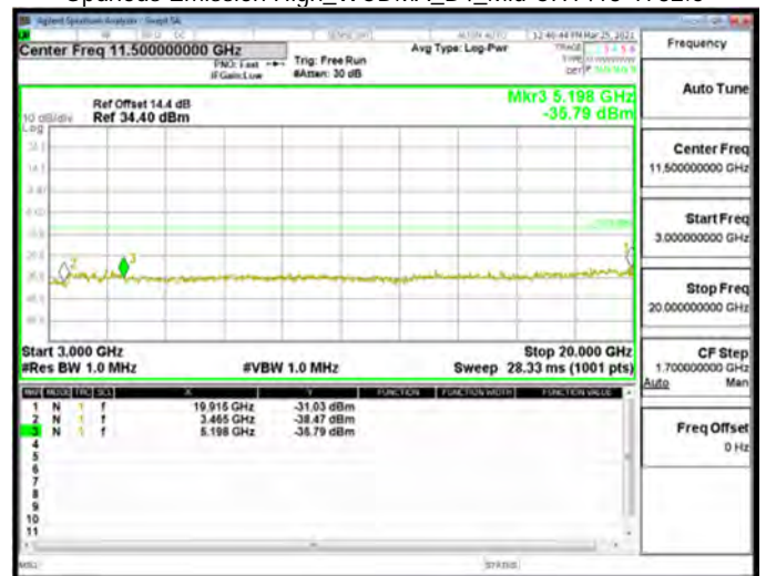
Spurious Emission High_WCDMA_B4_Mid CH1413-1732.6
