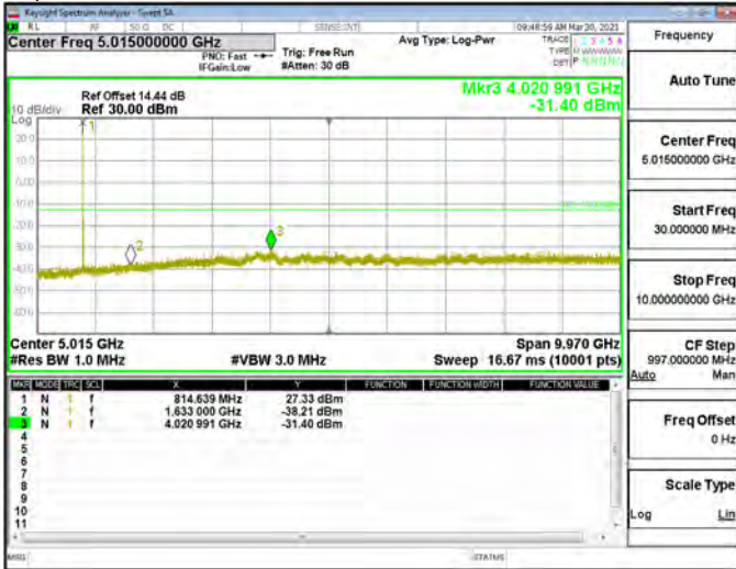
Spurious Emission_Band26-Part90s_5MHz_QPSK_RB1_0_CH26740
