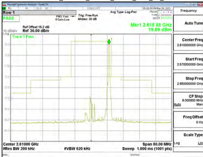
Emission Mask_Band38_20MHz_QPSK_RB1_99_CH38150
