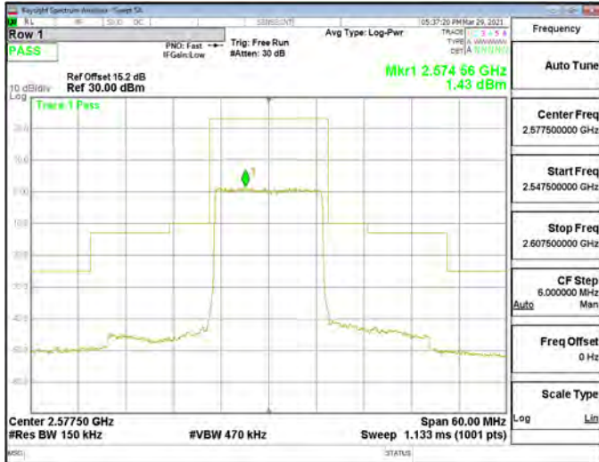
Emission Mask_Band38_15MHz_QPSK_RB75_0_CH38000
