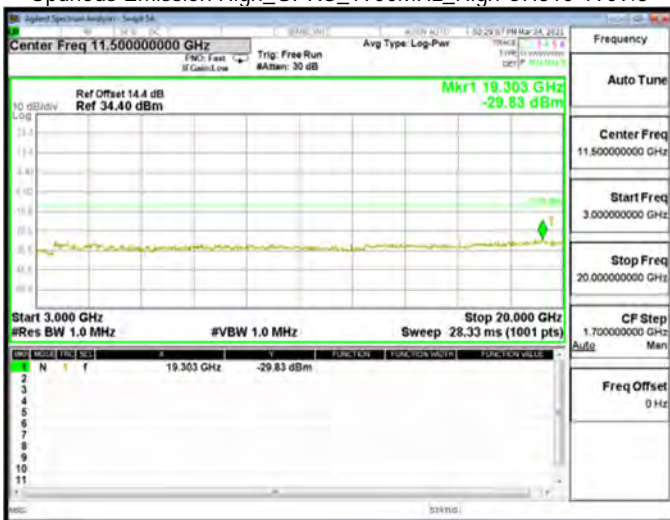
Spurious Emission High_GPRS_1900MHz_High CH810-1909.8
