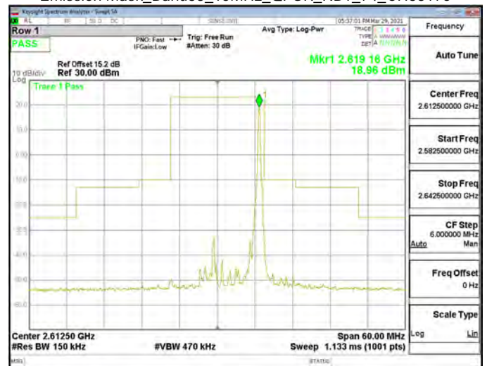
Emission Mask_Band38_15MHz_QPSK_RB1_74_CH38175
