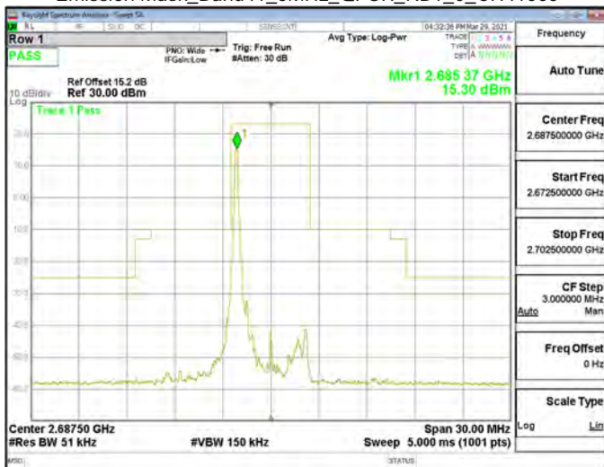
Emission Mask_Band41_5MHz_QPSK_RB1_0_CH41565
