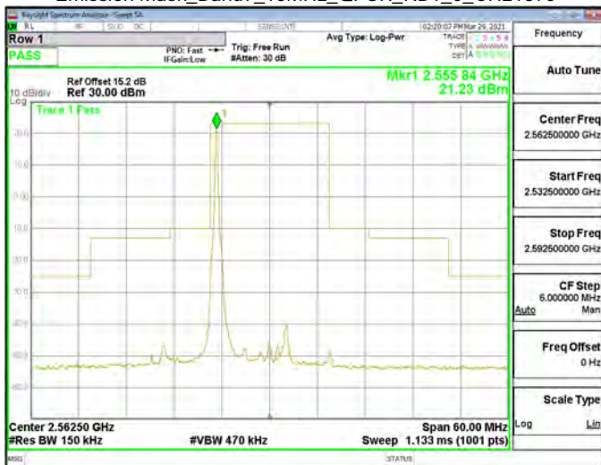
Emission Mask_Band7_15MHz_QPSK_RB1_0_CH21375
