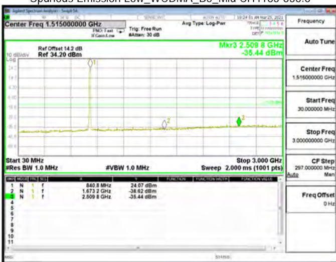
Spurious Emission Low_WCDMA_B5_Mid CH4183-836.6
