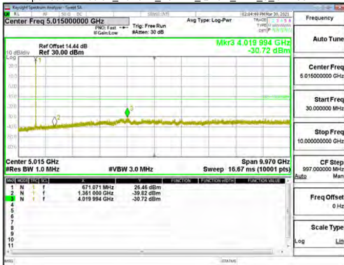
Spurious Emission_Band71_20MHz_QPSK_RB1_0_CH133297
