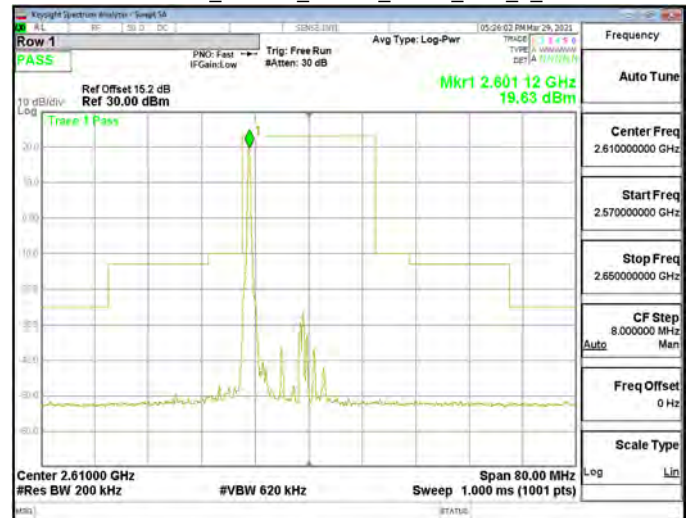
Emission Mask_Band38_20MHz_QPSK_RB1_0_CH38150
