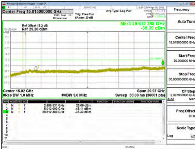
Spurious Emission_Band41_20MHz_QPSK_RB1_0_CH40620
