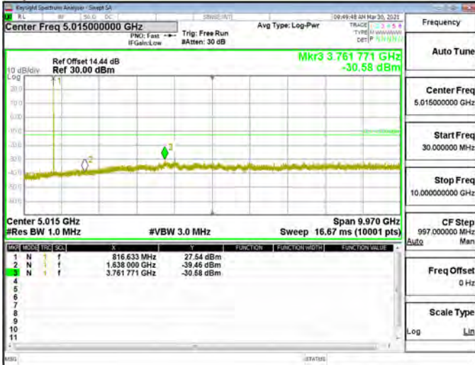
Spurious Emission_Band26-Part90s_5MHz_QPSK_RB1_0_CH26765
