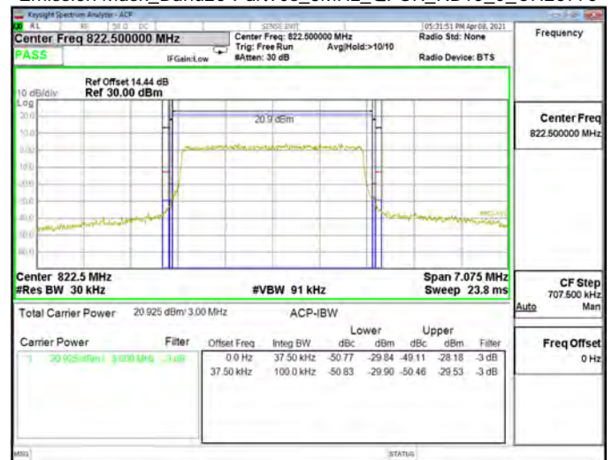
Emission Mask_Band26-Part90s_3MHz_QPSK_RB15_0_CH26775
