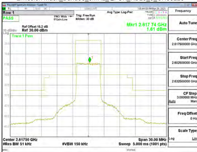
Emission Mask_Band38_5MHz_QPSK_RB25_0_CH38225
