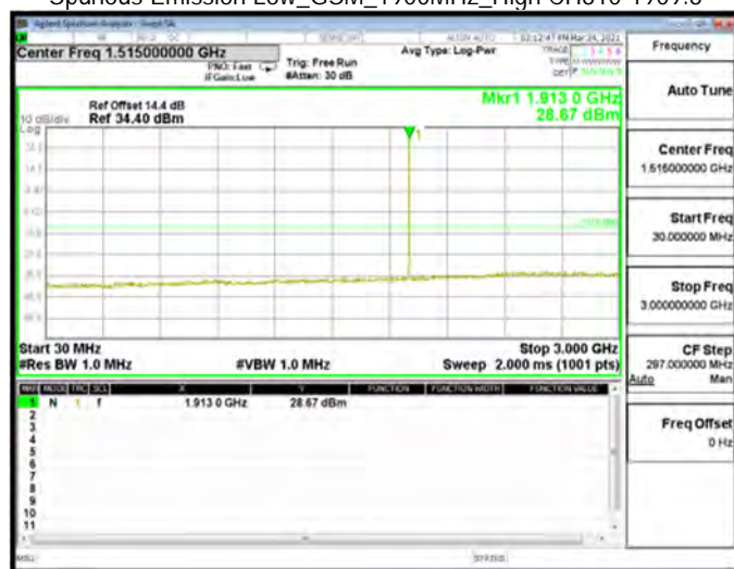
Spurious Emission Low_GSM_1900MHz_High CH810-1909.8
