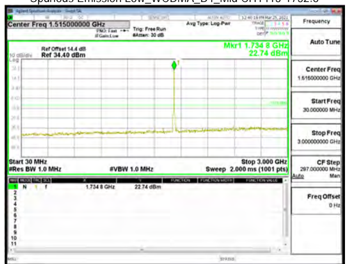
Spurious Emission Low_WCDMA_B4_Mid CH1413-1732.6
