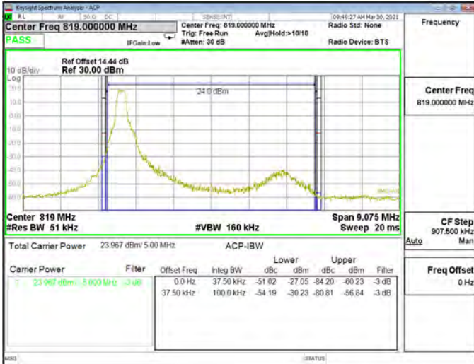
Emission Mask_Band26-Part90s_5MHz_QPSK_RB1_0_CH26765
