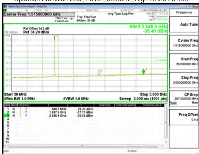
Spurious Emission Low_EDGE_850MHz_High CH251-848.8
