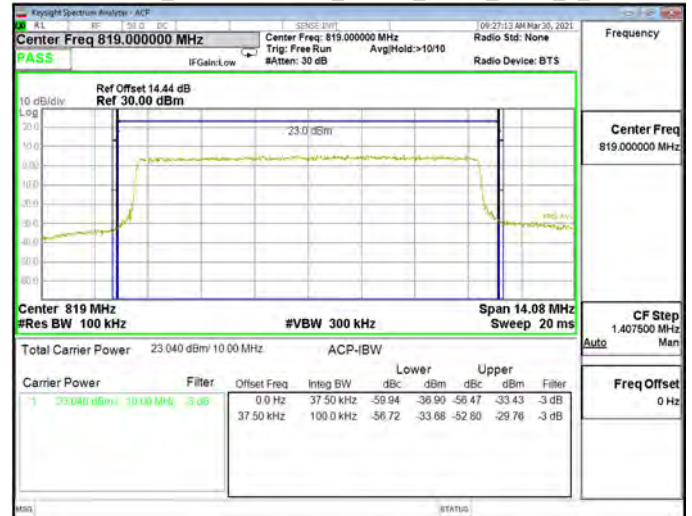
Emission Mask_Band26-Part90s_10MHz_QPSK_RB50_0_CH26740
