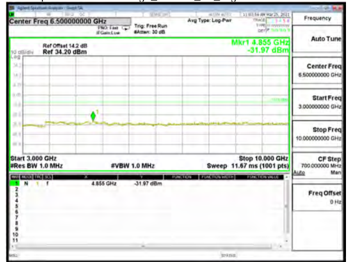
Spurious Emission High_HSUPA_B5_High CH4233-846.6
