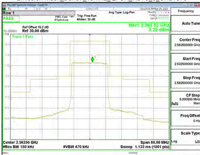
Emission Mask_Band7_15MHz_QPSK_RB75_0_CH21375
