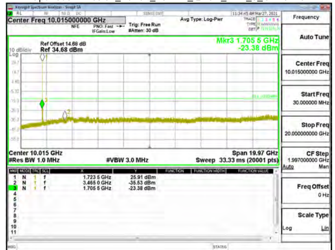
Spurious Emission_Band4_20MHz_QPSK_RB1_0_CH20300
