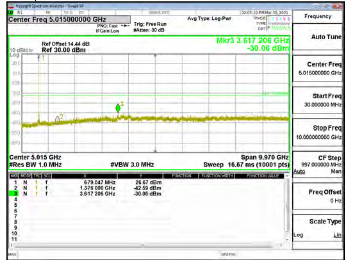
Spurious Emission_Band71_20MHz_QPSK_RB1_0_CH133372
