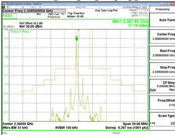
Emission Mask_Band30_5MHz_QPSK_RB1_0_CH27735
