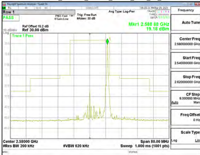
Emission Mask_Band38_20MHz_QPSK_RB1_99_CH38000
