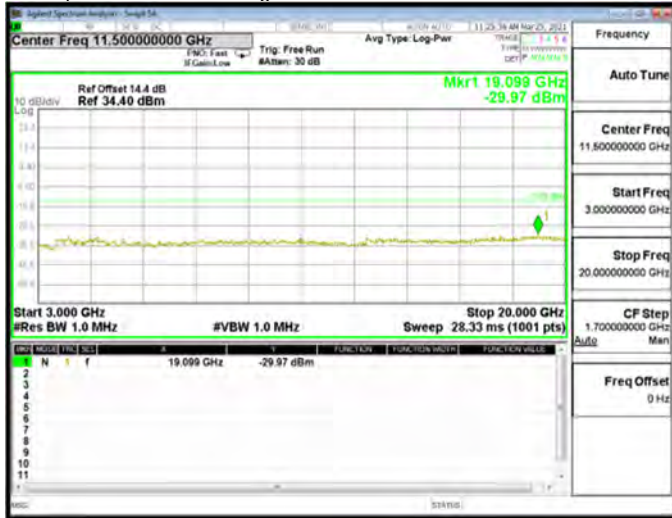
Spurious Emission High_WCDMA_B2_Mid CH9400-1880
