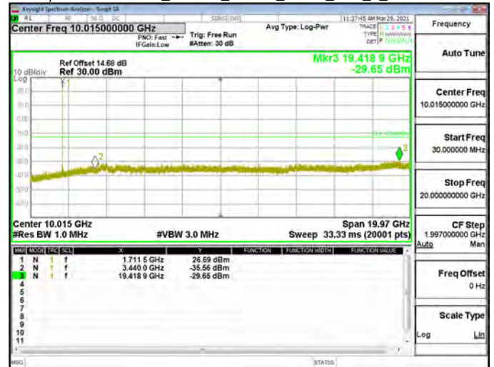
Spurious Emission_Band66_20MHz_QPSK_RB1_0_CH132322
