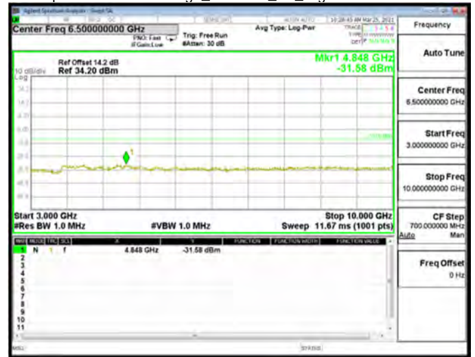
Spurious Emission High_HSDPA_B5_Low CH4132-826.4
