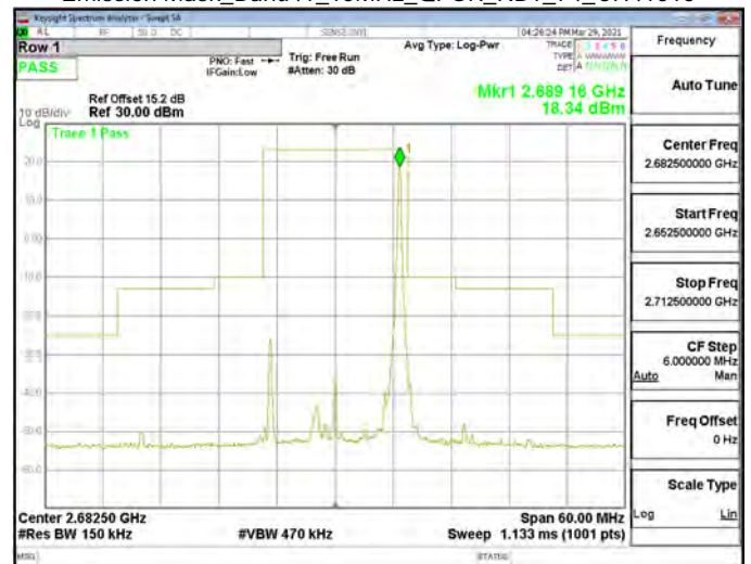
Emission Mask_Band41_15MHz_QPSK_RB1_74_CH41515
