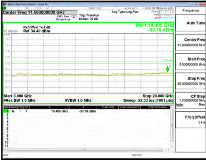
Spurious Emission High_GPRS_1900MHz_Mid CH661-1880
