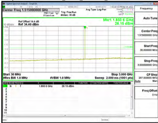
Spurious Emission Low_GPRS_1900MHz_Mid CH661-1880
