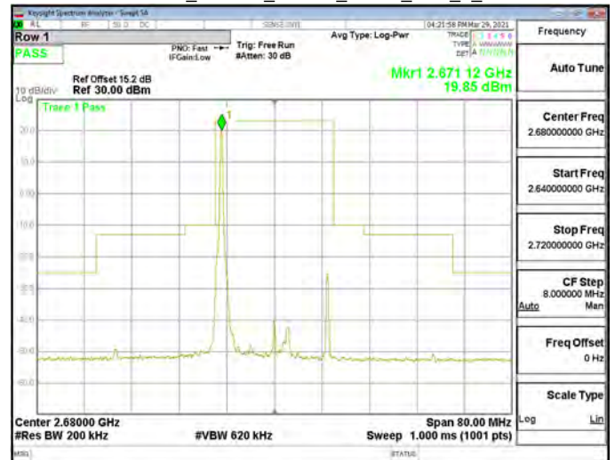
Emission Mask_Band41_20MHz_QPSK_RB1_0_CH41490
