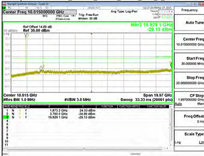
Spurious Emission_Band25_20MHz_QPSK_RB1_0_CH26590
