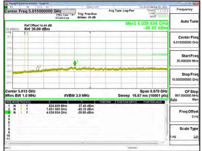
Spurious Emission_Band26_3MHz_QPSK_RB1_0_CH26915
