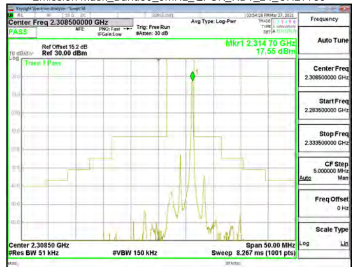
Emission Mask_Band30_5MHz_QPSK_RB1_24_CH27735
