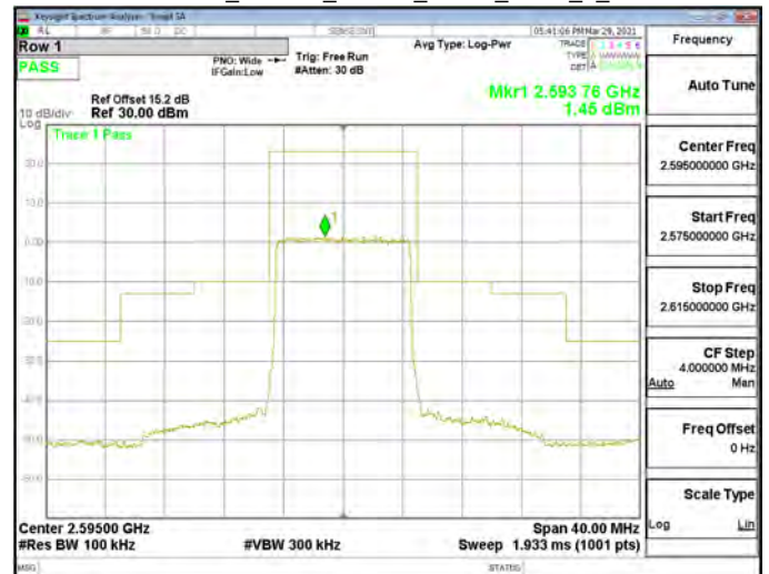
Emission Mask_Band38_10MHz_QPSK_RB50_0_CH38200
