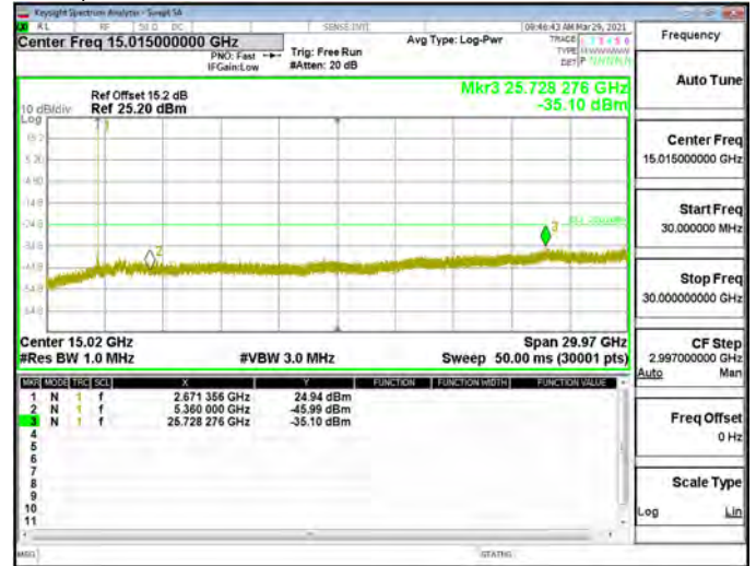
Spurious Emission_Band66_20MHz_QPSK_RB1_0_CH132072
