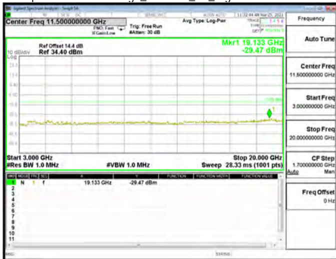
Spurious Emission High_WCDMA_B2_High CH9538-1907.6
