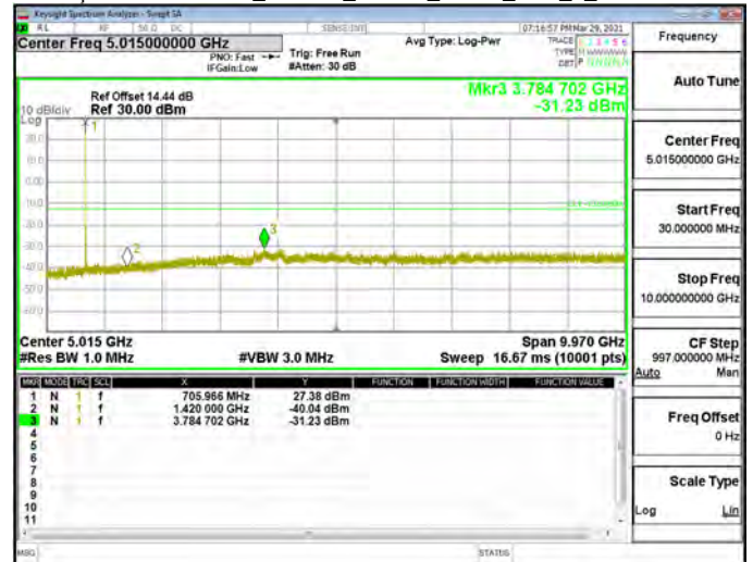
Spurious Emission_Band17_10MHz_QPSK_RB1_0_CH23800
