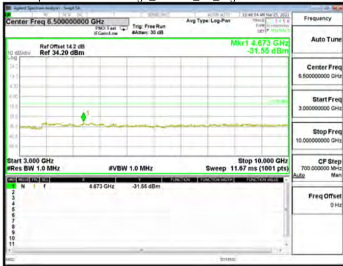
Spurious Emission High_HSUPA_B5_Low CH4132-826.4
