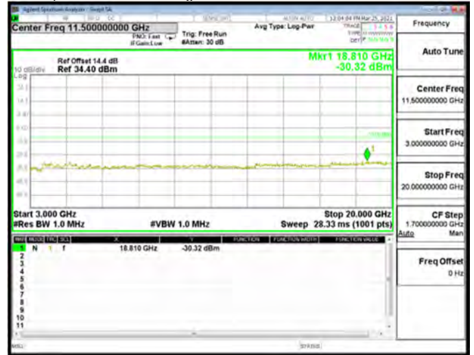
Spurious Emission High_HSDPA_B2_Mid CH9400-1880
