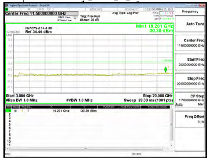
Spurious Emission High_WCDMA_B4_Low CH1312-1712.4
