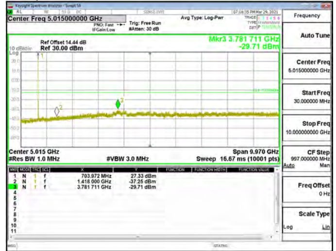
Spurious Emission_Band17_10MHz_QPSK_RB1_0_CH23790
