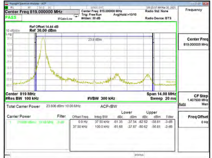
Emission Mask_Band26-Part90s_10MHz_QPSK_RB1_49_CH26740
