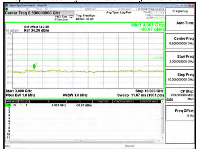
Spurious Emission High_GPRS_850MHz_High CH251-848.8
