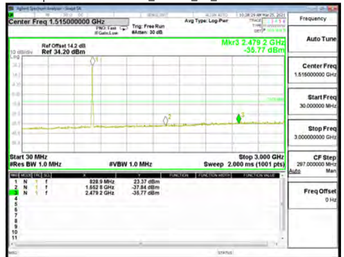
Spurious Emission Low_HSDPA_B5_Mid CH4183-836.6
