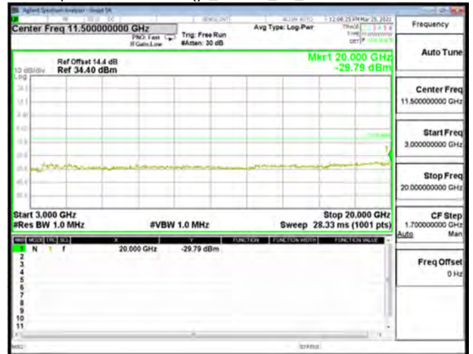
Spurious Emission High_HSDPA_B2_High CH9538-1907.6
