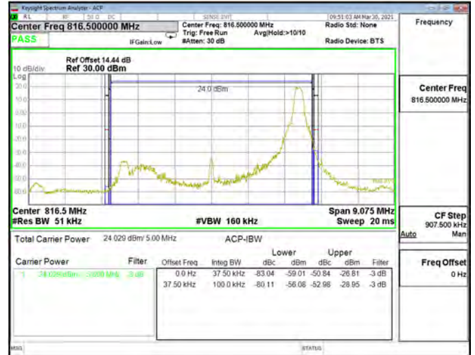
Emission Mask_Band26-Part90s_5MHz_QPSK_RB1_24_CH26740
