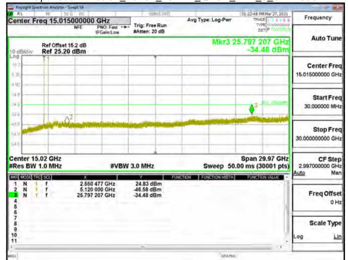
Spurious Emission_Band7_20MHz_QPSK_RB1_0_CH21350
