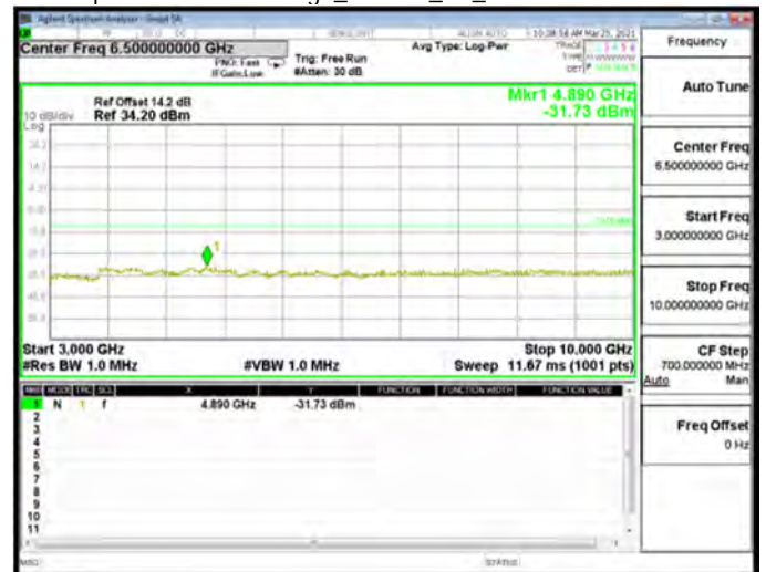
Spurious Emission High_HSDPA_B5_Mid CH4183-836.6
