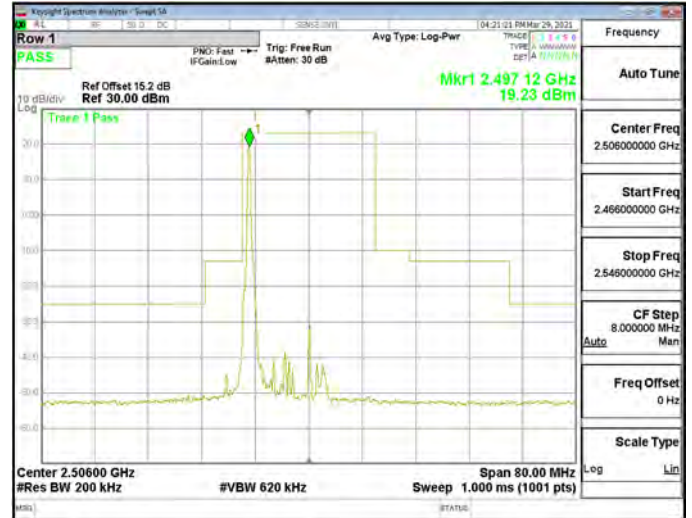
Emission Mask_Band41_20MHz_QPSK_RB1_0_CH40620
