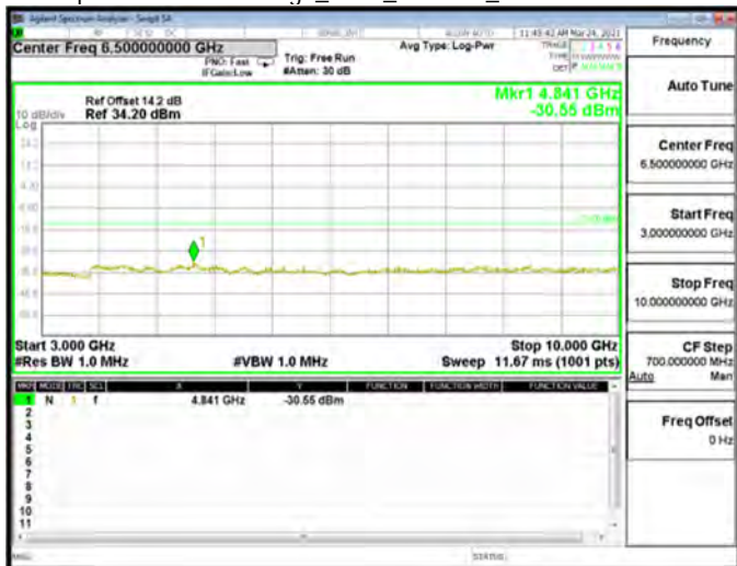
Spurious Emission High_GSM_850MHz_High CH251-848.8
