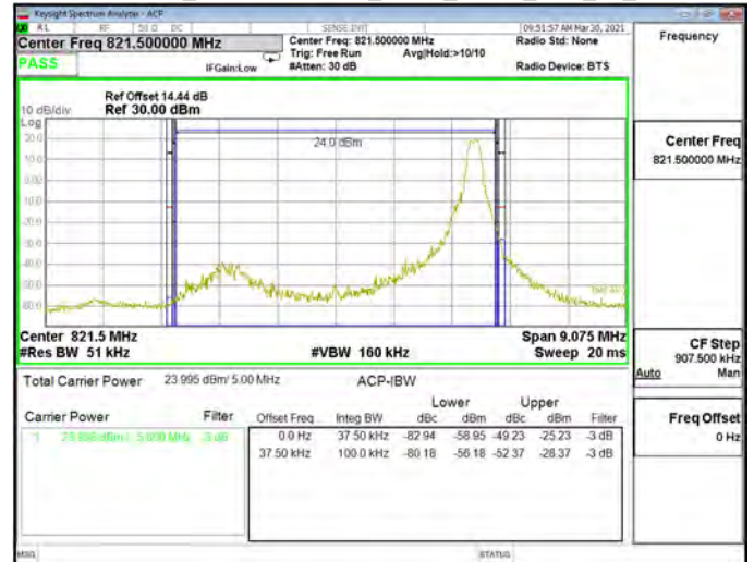
Emission Mask_Band26-Part90s_5MHz_QPSK_RB1_24_CH26765
