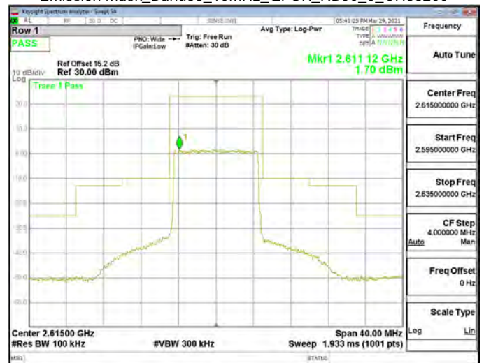
Emission Mask_Band38_10MHz_QPSK_RB50_0_CH38200
