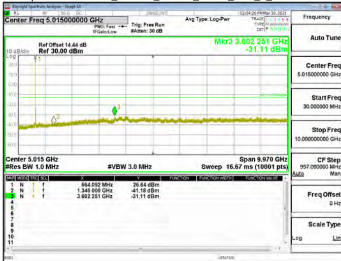
Spurious Emission_Band71_20MHz_QPSK_RB1_0_CH133297
