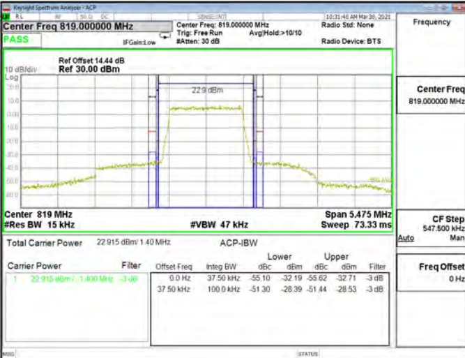
Emission Mask_Band26-Part90s_1.4MHz_QPSK_RB6_0_CH26783
