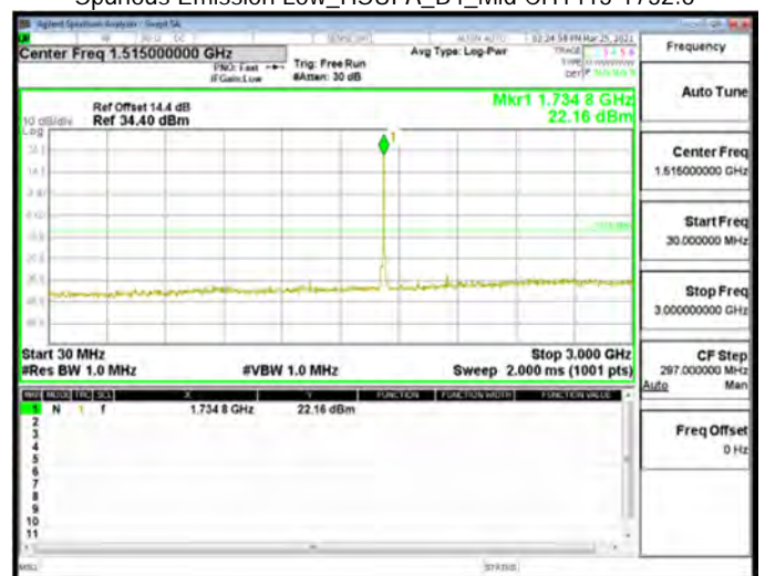
Spurious Emission Low_HSUPA_B4_Mid CH1413-1732.6
