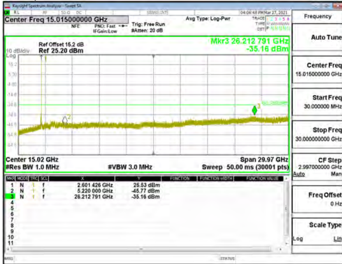
Spurious Emission_Band41_20MHz_QPSK_RB1_0_CH39750
