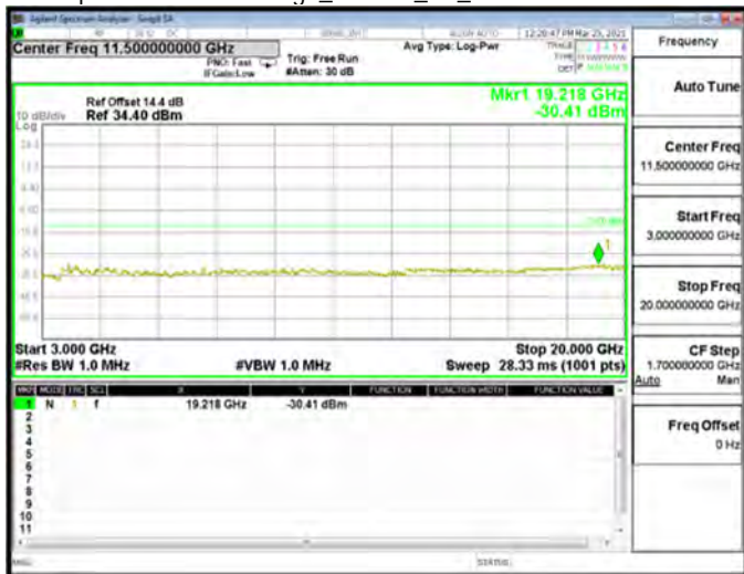
Spurious Emission High_HSUPA_B2_Mid CH9400-1880
