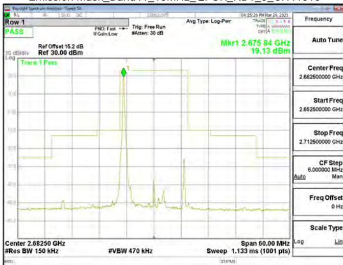
Emission Mask_Band41_15MHz_QPSK_RB1_0_CH41515
