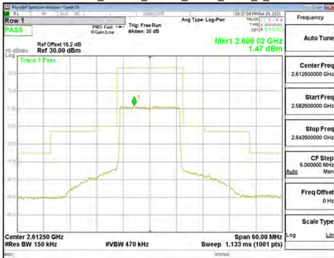
Emission Mask_Band38_15MHz_QPSK_RB75_0_CH38175
