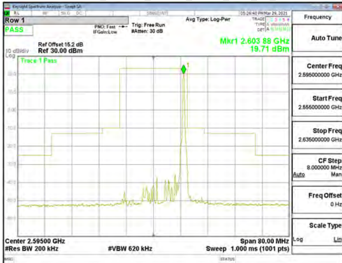
Emission Mask_Band38_20MHz_QPSK_RB1_99_CH38150
