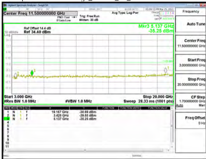
Spurious Emission High_HSDPA_B4_Mid CH1413-1732.6
