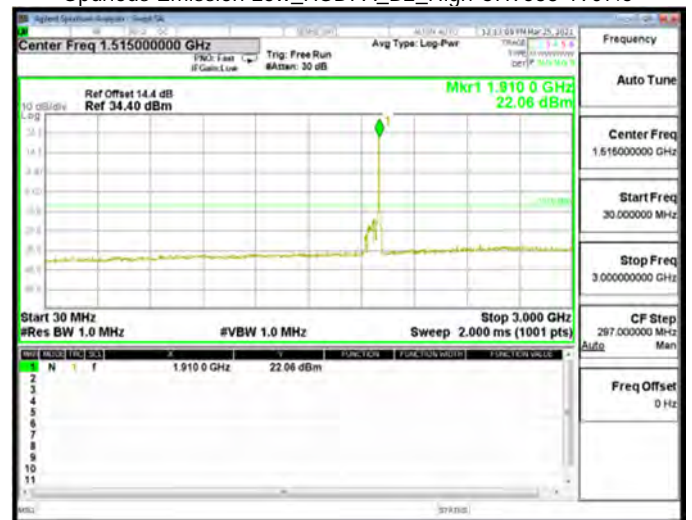
Spurious Emission Low_HSDPA_B2_High CH9538-1907.6
