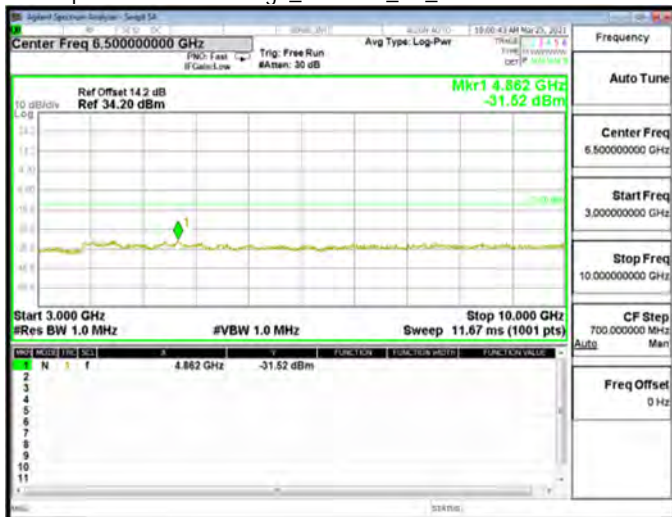
Spurious Emission High_WCDMA_B5_Mid CH4183-836.6
