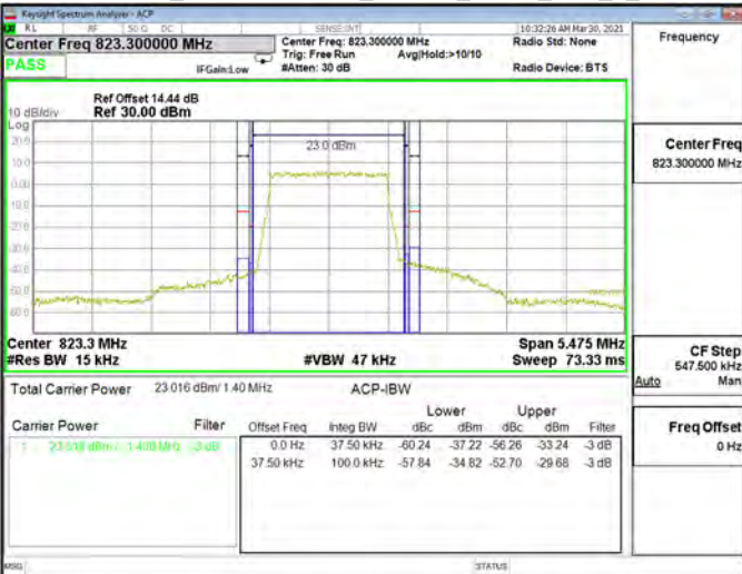
Emission Mask_Band26-Part90s_1.4MHz_QPSK_RB6_0_CH26783
