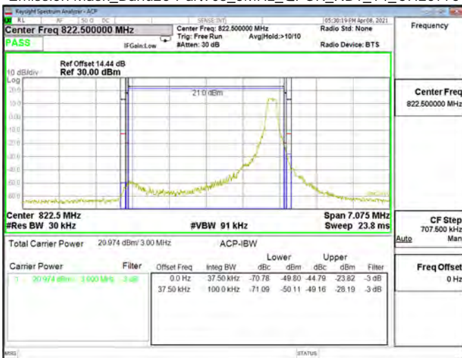
Emission Mask_Band26-Part90s_3MHz_QPSK_RB1_14_CH26775
