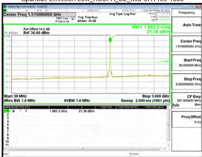
Spurious Emission Low_HSUPA_B2_Mid CH9400-1880
