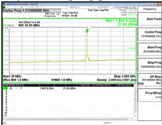
Spurious Emission Low_HSUPA_B2_Mid CH9400-1880
