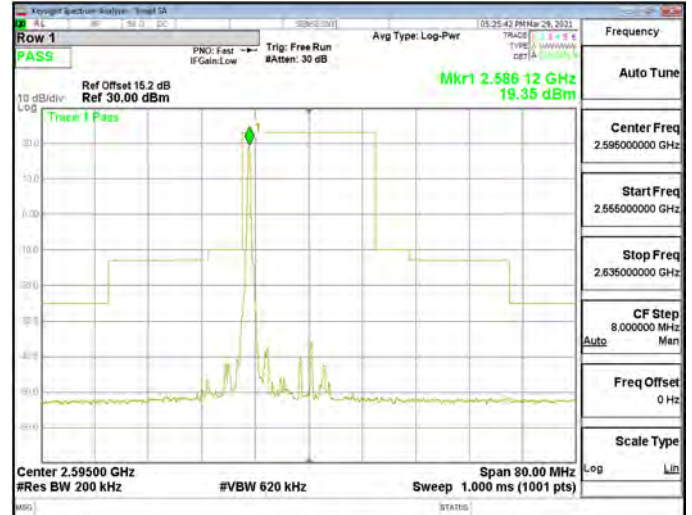
Emission Mask_Band38_20MHz_QPSK_RB1_0_CH38150
