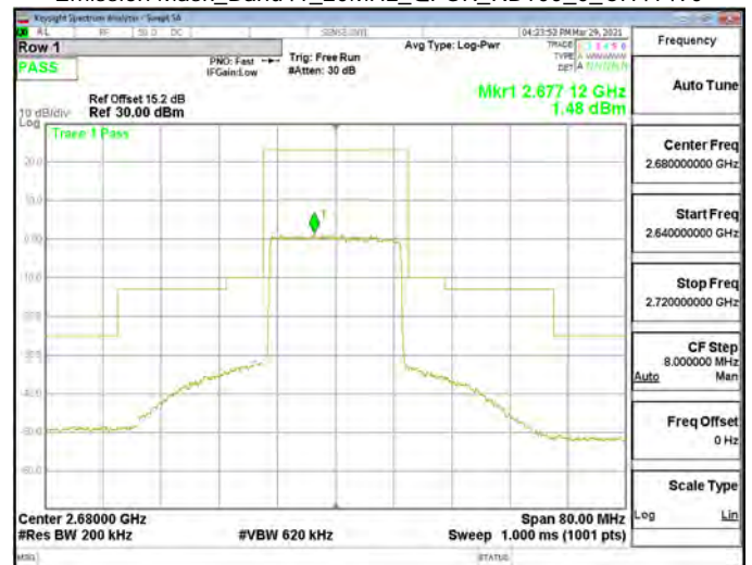
Emission Mask_Band41_20MHz_QPSK_RB100_0_CH41490
