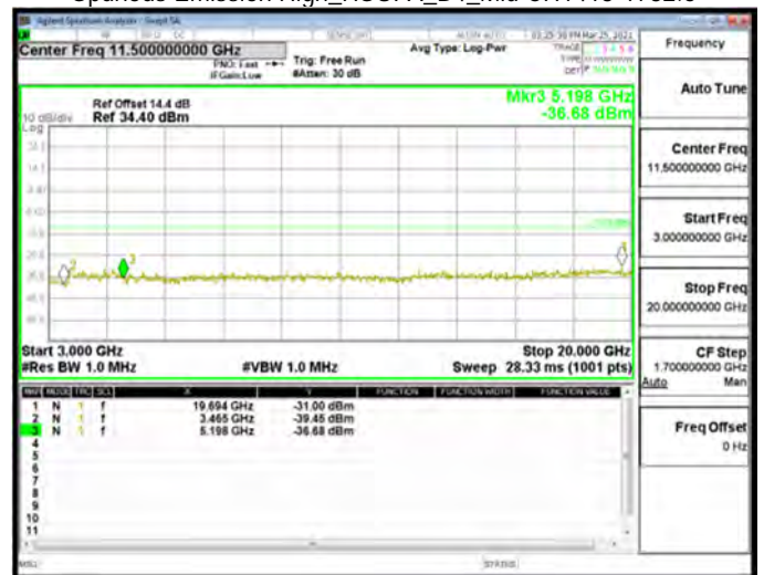
Spurious Emission High_HSUPA_B4_Mid CH1413-1732.6
