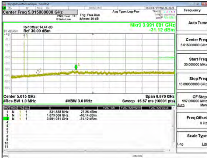
Spurious Emission_Band5_10MHz_QPSK_RB1_0_CH20600
