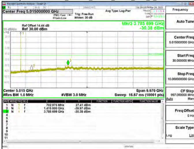
Spurious Emission_Band12_10MHz_QPSK_RB1_0_CH23130
