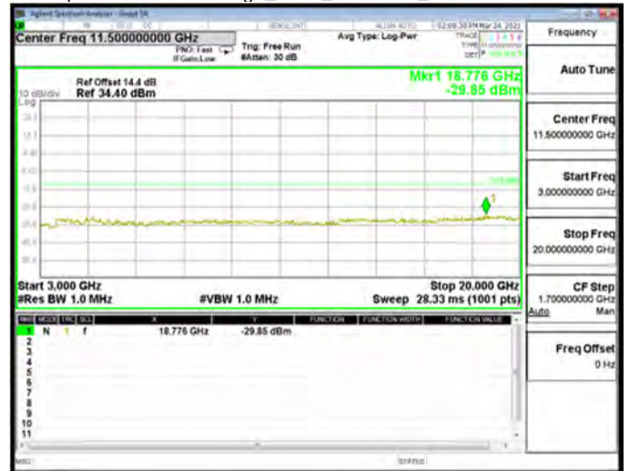
Spurious Emission High_GSM_1900MHz_High CH810-1909.8
