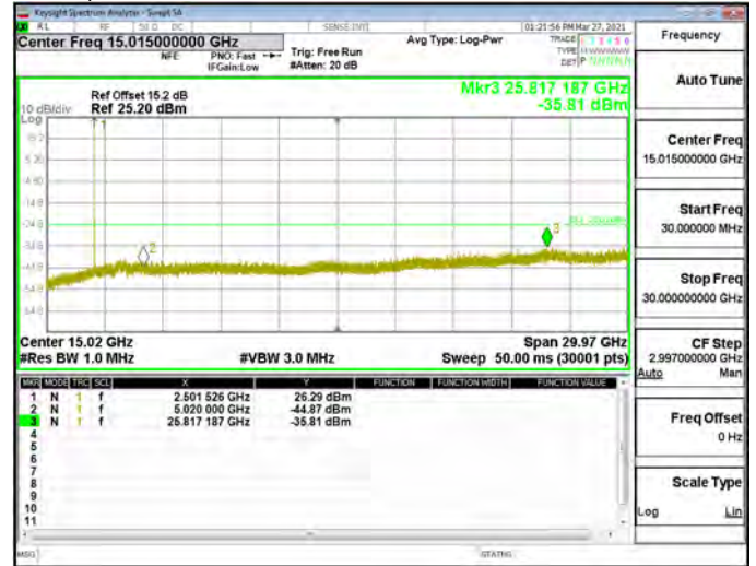
Spurious Emission_Band7_20MHz_QPSK_RB1_0_CH21100
