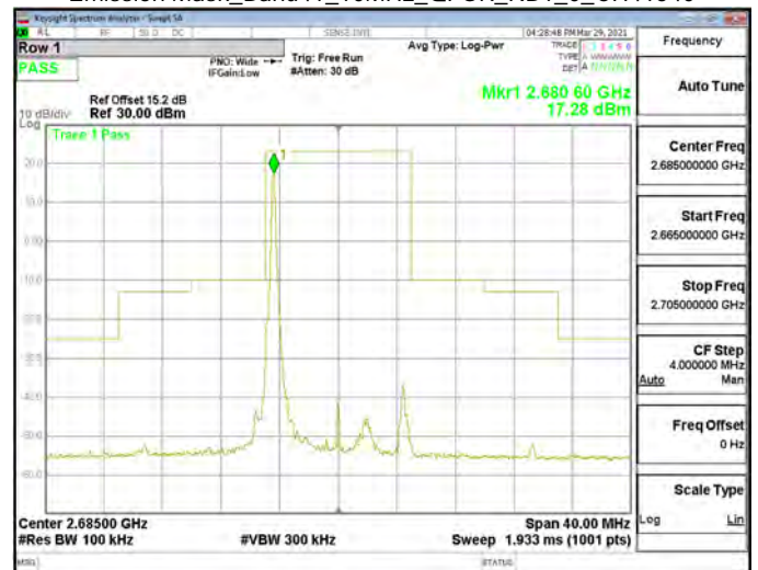
Emission Mask_Band41_10MHz_QPSK_RB1_0_CH41540
