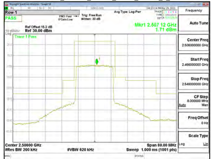
Emission Mask_Band41_20MHz_QPSK_RB100_0_CH40620
