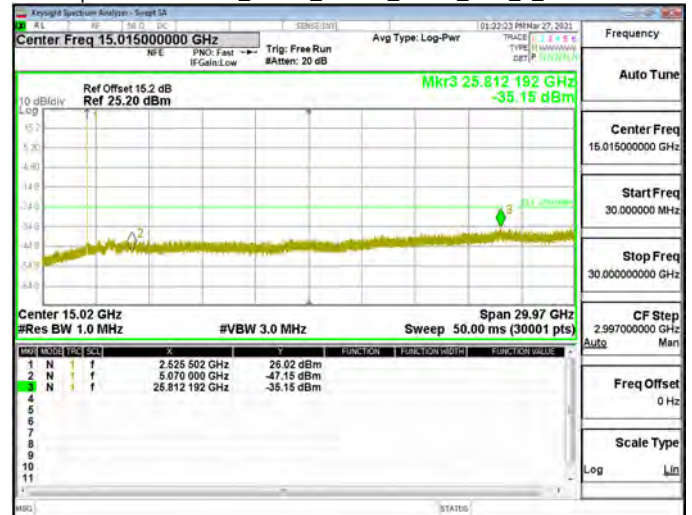
Spurious Emission_Band7_20MHz_QPSK_RB1_0_CH21350
