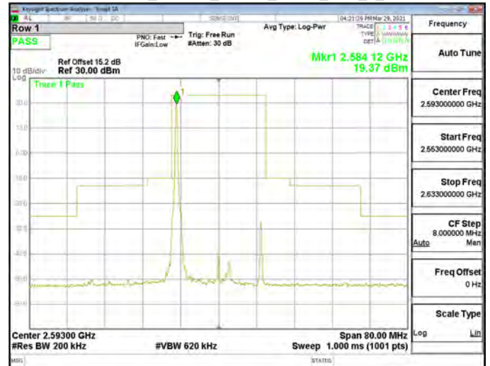
Emission Mask_Band41_20MHz_QPSK_RB1_0_CH41490
