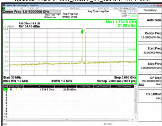
Spurious Emission Low_HSDPA_B4_Mid CH1413-1732.6
