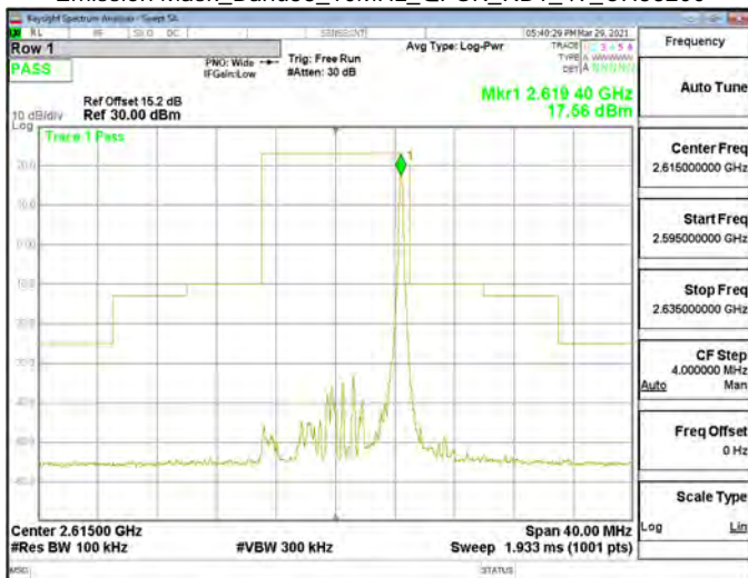
Emission Mask_Band38_10MHz_QPSK_RB1_49_CH38200
