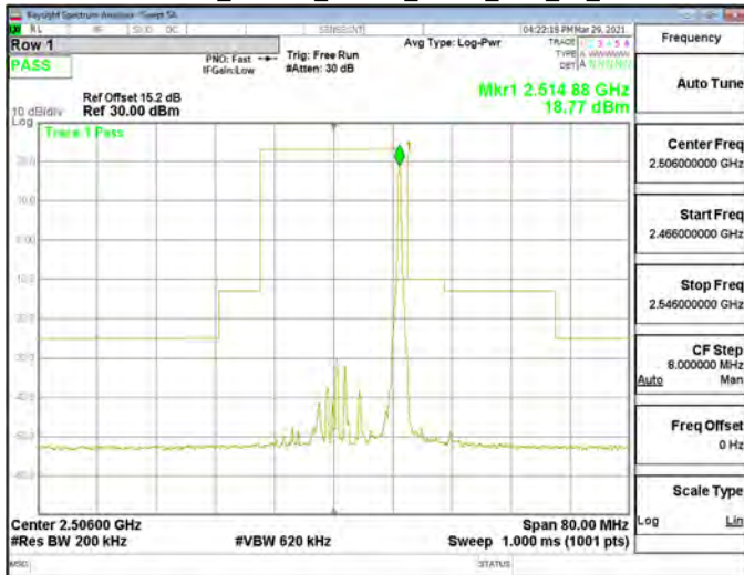
Emission Mask_Band41_20MHz_QPSK_RB1_99_CH40620
