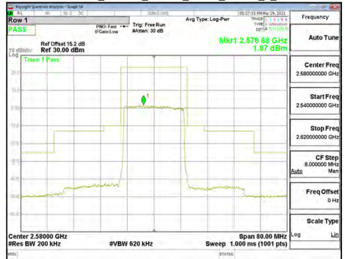
Emission Mask_Band38_20MHz_QPSK_RB100_0_CH38000
