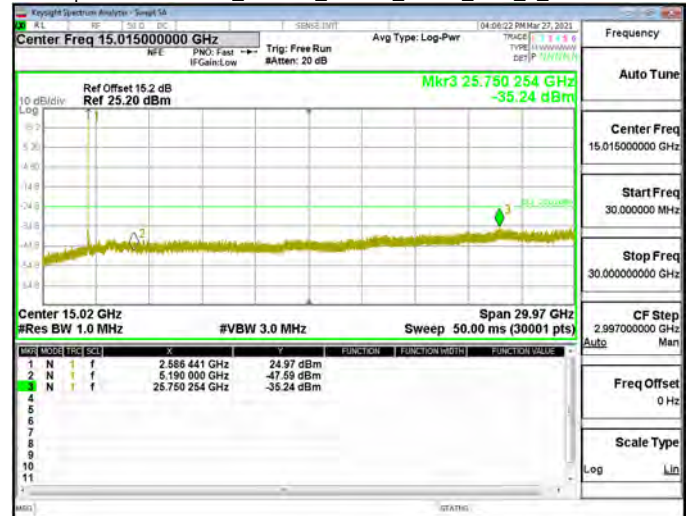
Spurious Emission_Band38_20MHz_QPSK_RB1_0_CH38000
