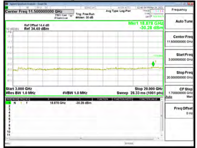
Spurious Emission High_EDGE_1900MHz_Mid CH661-1880
