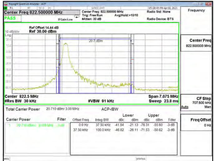
Emission Mask_Band26-Part90s_3MHz_QPSK_RB1_0_CH26775
