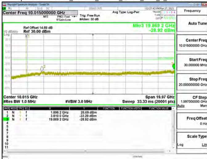
Spurious Emission_Band25_20MHz_QPSK_RB1_0_CH26590
