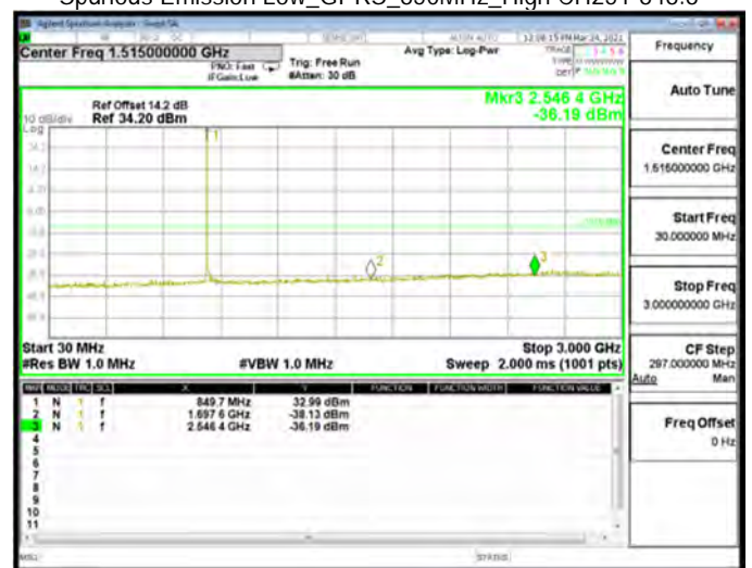
Spurious Emission Low_GPRS_850MHz_High CH251-848.8
