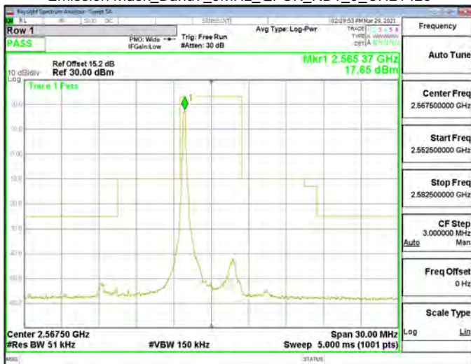
Emission Mask_Band7_5MHz_QPSK_RB1_0_CH21425
