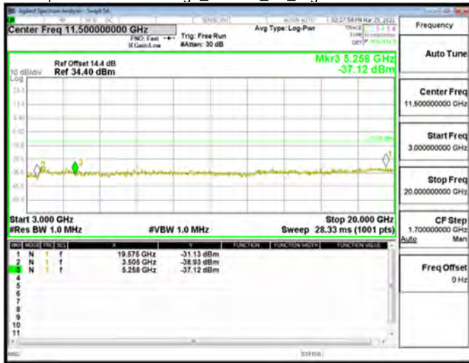
Spurious Emission High_WCDMA_B5_Low CH4132-826.4
