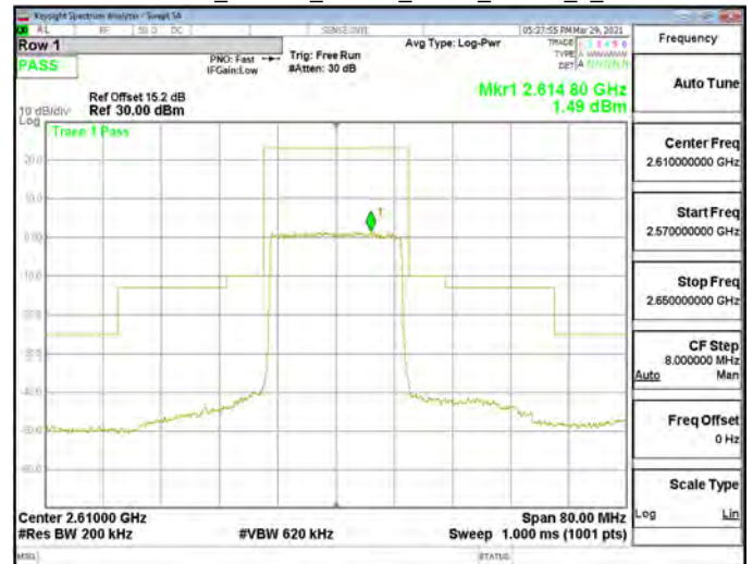
Emission Mask_Band38_20MHz_QPSK_RB100_0_CH38150
