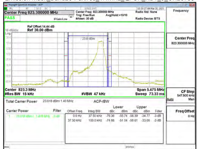
Emission Mask_Band26-Part90s_1.4MHz_QPSK_RB1_5_CH26783
