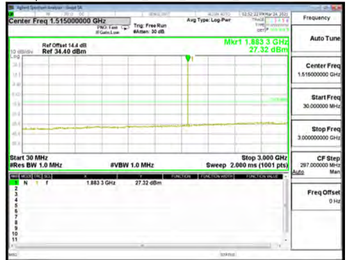
Spurious Emission Low_EDGE_1900MHz_High CH810-1909.8
