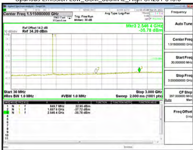
Spurious Emission Low_GSM_850MHz_High CH251-848.8
