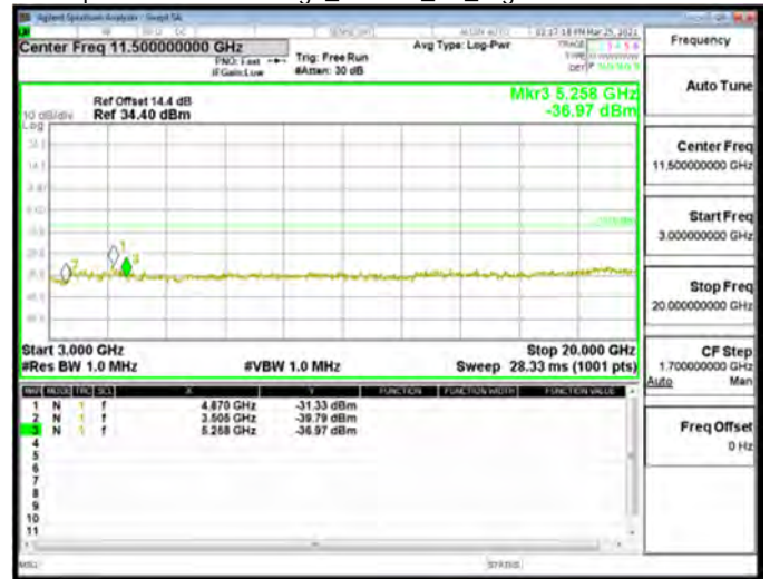
Spurious Emission High_HSUPA_B4_Low CH1312-1712.4
