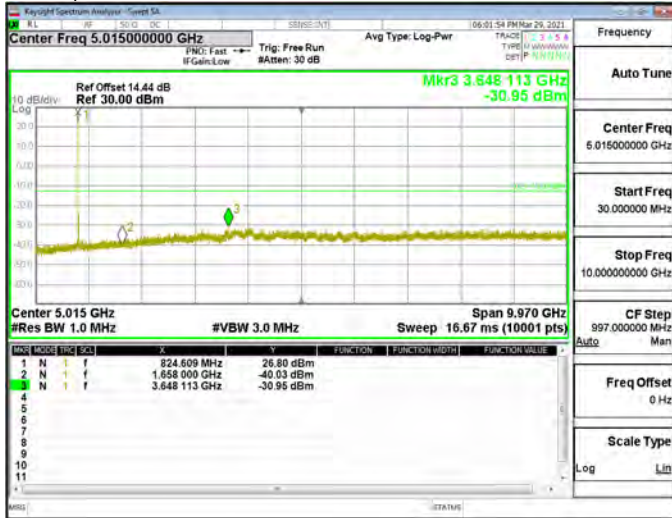
Spurious Emission_Band5_10MHz_QPSK_RB1_0_CH20525
