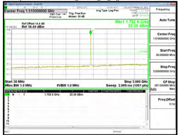
Spurious Emission Low_HSUPA_B4_Low CH1312-1712.4
