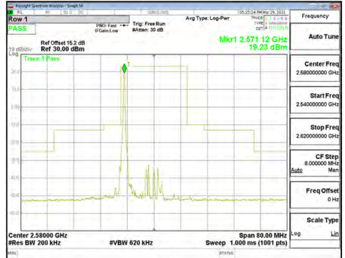
Emission Mask_Band38_20MHz_QPSK_RB1_0_CH38000
