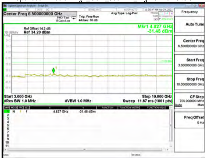
Spurious Emission High_GSM_850MHz_High CH251-848.8
