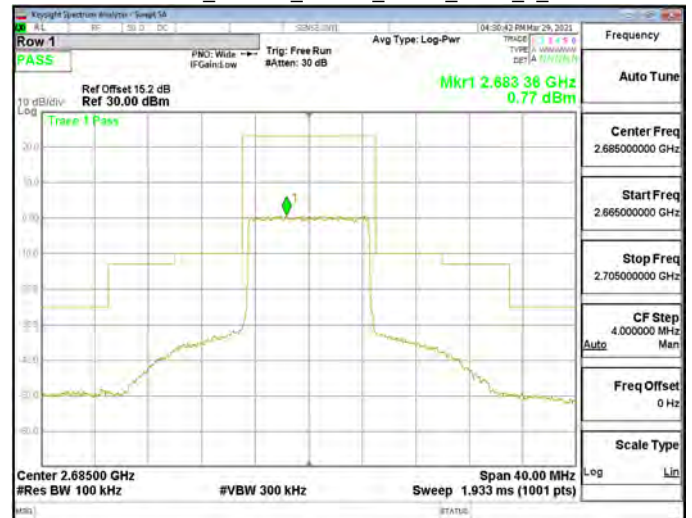
Emission Mask_Band41_10MHz_QPSK_RB50_0_CH41540
