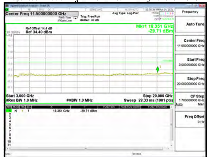
Spurious Emission High_EDGE_1900MHz_High CH810-1909.8
