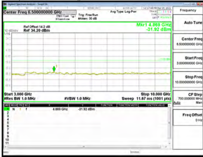
Spurious Emission High_EDGE_850MHz_Mid CH190-836.6
