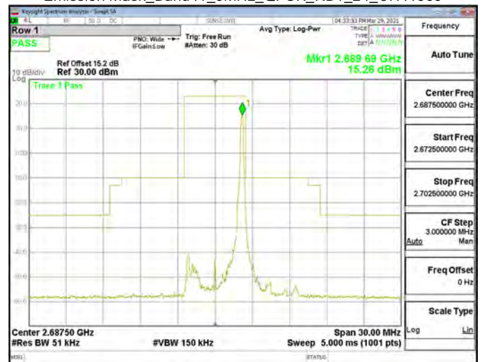
Emission Mask_Band41_5MHz_QPSK_RB1_24_CH41565
