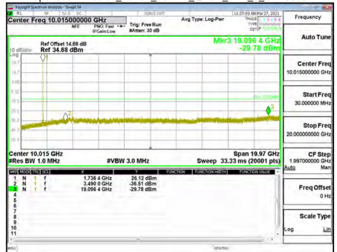
Spurious Emission_Band4_20MHz_QPSK_RB1_0_CH20300
