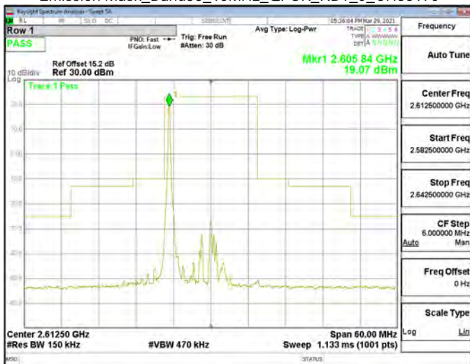
Emission Mask_Band38_15MHz_QPSK_RB1_0_CH38175
