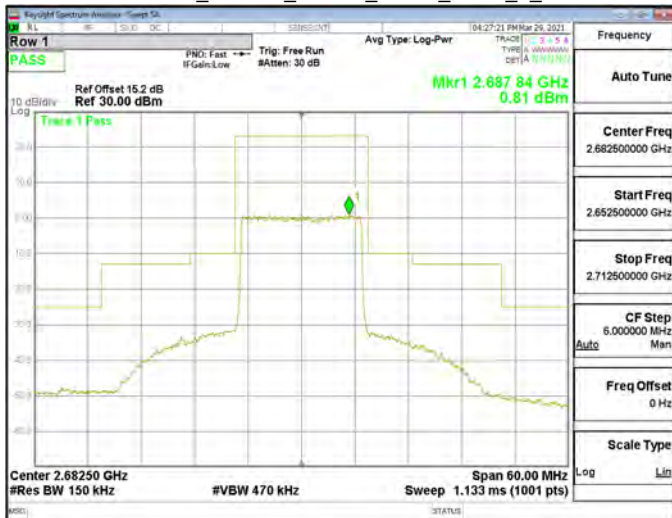
Emission Mask_Band41_15MHz_QPSK_RB75_0_CH41515
