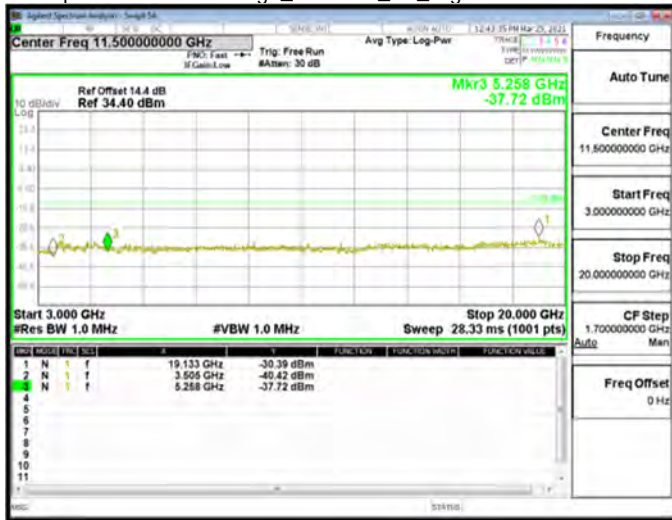
Spurious Emission High_HSDPA_B4_Low CH1312-1712.4
