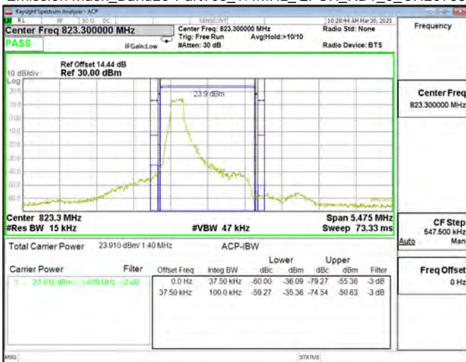
Emission Mask_Band26-Part90s_1.4MHz_QPSK_RB1_0_CH26783
