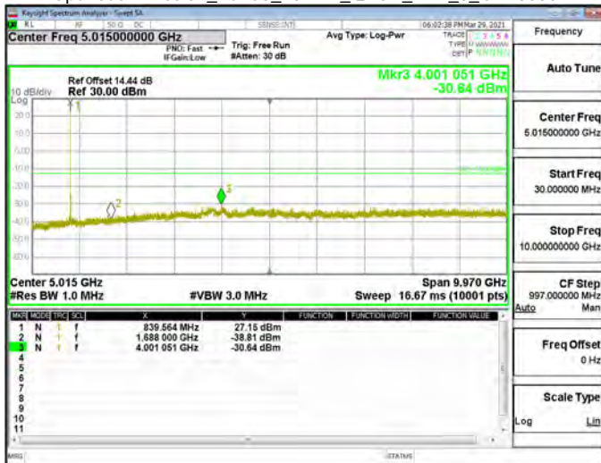
Spurious Emission_Band5_10MHz_QPSK_RB1_0_CH20600
