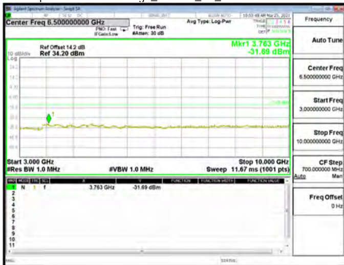
Spurious Emission High_HSUPA_B5_Mid CH4183-836.6
