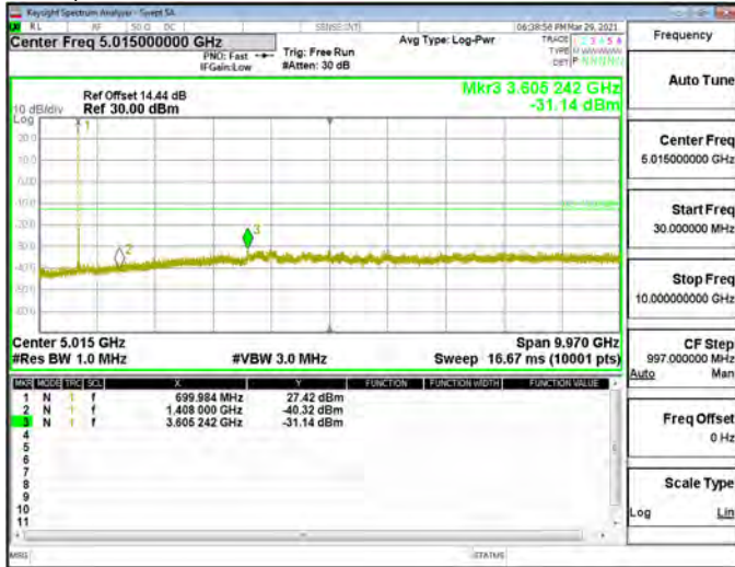
Spurious Emission_Band12_10MHz_QPSK_RB1_0_CH23095
