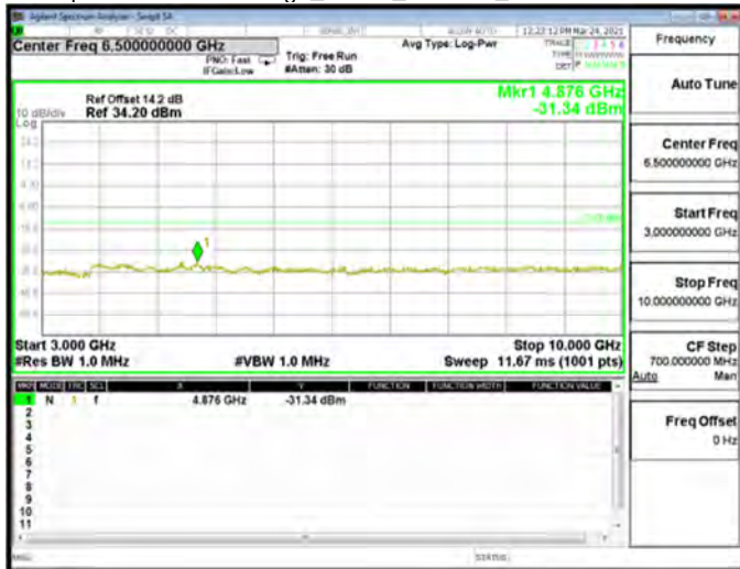
Spurious Emission High_EDGE_850MHz_High CH251-848.8
