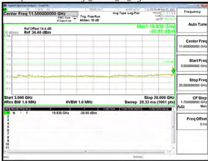
Spurious Emission High_HSUPA_B2_Low CH9262-1852.4
