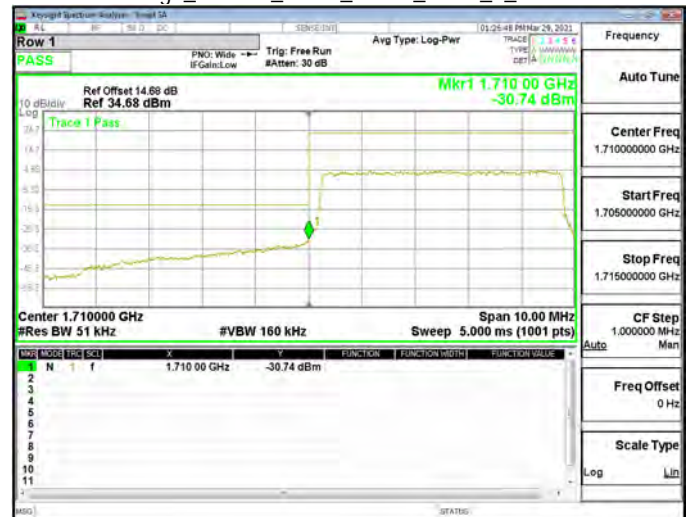
Band Edge_Band66_5MHz_QPSK_RB25_0_CH132647
