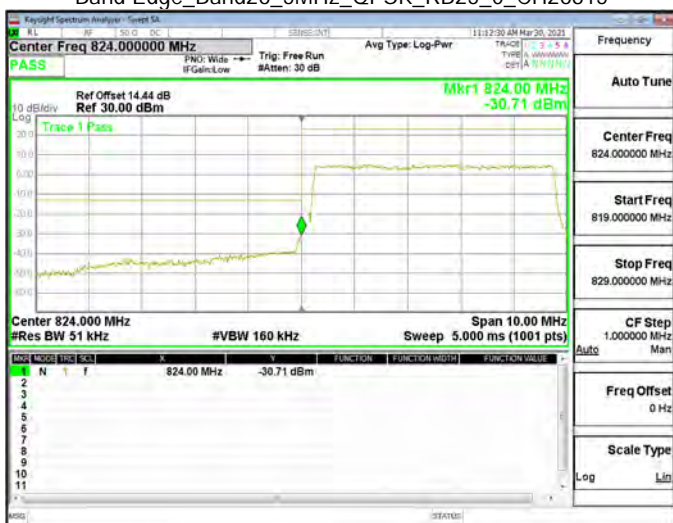
Band Edge_Band26_5MHz_QPSK_RB25_0_CH26815
