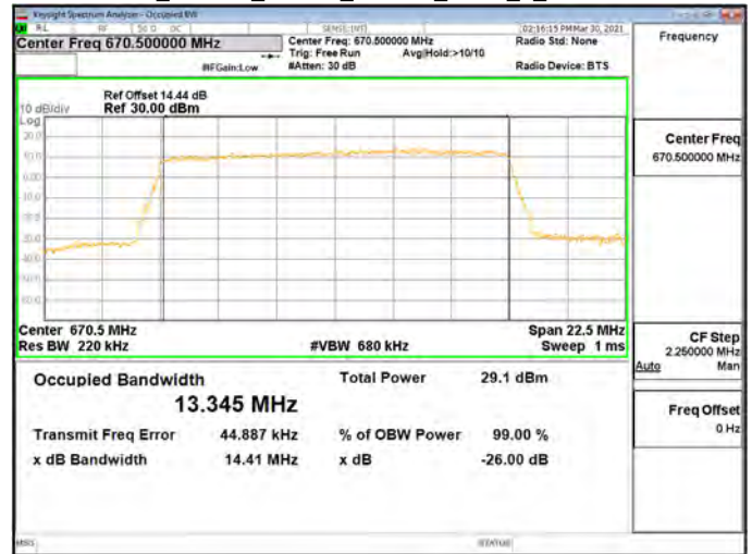
OBW_Band71_15MHz_64QAM_RB75_0_CH133297
