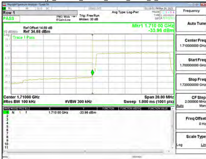
Band Edge_Band66_10MHz_QPSK_RB50_0_CH132022
