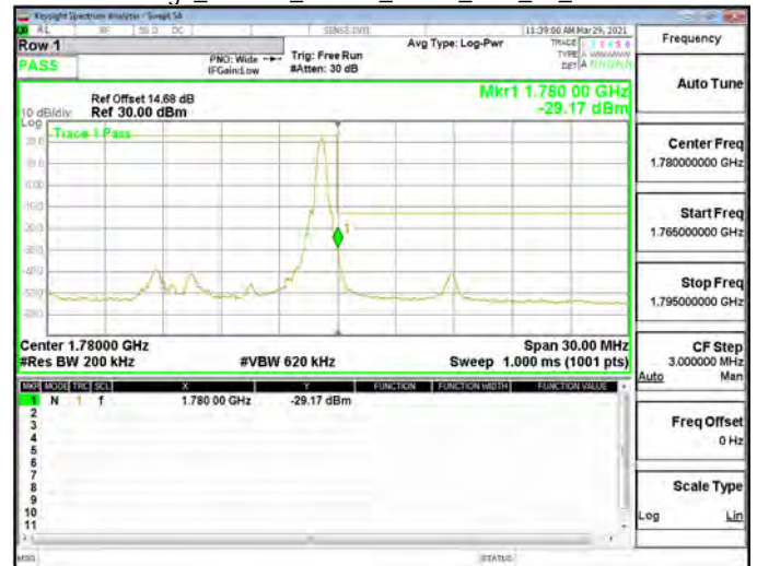
Band Edge_Band66_15MHz_QPSK_RB1_74_CH132597
