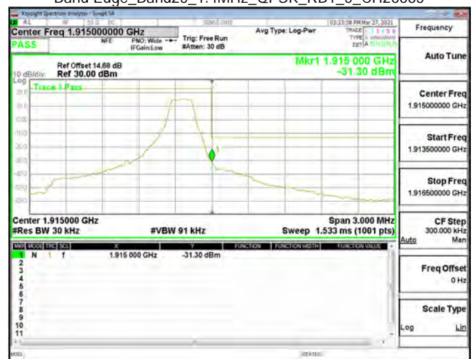
Band Edge_Band25_1.4MHz_QPSK_RB1_5_CH26683
