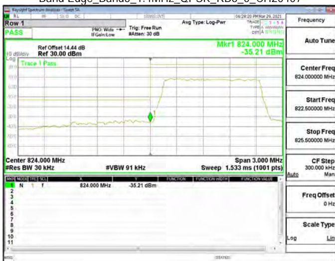
Band Edge_Band5_1.4MHz_QPSK_RB6_0_CH20407
