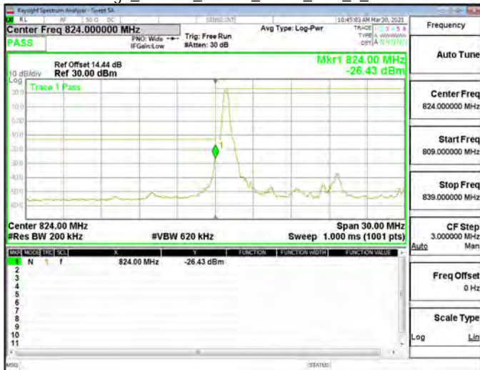
Band Edge_Band26_15MHz_QPSK_RB1_0_CH26865
