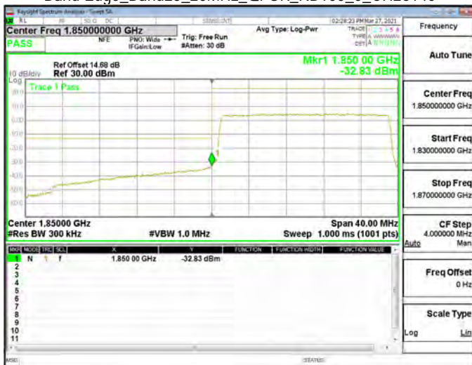
Band Edge_Band25_20MHz_QPSK_RB100_0_CH26140
