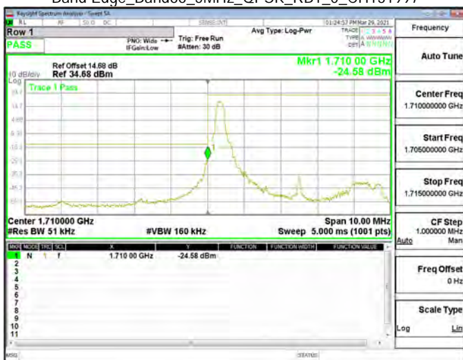
Band Edge_Band66_5MHz_QPSK_RB1_0_CH131997
