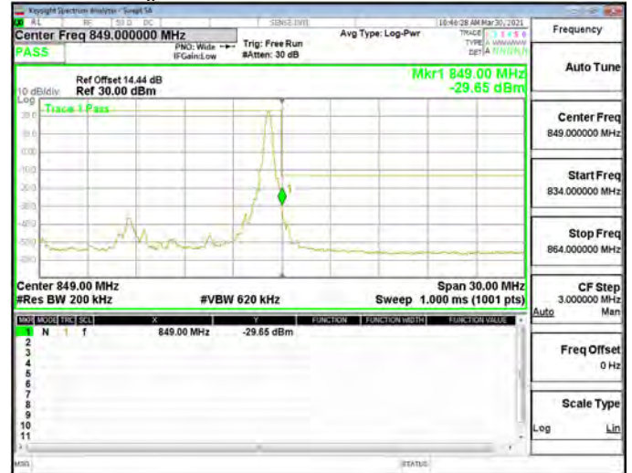
Band Edge_Band26_15MHz_QPSK_RB75_0_CH26865
