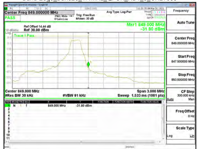
Band Edge_Band26_1.4MHz_QPSK_RB1_5_CH27033
