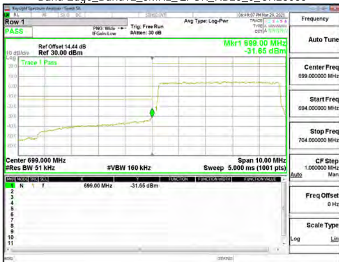
Band Edge_Band12_5MHz_QPSK_RB25_0_CH23035
