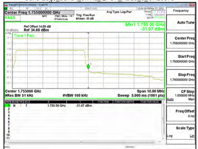
Band Edge_Band4_5MHz_QPSK_RB25_0_CH20375
