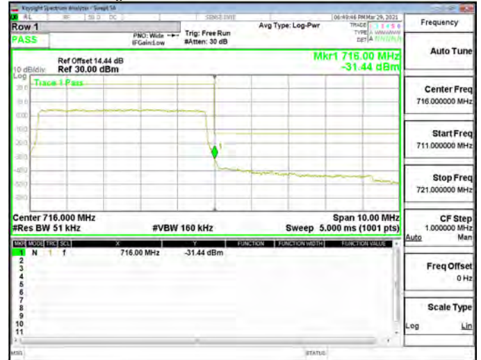
Band Edge_Band12_10MHz_QPSK_RB1_0_CH23060
