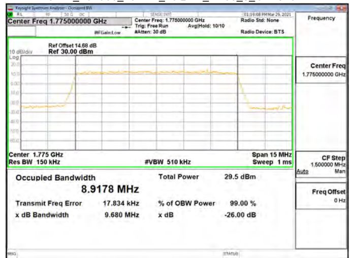
OBW_Band66_10MHz_16QAM_RB50_0_CH132622
