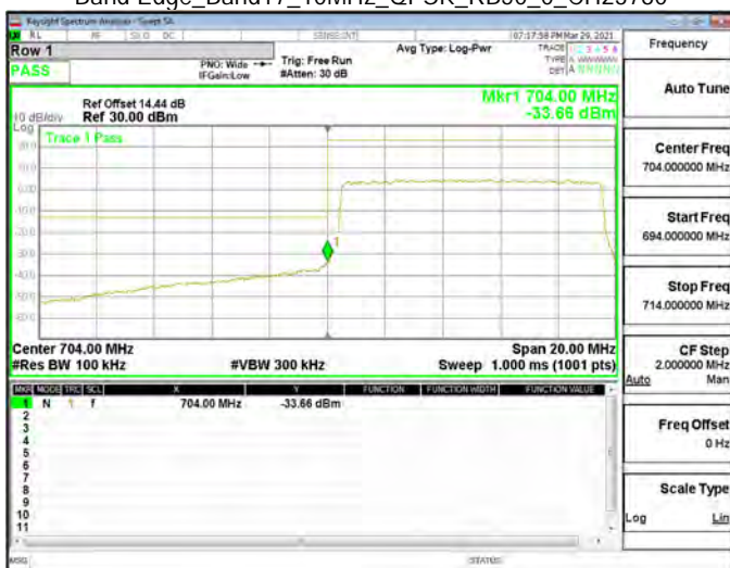
Band Edge_Band17_10MHz_QPSK_RB50_0_CH23780
