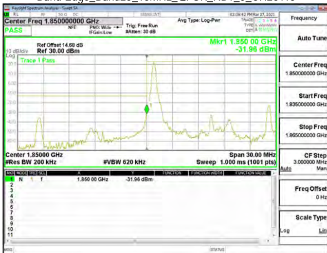
Band Edge_Band25_15MHz_QPSK_RB1_0_CH26115
