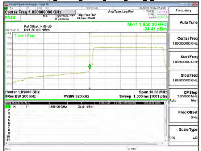
Band Edge_Band25_15MHz_QPSK_RB75_0_CH26615
