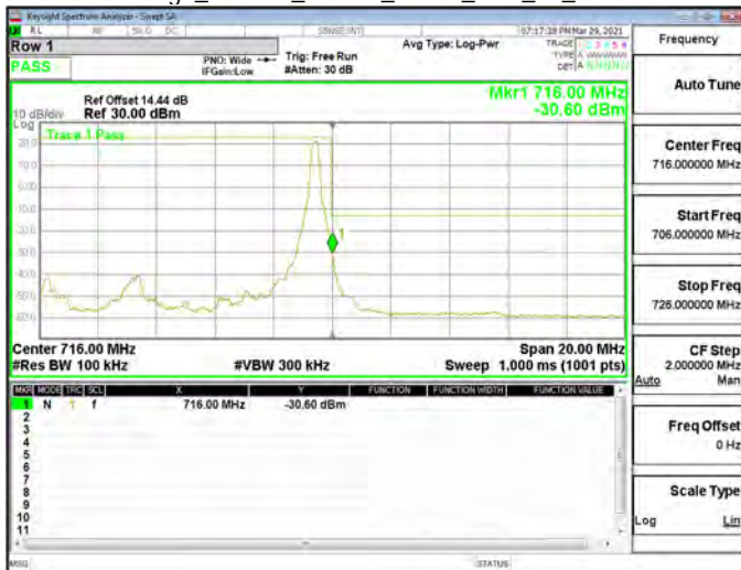
Band Edge_Band17_10MHz_QPSK_RB50_0_CH23780
