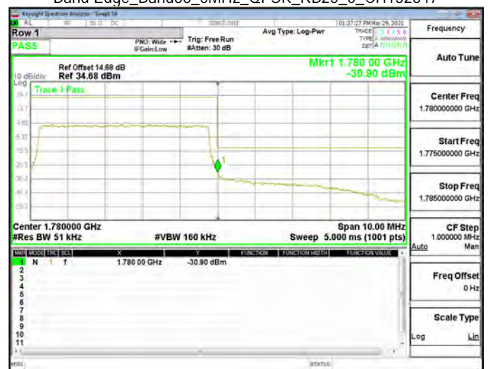
Band Edge_Band66_5MHz_QPSK_RB25_0_CH132647
