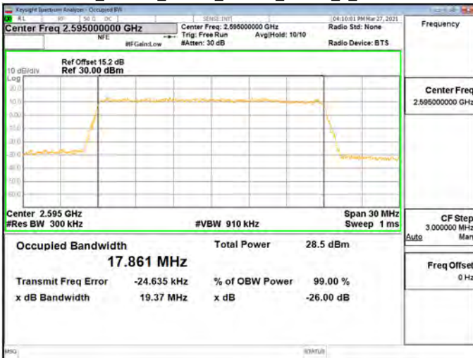
OBW_Band38_20MHz_64QAM_RB100_0_CH38150
