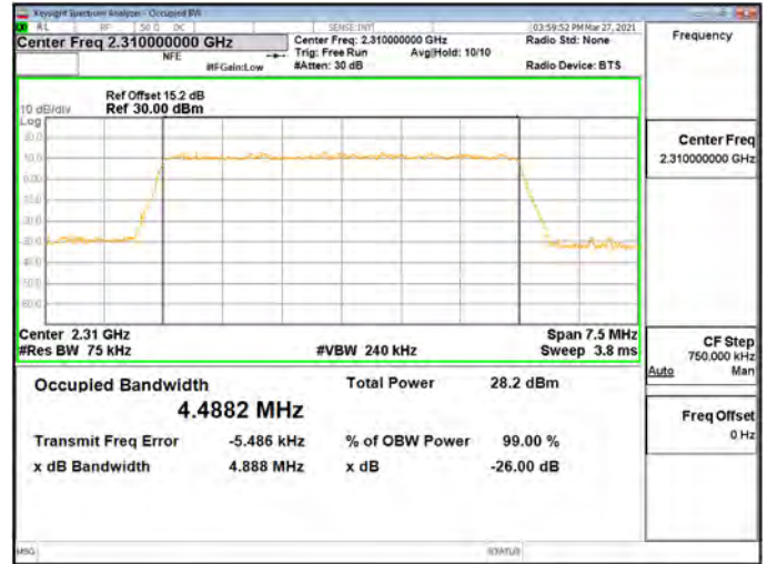
OBW_Band30_5MHz_64QAM_RB25_0_CH27735
