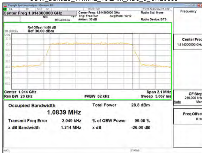
OBW Band25 1.4MHz 16QAM RB6 0 CH26683
