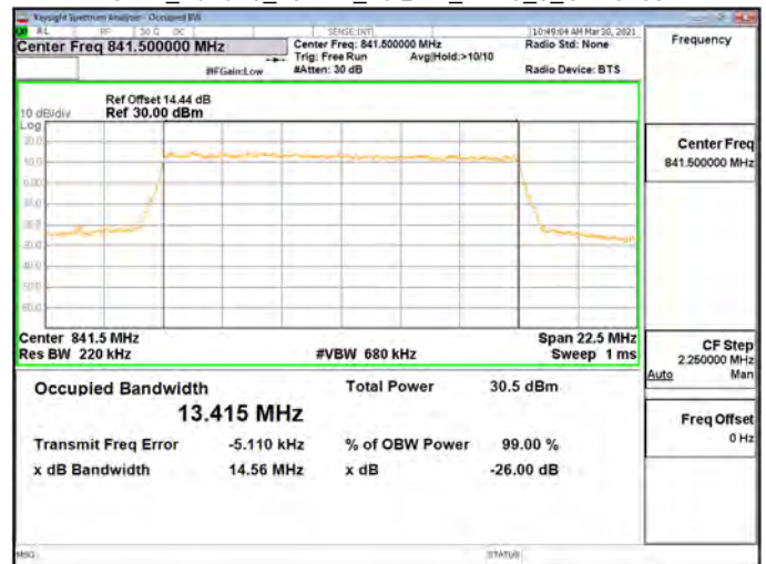
OBW_Band26_15MHz_16QAM_RB75_0_CH26965
