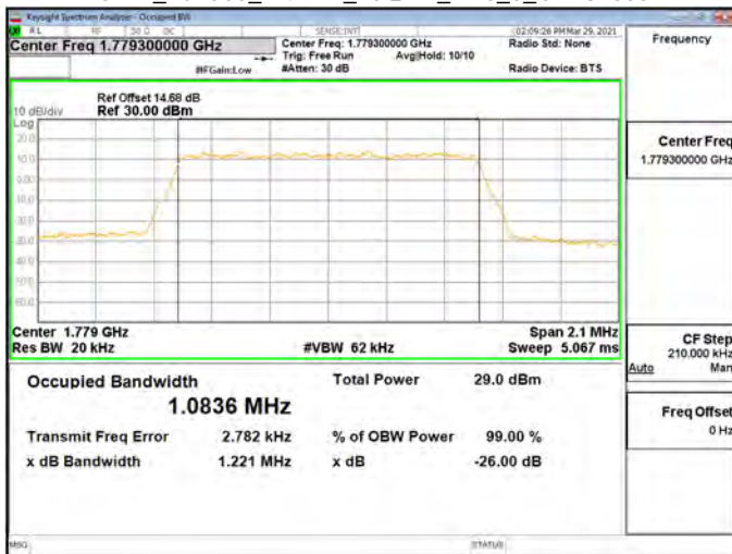
OBW_Band66_1.4MHz_16QAM_RB6_0_CH132665
