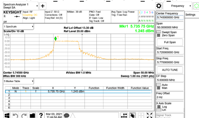
802.11ax_20MHz_Chain0_5745MHz_RU106_53
