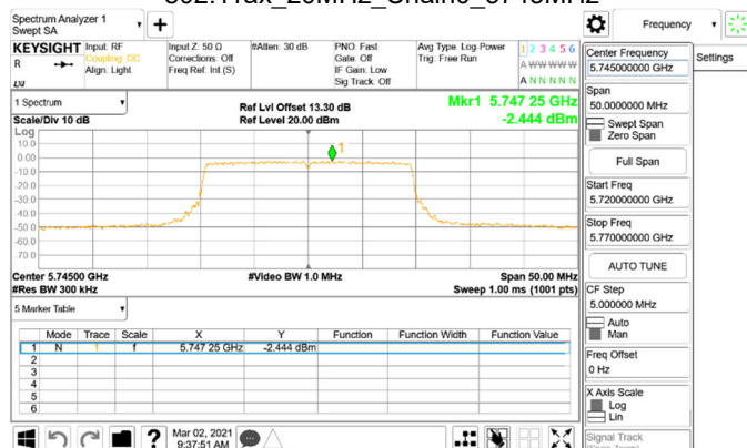
802.11ax_20MHz_Chain0_5745MHz_RU106_53
