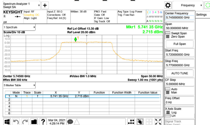
802.11a_20MHz_Chain0_5745MHz
