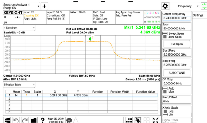
802.11a_20MHz_Chain0_5240MHz
