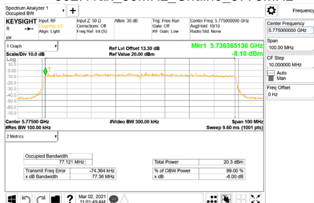
802.11ax_80MHz_Chain0_5775MHz
