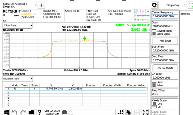
802.11ax_20MHz_Chain1_5745MHz_RU106_53
