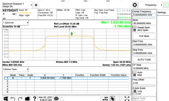
802.11ax_20MHz_Chain0_5825MHz_RU106_54
