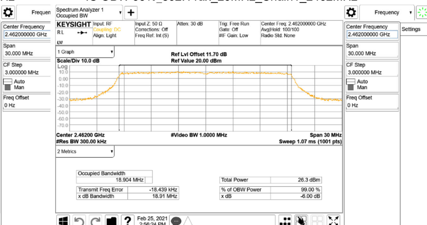
IC OBW 99%_802.11ax_20MHz_Chain1_2462MHz
