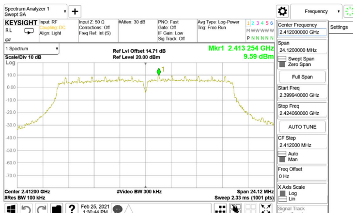
Reference Level _802.11g_20MHz_Chain0_2412MHz
