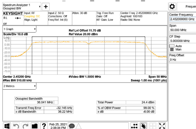
IC OBW 99%_802.11n_40MHz_Chain0_2452MHz
