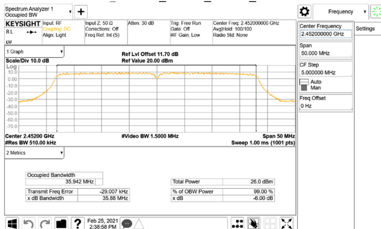
IC OBW 99%_802.11n_40MHz_Chain1_2452MHz
