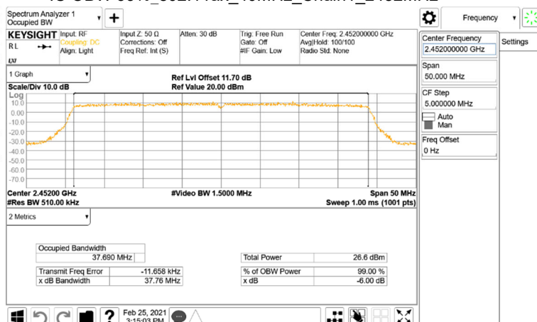
IC OBW 99%_802.11ax_40MHz_Chain1_2452MHz
