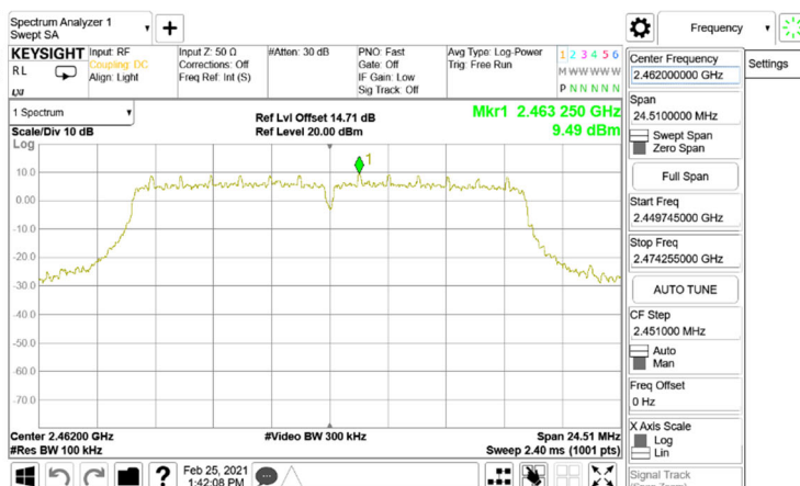
Reference Level _802.11g_20MHz_Chain0_2462MHz
