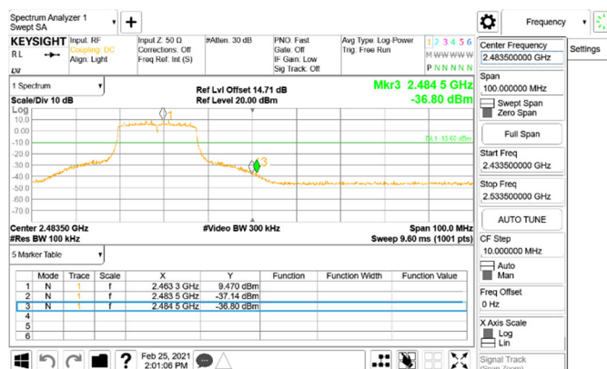
Band Edge_802.11n_20MHz_Chain0_2462MHz
