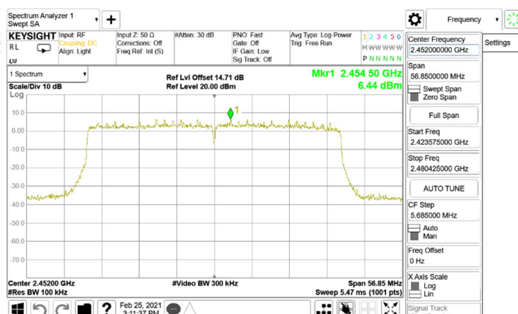
Reference Level _802.11ax_40MHz_Chain0_2452MHz
