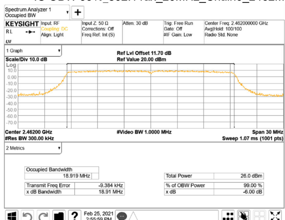
IC OBW 99%_802.11ax_20MHz_Chain0_2462MHz
