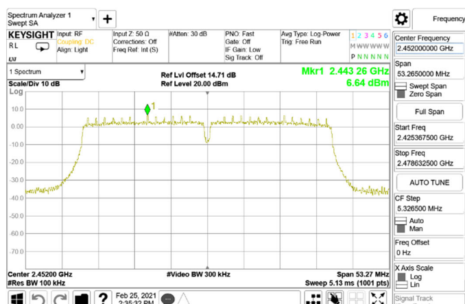
Reference Level _802.11n_40MHz_Chain0_2452MHz
