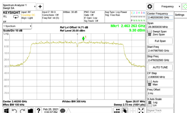
Reference Level _802.11ax_20MHz_Chain0_2462MHz
