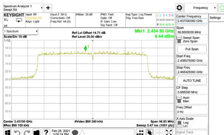
Reference Level _802.11ax_40MHz_Chain0_2437MHz
