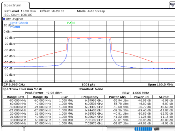
Plot on Channel 6965MHz
