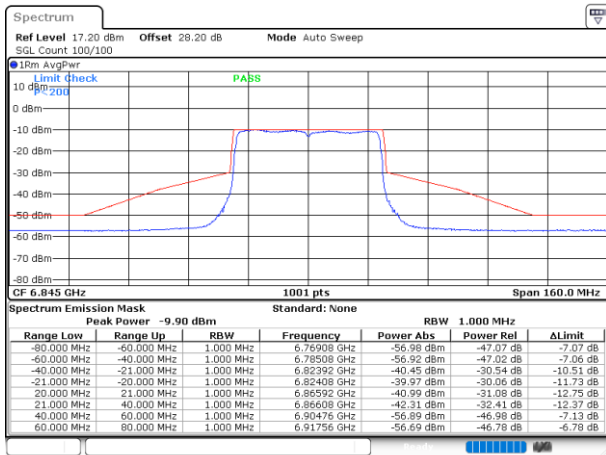
Plot on Channel 6845MHz
