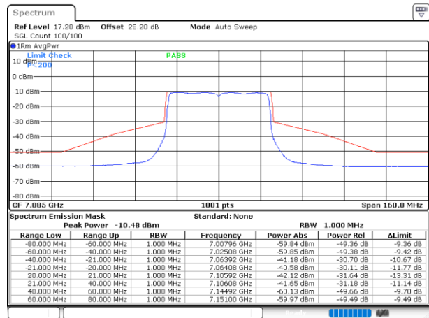
Plot on Channel 7085MHz
