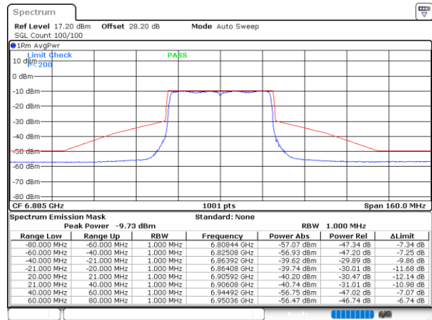
Plot on Channel 6885MHz
