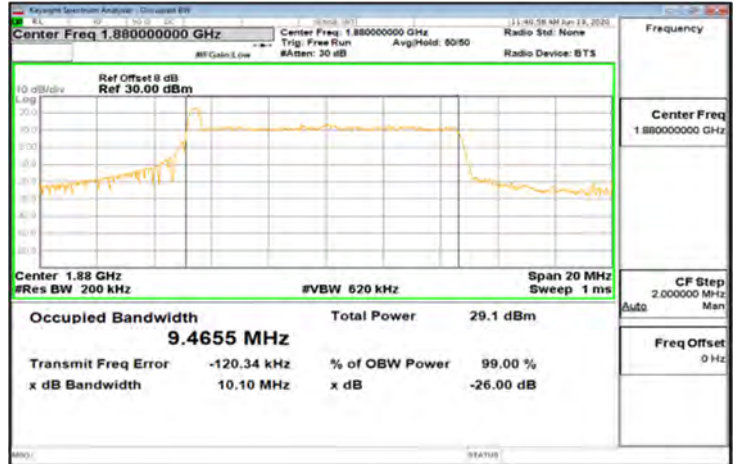
CP-OFDM_Band2_10MHz_QPSK_52_0_Main_MidCH376000-1880
