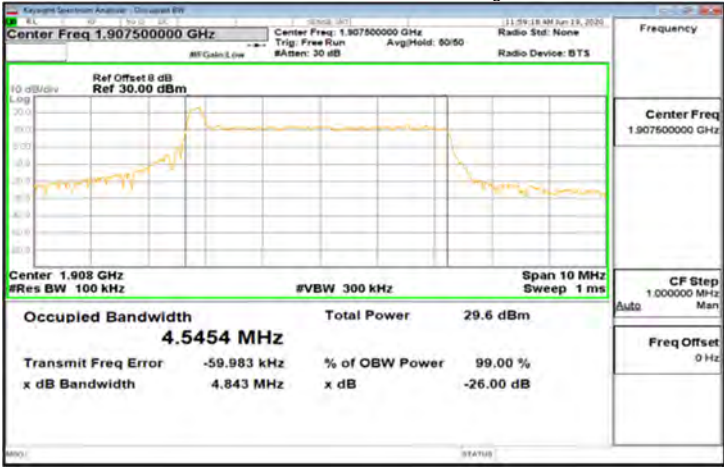
CP-OFDM_Band2_5MHz_16QAM_25_0_Main_HighCH381500-1907.5
