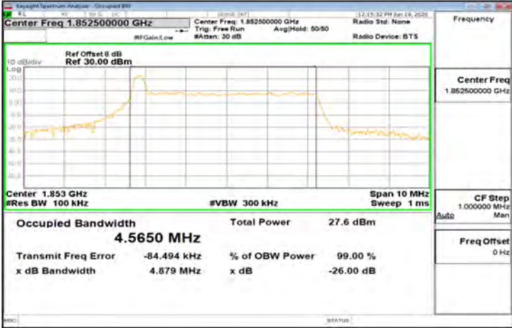
CP-OFDM_Band2_5MHz_256QAM_25_0_Main_LowCH370500-1852.5
