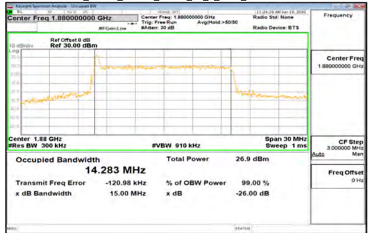
CP-OFDM_Band2_15MHz_QPSK_79_0_Main_MidCH376000-1880
