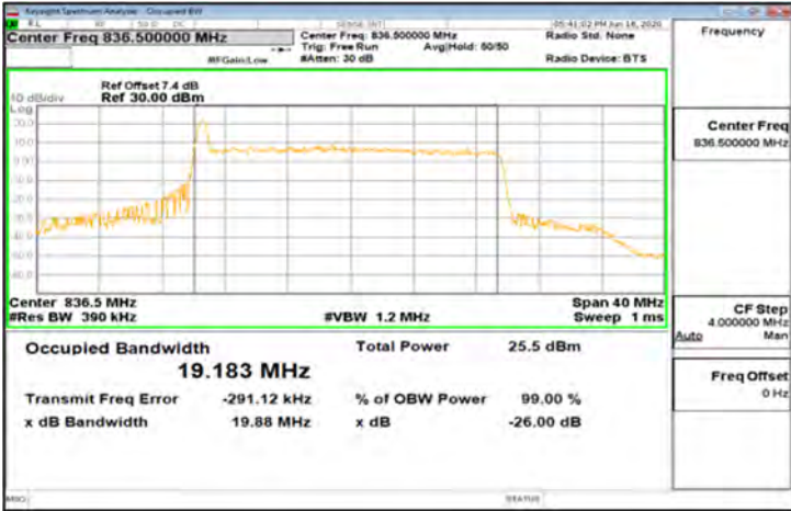
CP-OFDM_Band5_20MHz_256QAM_106_0_Main_MidCH167300-836.5
