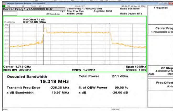
CP-OFDM_Band66_20MHz_64QAM_106_0_Main_MidCH349000-1745
