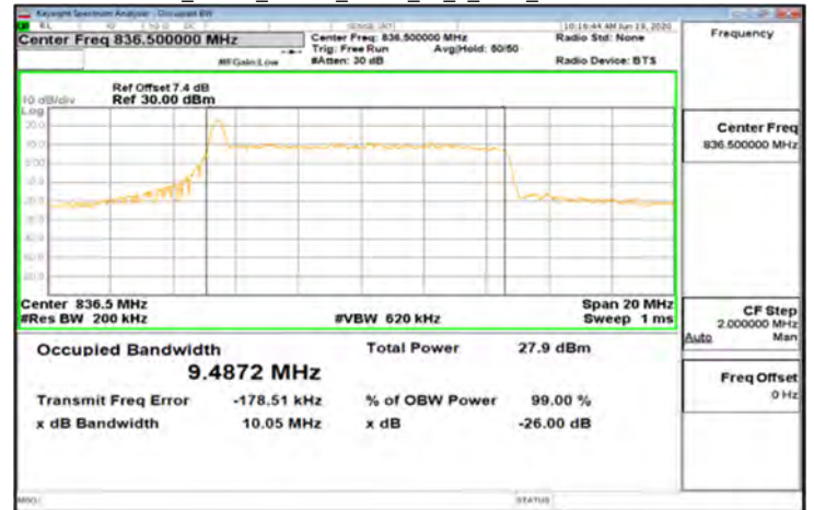
CP-OFDM_Band5_10MHz_QPSK_52_0_Main_MidCH167300-836.5
