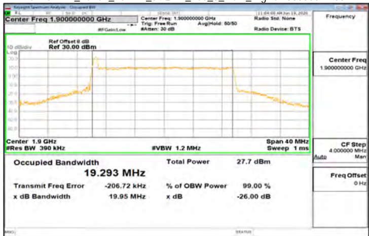
CP-OFDM_Band2_20MHz_64QAM_106_0_Main_HighCH38000-1900
