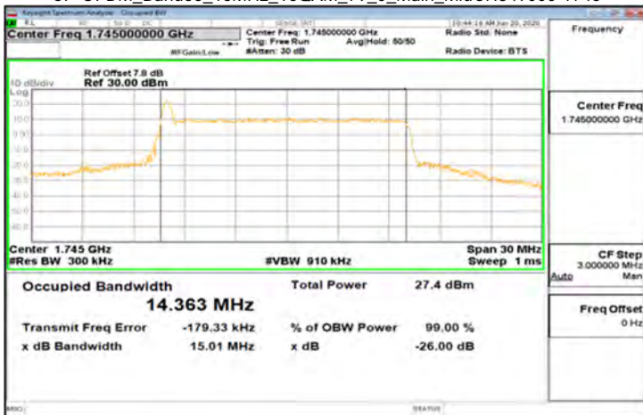
CP-OFDM_Band66_15MHz_16QAM_79_0_Main_MidCH349000-1745
