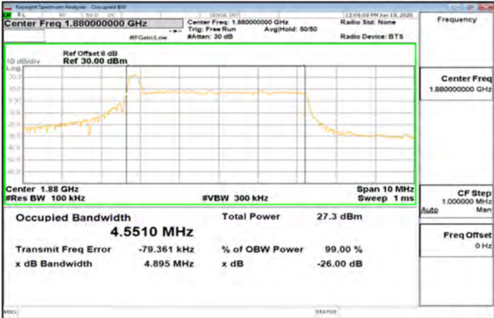
CP-OFDM_Band2_5MHz_256QAM_25_0_Main_MidCH376000-1880
