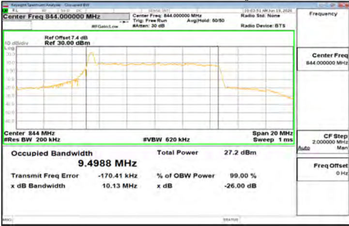
CP-OFDM_Band5_10MHz_16QAM_52_0_Main_LowCH168800-829
