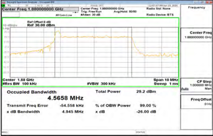
CP-OFDM_Band2_5MHz_64QAM_25_0_Main_MidCH376000-1880
