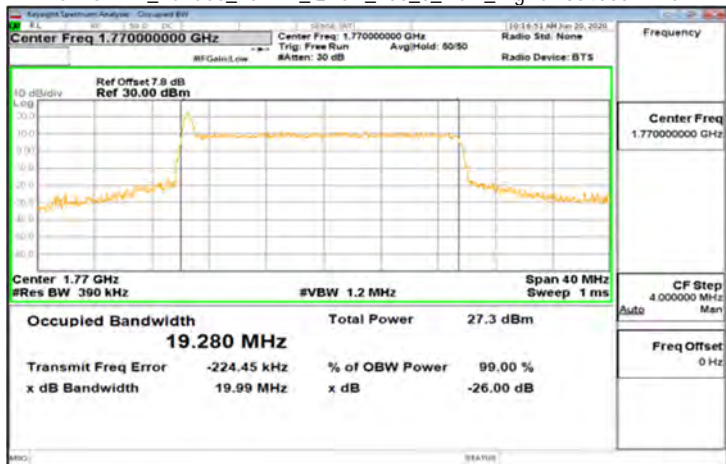
CP-OFDM_Band66_20MHz_QPSK_106_0_Main_HighCH354000-1770
