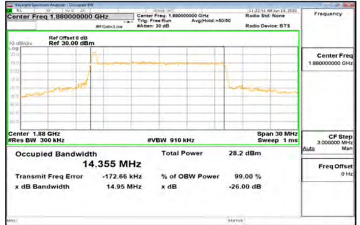
CP-OFDM_Band2_15MHz_64QAM_79_0_Main_MidCH376000-1880
