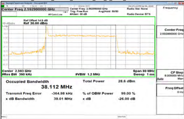
CP-OFDM_Band41_40MHz_256QAM_106_0_Main_MidCH518598-2592.99
