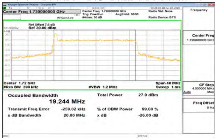
CP-OFDM_Band66_20MHz_16QAM_106_0_Main_LowCH344000-1720
