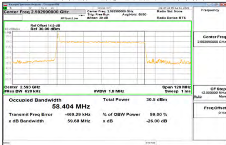
CP-OFDM_Band41_60MHz_64QAM_162_0_Main_MidCH518598
