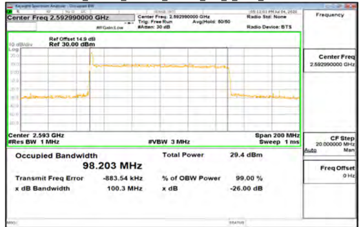
CP-OFDM_Band41_100MHz_64QAM_273_0_Main_MidCH518598
