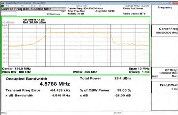
CP-OFDM_Band5_5MHz_16QAM_25_0_Main_MidCH167300-836.5
