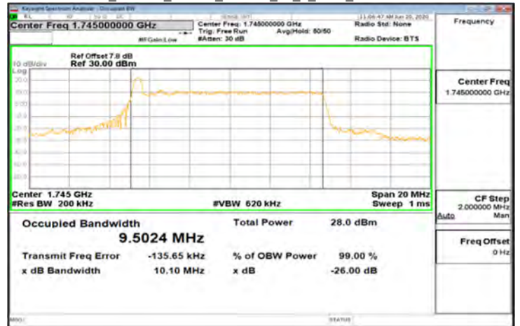
CP-OFDM_Band66_10MHz_64QAM_52_0_Main_MidCH349000-1745
