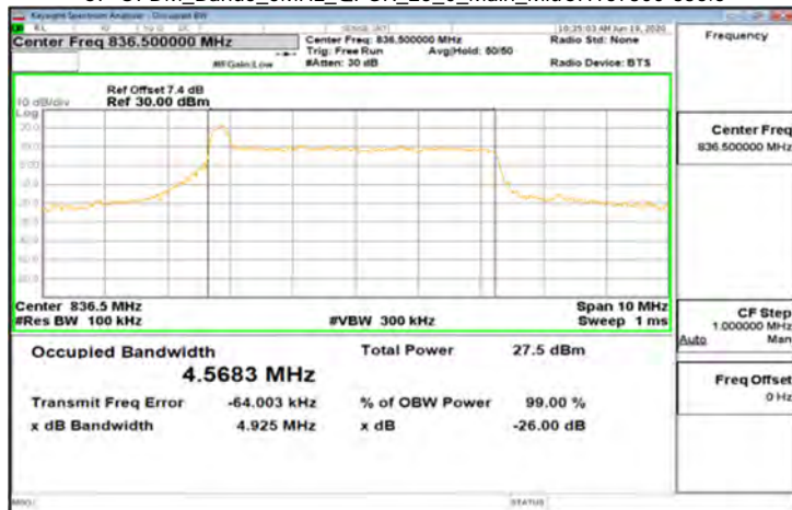
CP-OFDM_Band5_5MHz_QPSK_25_0_Main_MidCH167300-836.5
