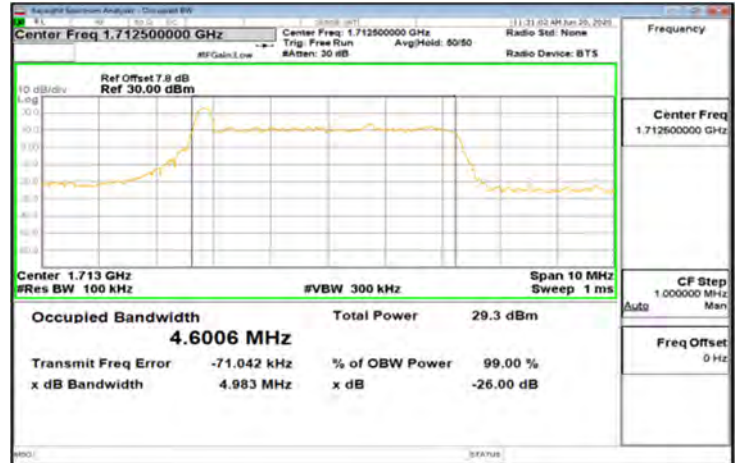
CP-OFDM_Band66_5MHz_64QAM_25_0_Main_LowCH342500-1712.5
