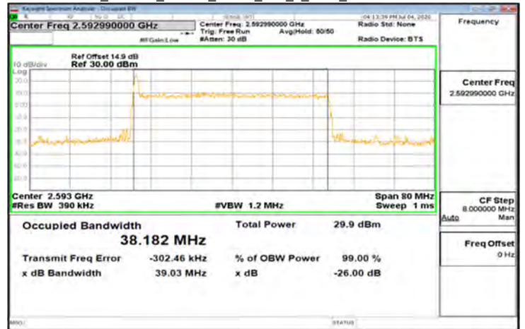
CP-OFDM_Band41_40MHz_QPSK_106_0_Main_MidCH518598-2592.99
