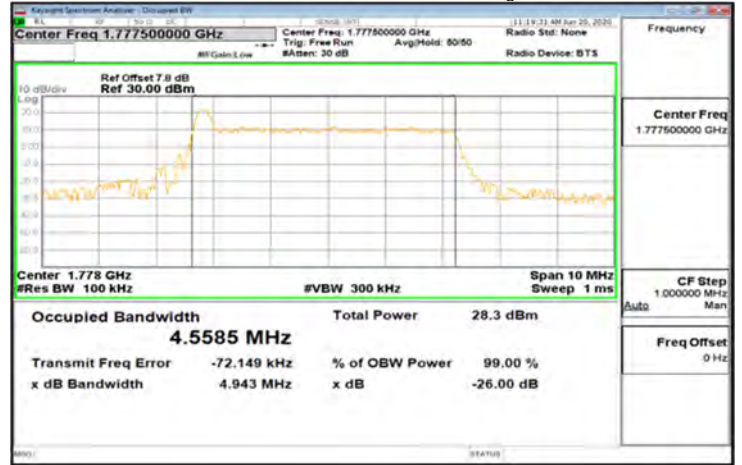
CP-OFDM_Band66_5MHz_16QAM_25_0_Main_HighCH355500-1777.5
