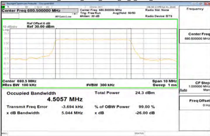
DFT-s-OFDM_Band71_5MHz_QPSK_25_0_Main_MidCH136100
