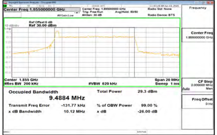
CP-OFDM_Band2_10MHz_QPSK_52_0_Main_LowCH371000-1855
