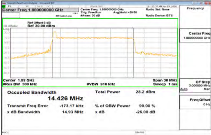
CP-OFDM_Band2_15MHz_16QAM_79_0_Main_MidCH376000-1880
