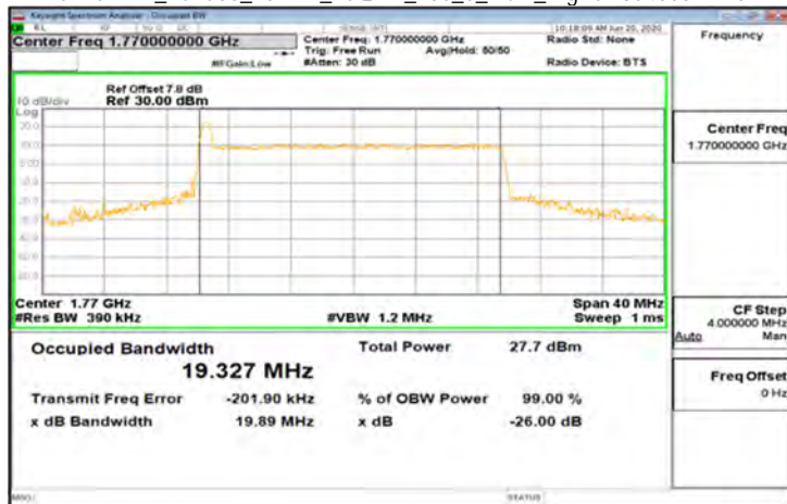
CP-OFDM_Band66_20MHz_16QAM_106_0_Main_HighCH354000-1770
