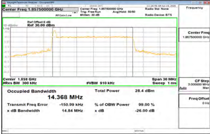
CP-OFDM_Band2_15MHz_16QAM_79_0_Main_LowCH371500-1857.5
