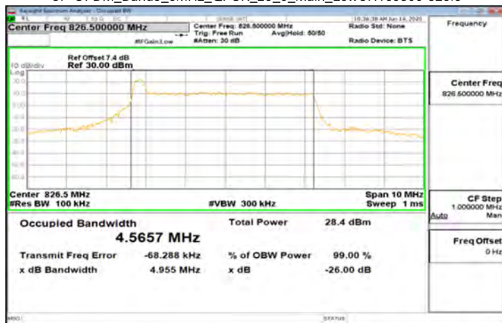
CP-OFDM_Band5_5MHz_QPSK_25_0_Main_LowCH165300-826.5
