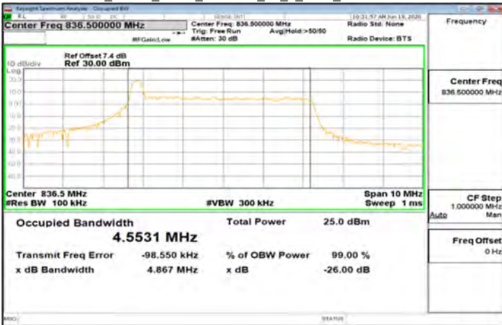
CP-OFDM_Band5_5MHz_256QAM_25_0_Main_MidCH167300-836.5
