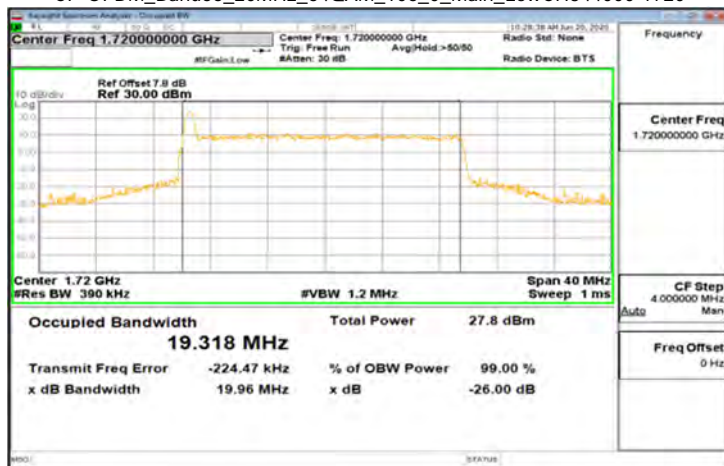
CP-OFDM_Band66_20MHz_64QAM_106_0_Main_LowCH344000-1720
