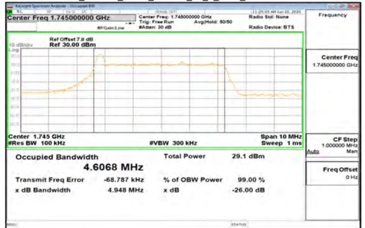
CP-OFDM_Band66_5MHz_64QAM_25_0_Main_MidCH349000-1745
