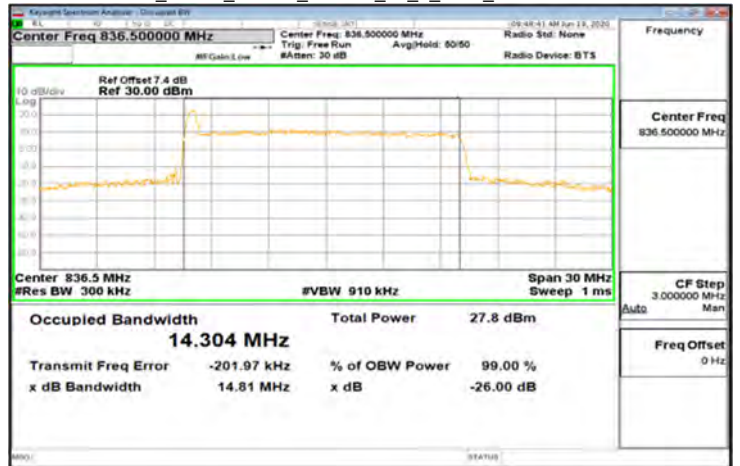
CP-OFDM_Band5_15MHz_64QAM_79_0_Main_MidCH167300-836.5
