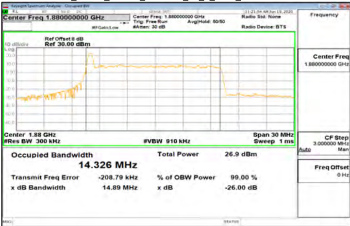
CP-OFDM_Band2_15MHz_256QAM_79_0_Main_MidCH376000-1880
