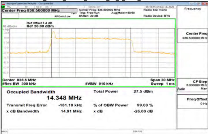
CP-OFDM_Band5_15MHz_16QAM_79_0_Main_MidCH167300-836.5
