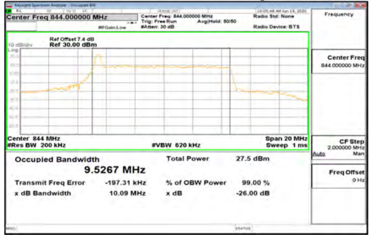
CP-OFDM_Band5_10MHz_64QAM_52_0_Main_LowCH168800-829
