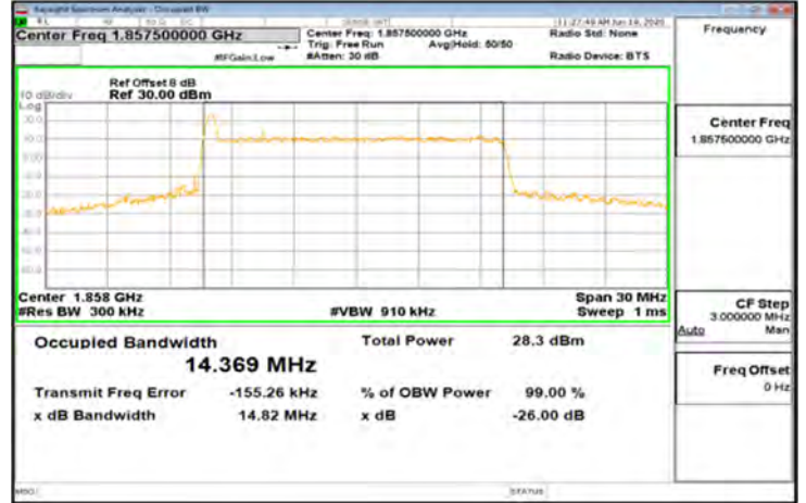
CP-OFDM_Band2_15MHz_64QAM_79_0_Main_LowCH371500-1857.5
