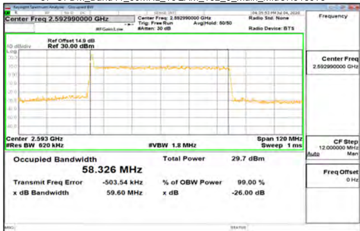
CP-OFDM_Band41_60MHz_16QAM_162_0_Main_MidCH518598
