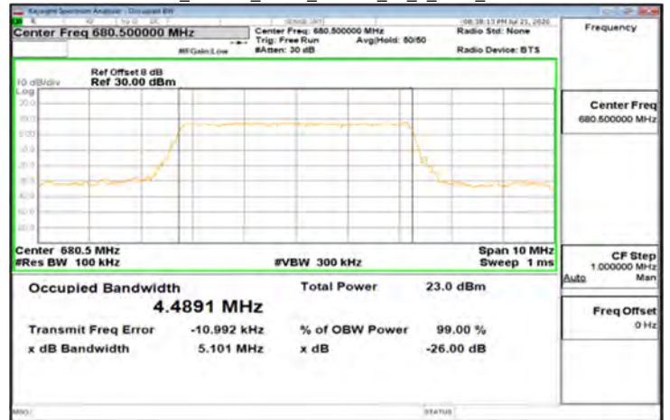
DFT-s-OFDM_Band71_5MHz_16QAM_25_0_Main_MidCH136100
