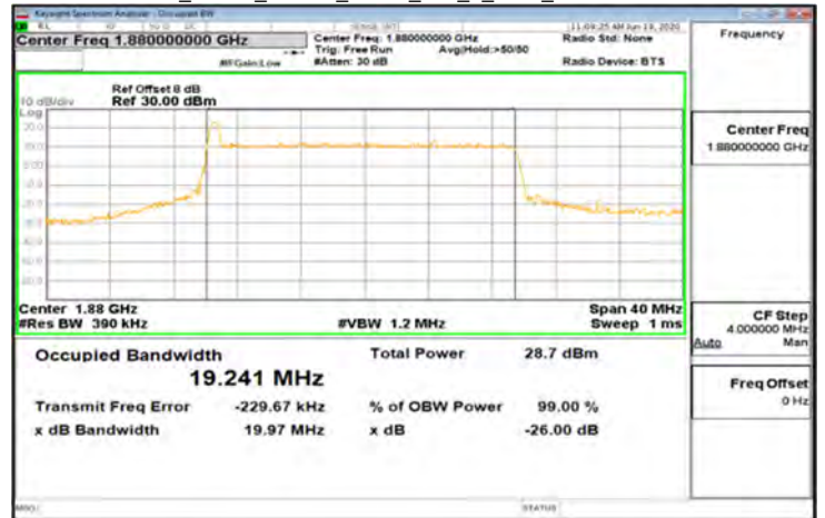
CP-OFDM_Band2_20MHz_QPSK_106_0_Main_MidCH376000-1880
