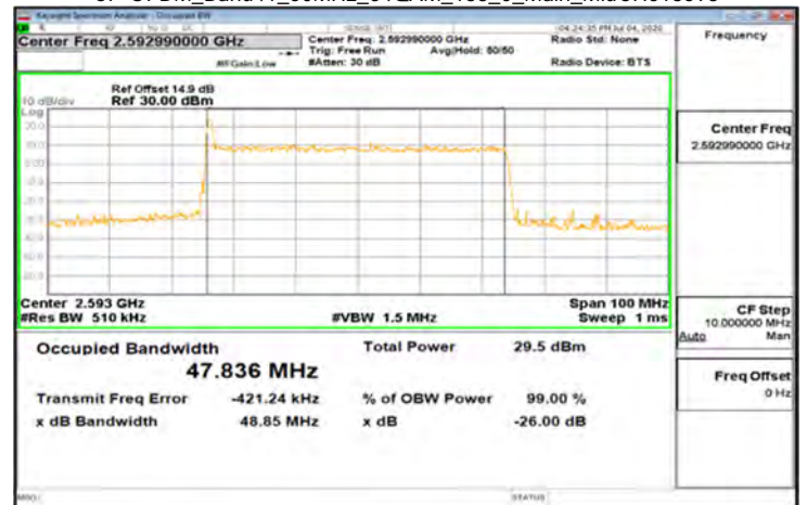
CP-OFDM_Band41_50MHz_64QAM_133_0_Main_MidCH518598
