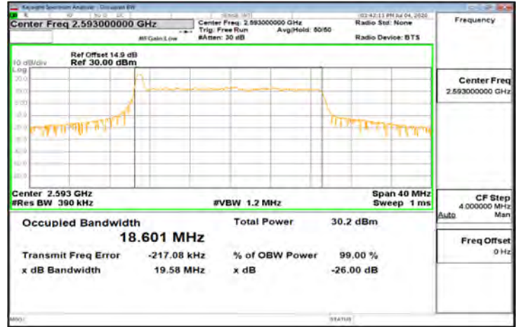
CP-OFDM_Band41_20MHz_QPSK_51_0_Main_MidCH518598-2593
