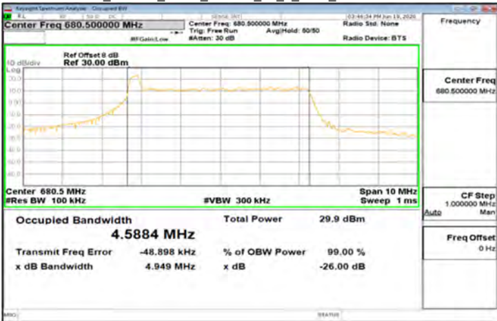
CP-OFDM_Band71_5MHz_16QAM_25_0_Main_MidCH136100-680.5
