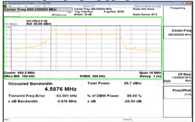
CP-OFDM_Band71_5MHz_QPSK_25_0_Main_MidCH136100-680.5
