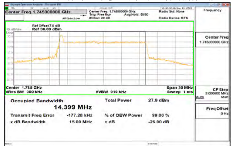
CP-OFDM_Band66_15MHz_64QAM_79_0_Main_MidCH349000-1745
