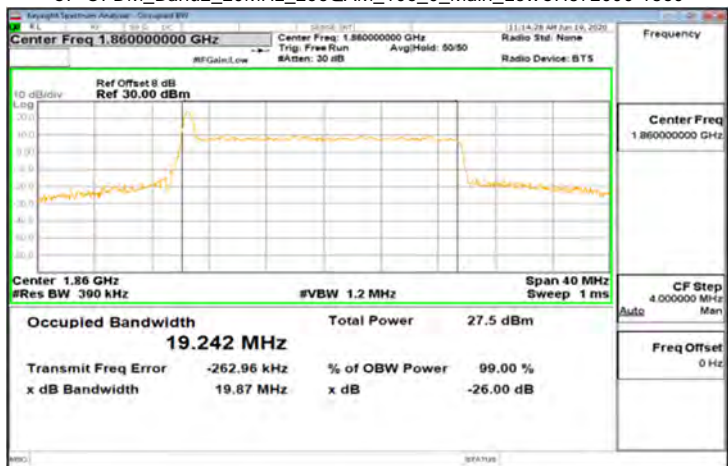
CP-OFDM_Band2_20MHz_256QAM_106_0_Main_LowCH372000-1860
