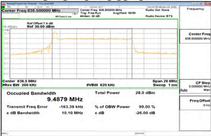
CP-OFDM_Band5_10MHz_16QAM_52_0_Main_MidCH167300-836.5
