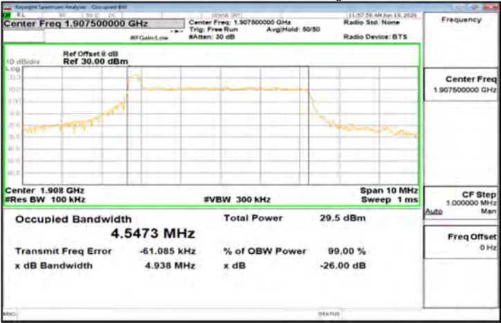
CP-OFDM_Band2_5MHz_QPSK_25_0_Main_HighCH381500-1907.5
