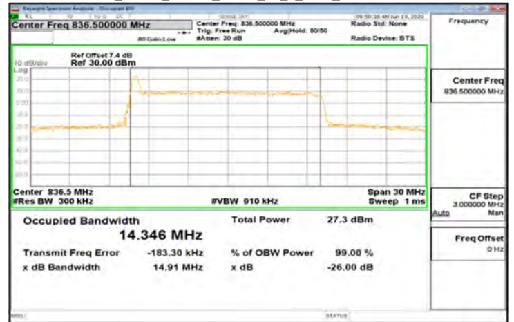
CP-OFDM_Band5_15MHz_QPSK_79_0_Main_MidCH167300-836.5
