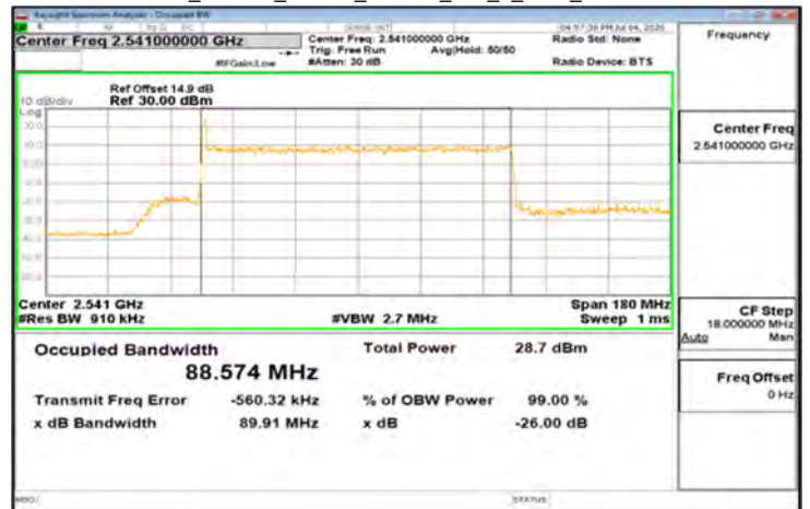
CP-OFDM_Band41_90MHz_64QAM_245_0_Main_MidCH518598
