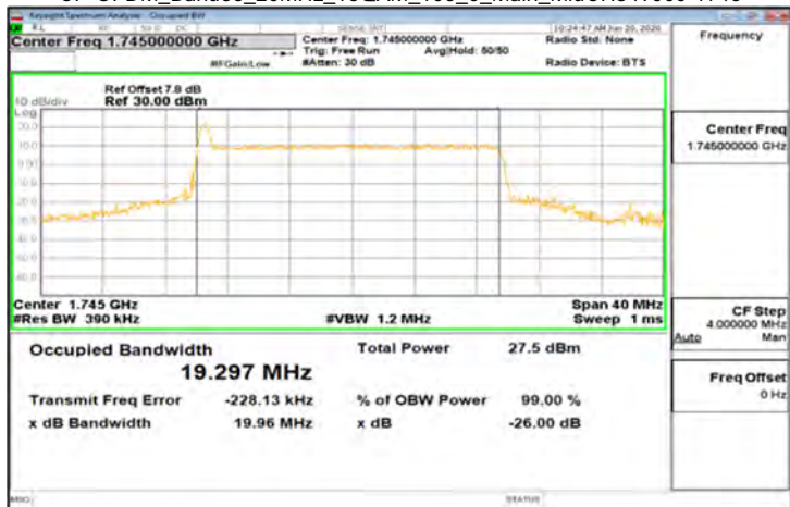
CP-OFDM_Band66_20MHz_16QAM_106_0_Main_MidCH349000-1745
