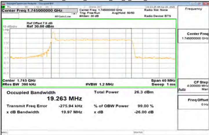
CP-OFDM_Band66_20MHz_256QAM_106_0_Main_MidCH349000-1745
