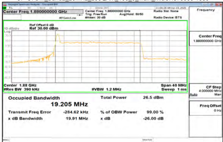
CP-OFDM_Band2_20MHz_256QAM_106_0_Main_MidCH376000-1880
