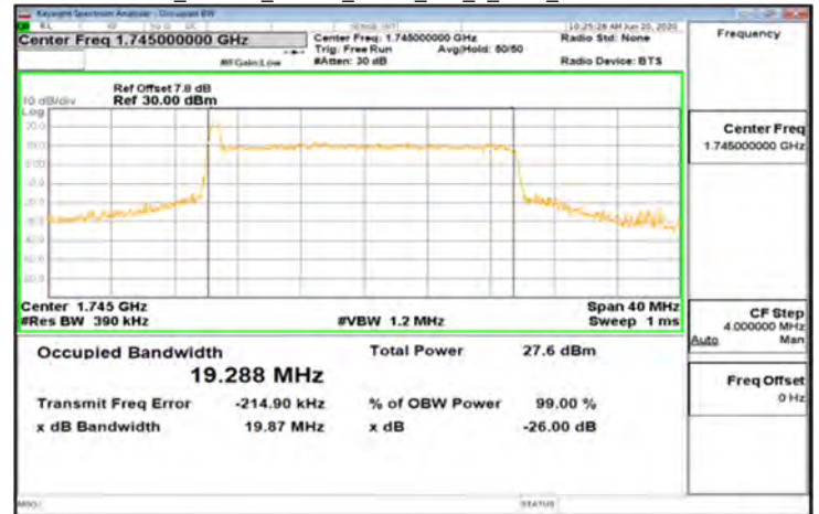
CP-OFDM_Band66_20MHz_QPSK_106_0_Main_MidCH349000-1745
