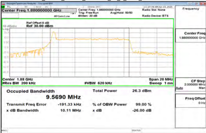
CP-OFDM_Band2_10MHz_256QAM_52_0_Main_MidCH376000-1880
