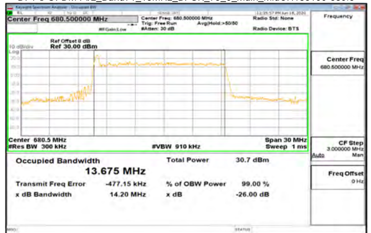
DFT-s-OFDM Pi/2_Band71_15MHz_BPSK_75_0_Main_MidCH136100-680.5
