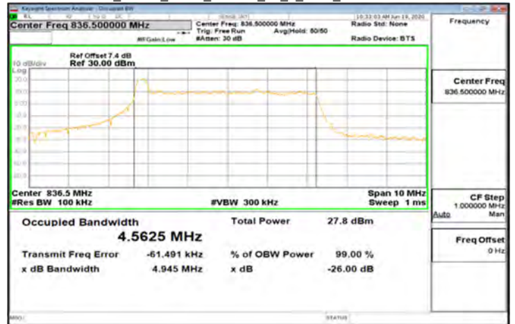
CP-OFDM_Band5_5MHz_64QAM_25_0_Main_MidCH167300-836.5
