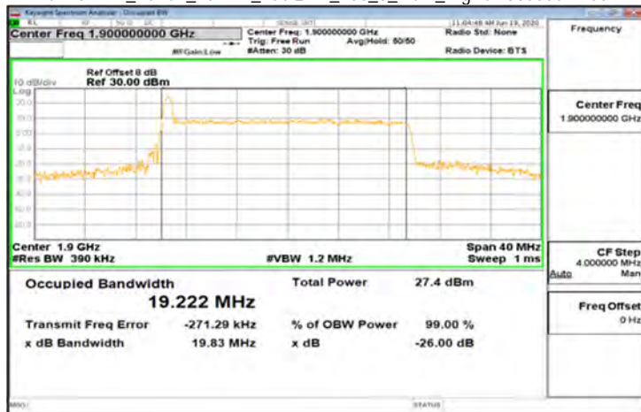
CP-OFDM_Band2_20MHz_256QAM_106_0_Main_HighCH38000-1900
