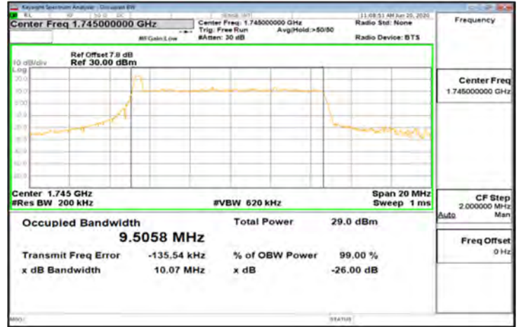
CP-OFDM_Band66_10MHz_QPSK_52_0_Main_MidCH349000-1745
