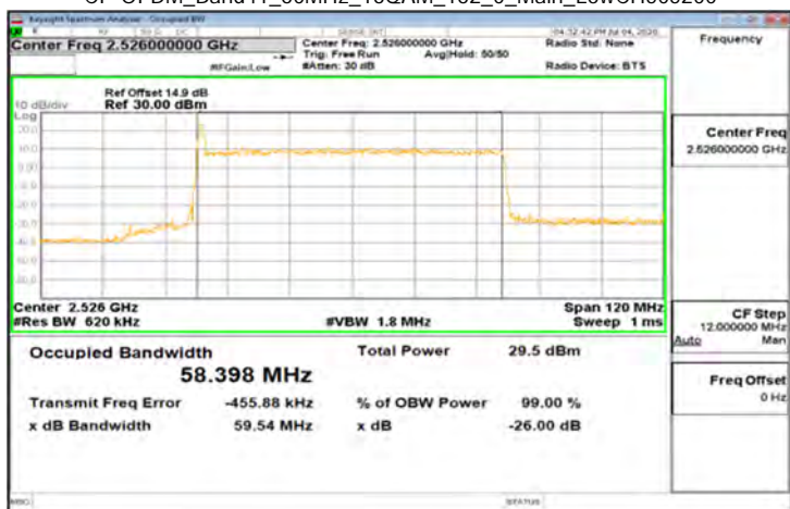
CP-OFDM_Band41_60MHz_16QAM_162_0_Main_LowCH505200
