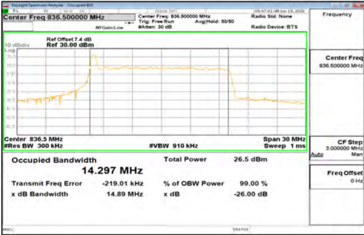
CP-OFDM_Band5_15MHz_256QAM_79_0_Main_MidCH167300-836.5
