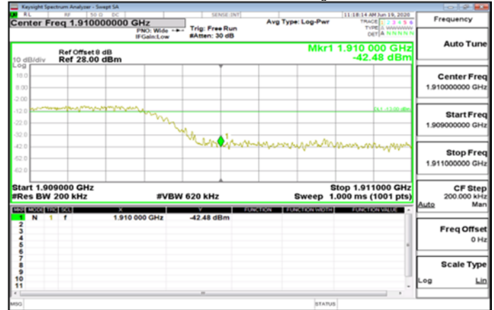
CP-OFDM_Band2_15MHz_QPSK_79_0_HighCH380500-1902.5
