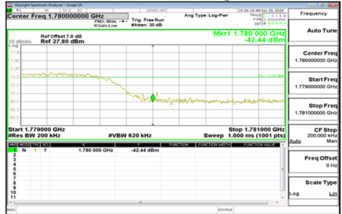
CP-OFDM_Band66_15MHz_QPSK_79_0_HighCH354500-1772.5
