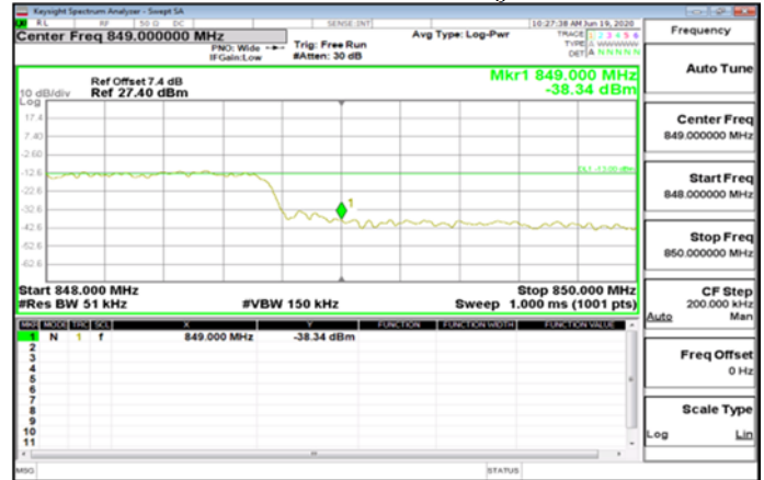
CP-OFDM_Band5_5MHz_QPSK_25_0_HighCH169300-846.5
