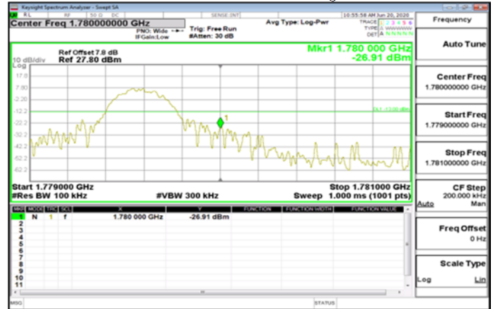
CP-OFDM_Band66_10MHz_QPSK_1_51_HighCH355000-1775
