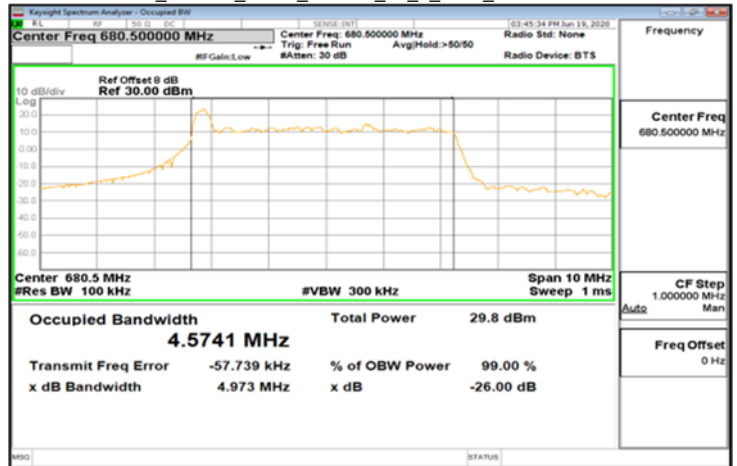
CP-OFDM_Band71_5MHz_64QAM_25_0_Main_MidCH136100-680.5
