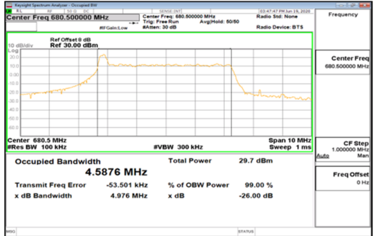
CP-OFDM_Band71_5MHz_QPSK_25_0_Main_MidCH136100-680.5
