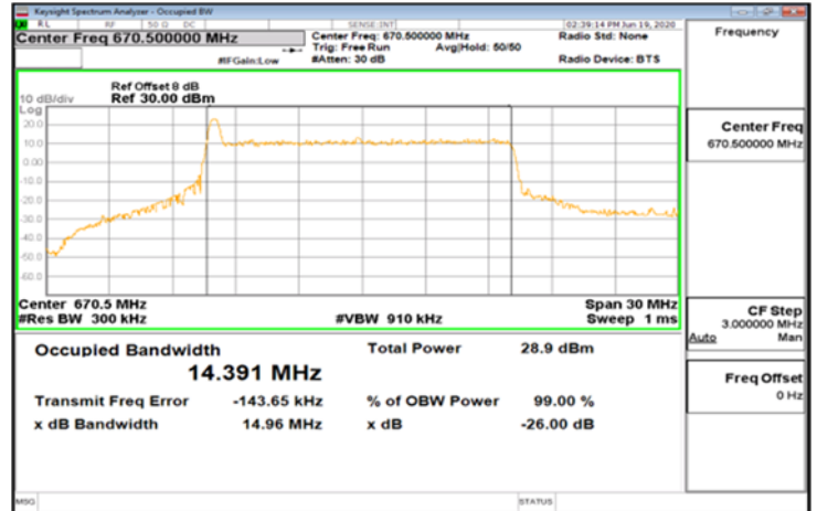
CP-OFDM_Band71_15MHz_QPSK_79_0_Main_LowCH134100-670.5
