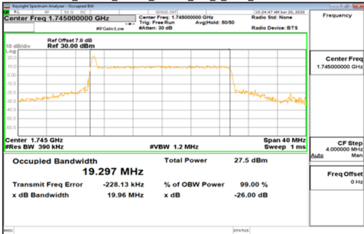
CP-OFDM_Band66_20MHz_16QAM_106_0_Main_MidCH349000-1745
