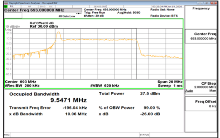
CP-OFDM_Band71_10MHz_256QAM_52_0_Main_HighCH138600-693
