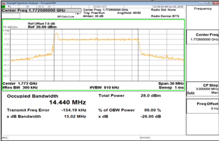
CP-OFDM_Band66_15MHz_QPSK_79_0_Main_HighCH354500-1772.5
