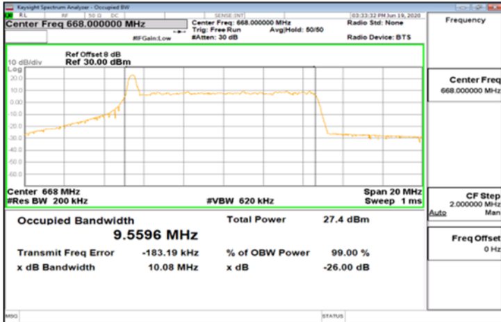
CP-OFDM_Band71_10MHz_256QAM_52_0_Main_LowCH133600-668
