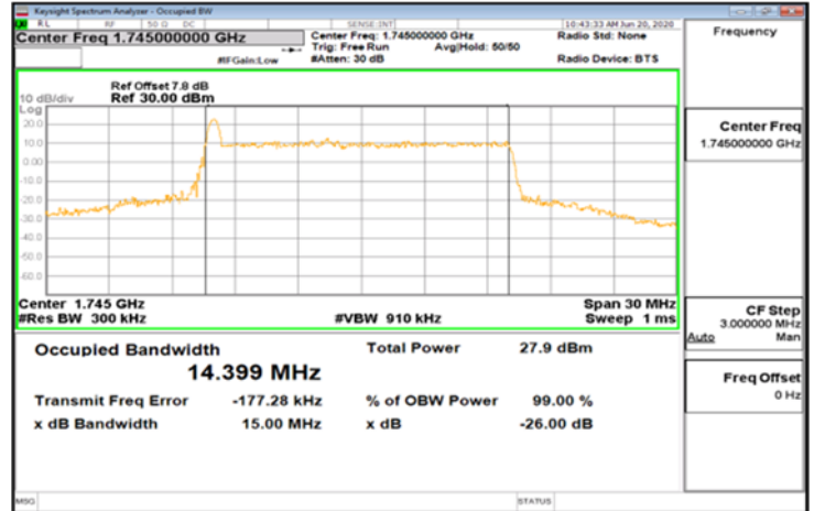
CP-OFDM_Band66_15MHz_64QAM_79_0_Main_MidCH349000-1745
