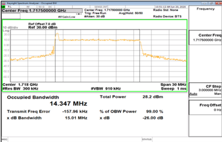
CP-OFDM_Band66_15MHz_16QAM_79_0_Main_LowCH343500-1717.5
