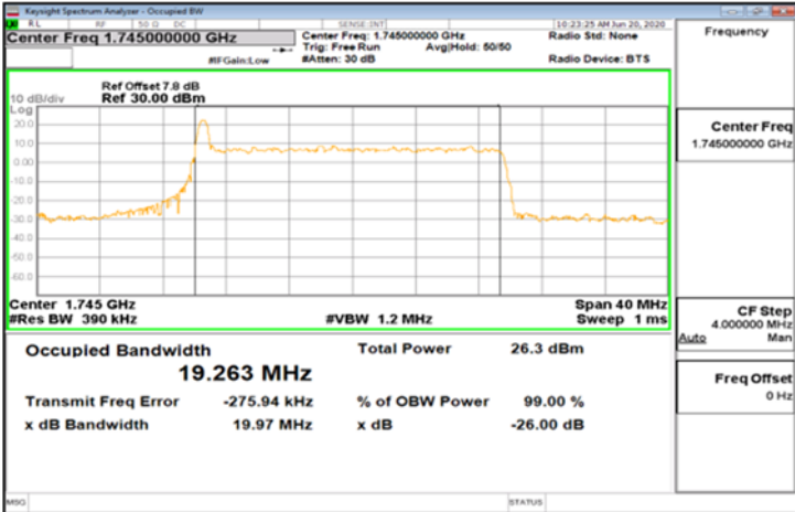
CP-OFDM_Band66_20MHz_256QAM_106_0_Main_MidCH349000-1745
