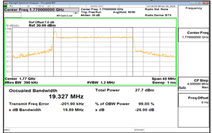
CP-OFDM_Band66_20MHz_16QAM_106_0_Main_HighCH354000-1770
