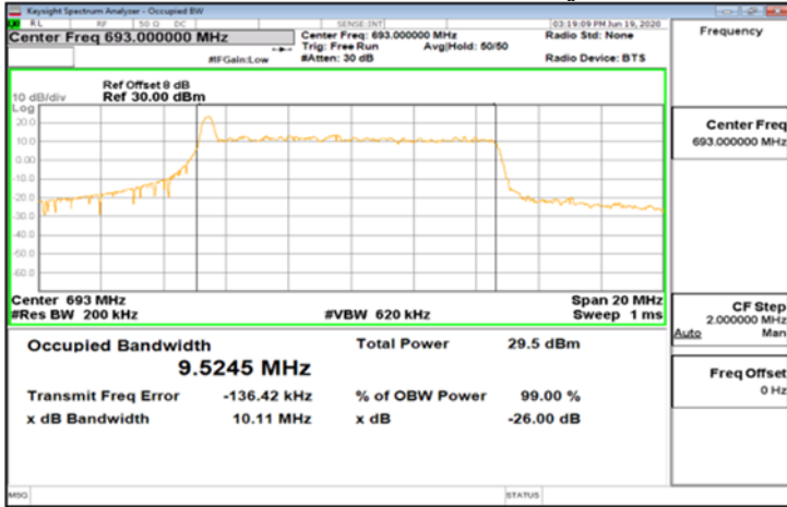
CP-OFDM_Band71_10MHz_64QAM_52_0_Main_HighCH138600-693
