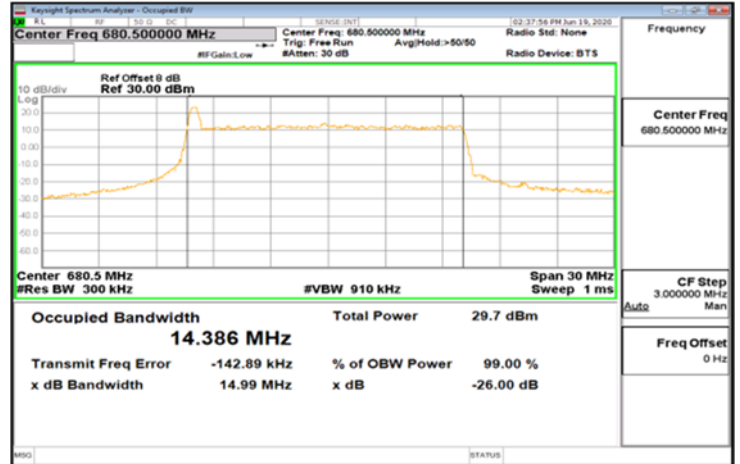
CP-OFDM_Band71_15MHz_QPSK_79_0_Main_MidCH136100-680.5
