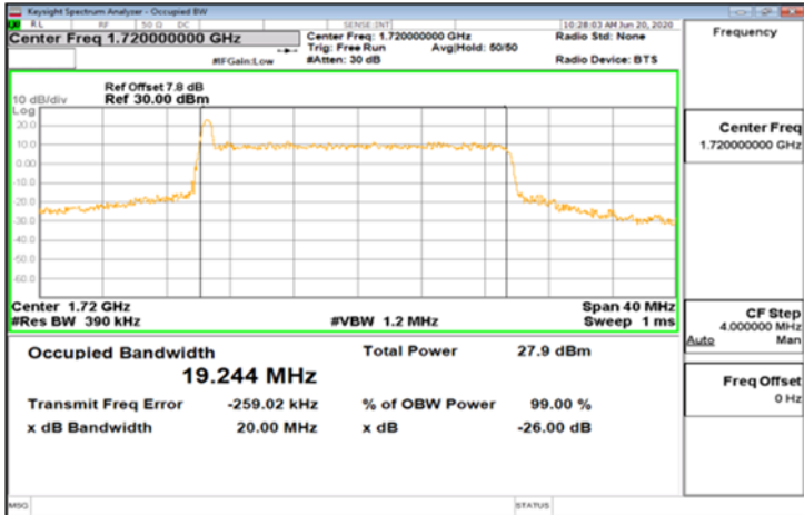
CP-OFDM_Band66_20MHz_16QAM_106_0_Main_LowCH344000-1720
