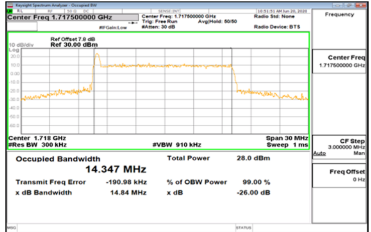
CP-OFDM_Band66_15MHz_64QAM_79_0_Main_LowCH343500-1717.5
