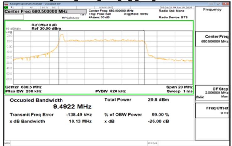
CP-OFDM_Band71_10MHz_QPSK_52_0_Main_MidCH136100-680.5
