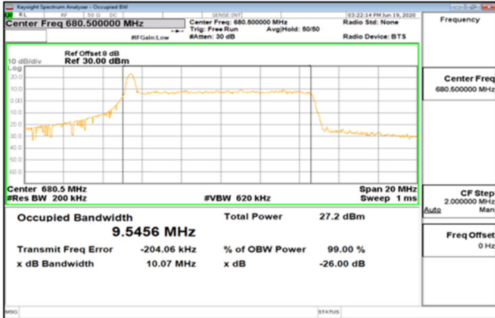
CP-OFDM_Band71_10MHz_256QAM_52_0_Main_MidCH136100-680.5
