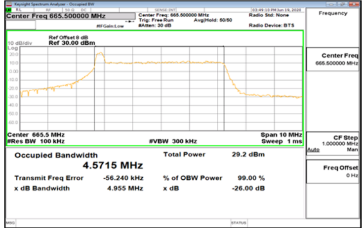
CP-OFDM_Band71_5MHz_QPSK_25_0_Main_LowCH133100-665.5
