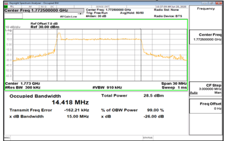
CP-OFDM_Band66_15MHz_16QAM_79_0_Main_HighCH354500-1772.5
