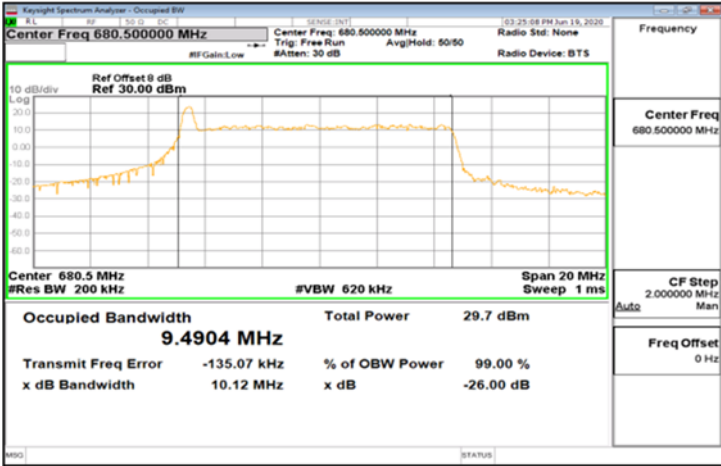
CP-OFDM_Band71_10MHz_16QAM_52_0_Main_MidCH136100-680.5
