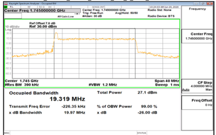
CP-OFDM_Band66_20MHz_64QAM_106_0_Main_MidCH349000-1745
