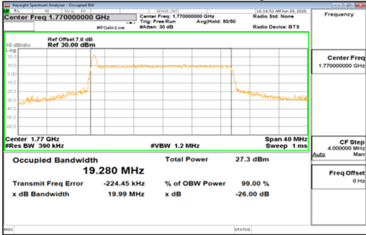
CP-OFDM_Band66_20MHz_QPSK_106_0_Main_HighCH354000-1770
