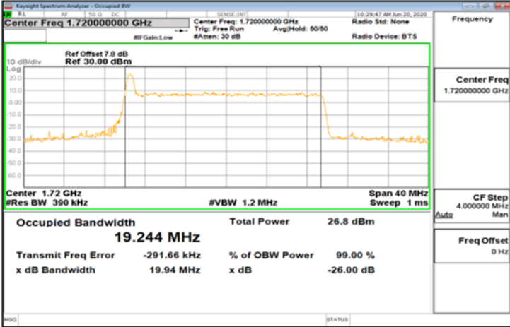
CP-OFDM_Band66_20MHz_256QAM_106_0_Main_LowCH344000-1720
