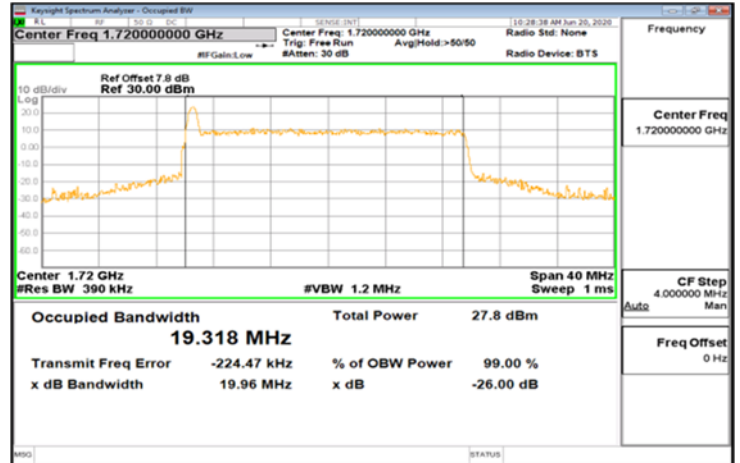
CP-OFDM_Band66_20MHz_64QAM_106_0_Main_LowCH344000-1720
