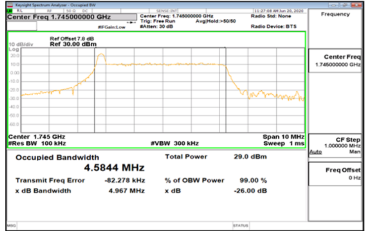
CP-OFDM_Band66_5MHz_QPSK_25_0_Main_MidCH349000-1745
