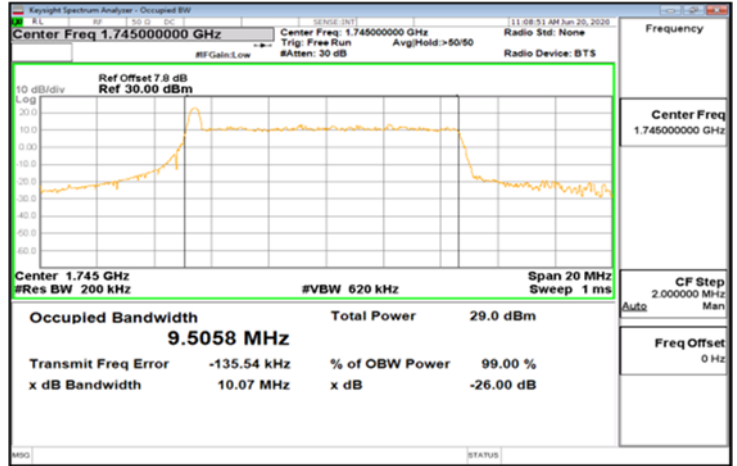
CP-OFDM_Band66_10MHz_QPSK_52_0_Main_MidCH349000-1745
