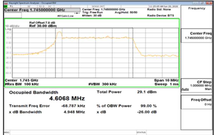
CP-OFDM_Band66_5MHz_64QAM_25_0_Main_MidCH349000-1745
