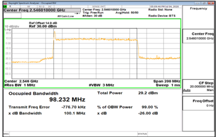
CP-OFDM_Band41_100MHz_64QAM_273_0_Main_MidCH518598
