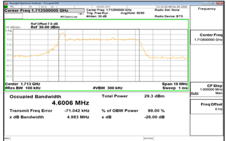
CP-OFDM_Band66_5MHz_64QAM_25_0_Main_LowCH342500-1712.5
