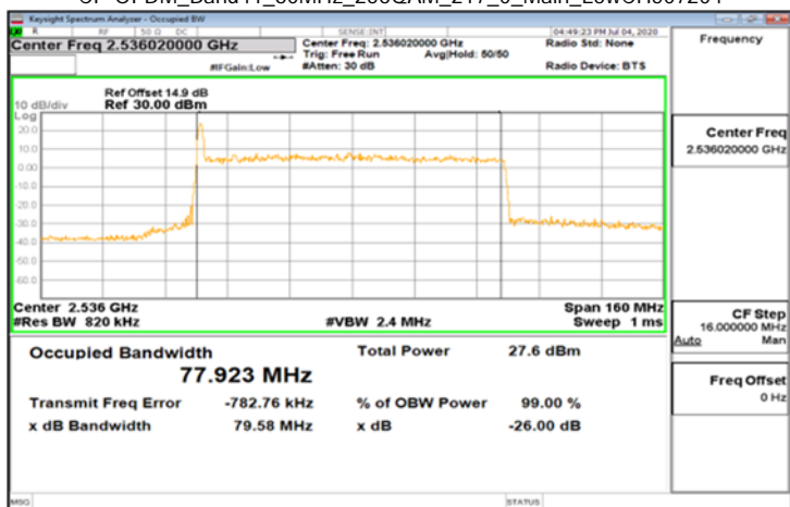
CP-OFDM_Band41_80MHz_256QAM_217_0_Main_LowCH507204
