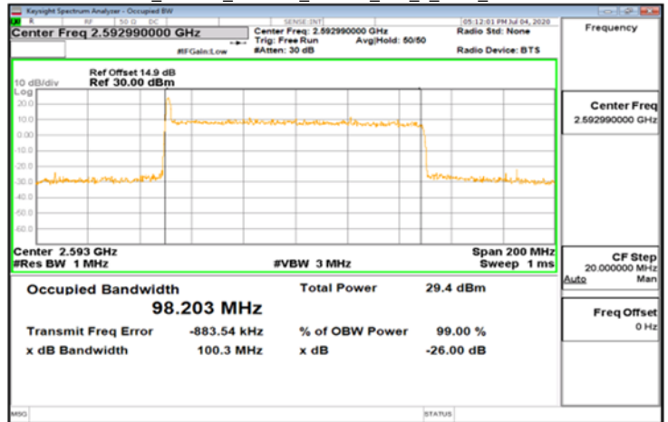
CP-OFDM_Band41_100MHz_64QAM_273_0_Main_MidCH518598
