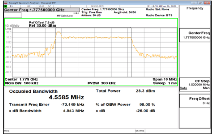
CP-OFDM_Band66_5MHz_16QAM_25_0_Main_HighCH355500-1777.5
