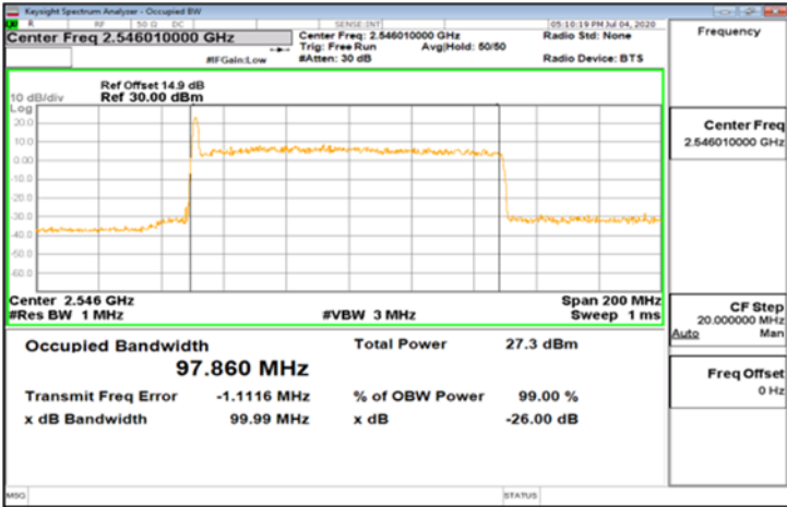
CP-OFDM_Band41_100MHz_256QAM_273_0_Main_LowCH509202
