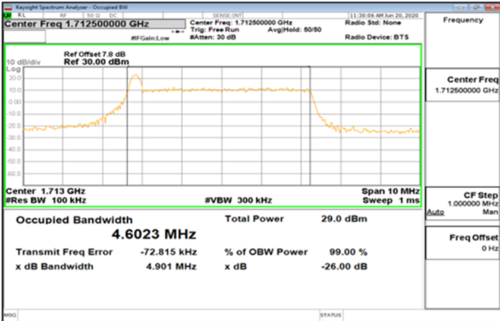
CP-OFDM_Band66_5MHz_16QAM_25_0_Main_LowCH342500-1712.5
