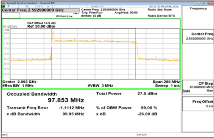
CP-OFDM_Band41_100MHz_256QAM_273_0_Main_MidCH518598
