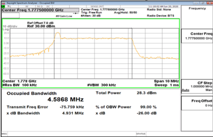
CP-OFDM_Band66_5MHz_QPSK_25_0_Main_HighCH355500-1777.5
