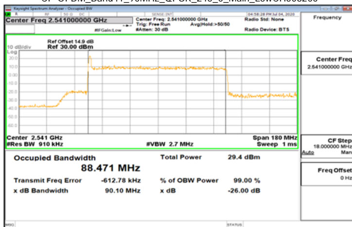
CP-OFDM_Band41_90MHz_QPSK_245_0_Main_LowCH508200
