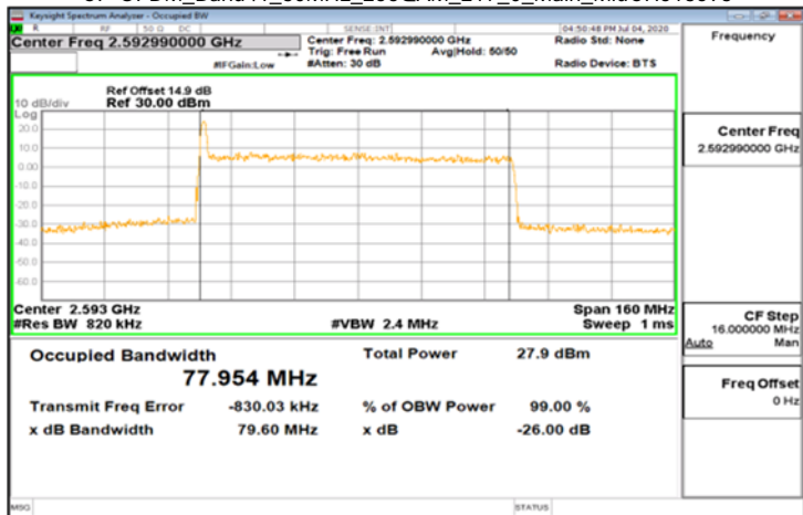
CP-OFDM_Band41_80MHz_256QAM_217_0_Main_MidCH518598
