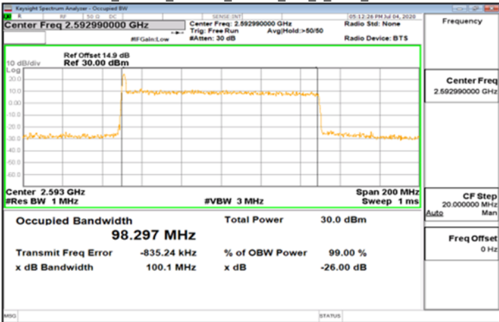
CP-OFDM_Band41_100MHz_16QAM_273_0_Main_MidCH518598
