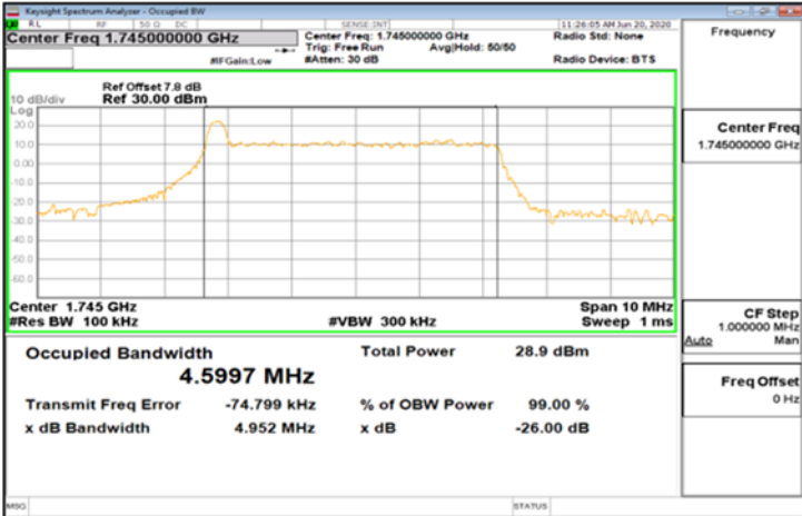
CP-OFDM_Band66_5MHz_16QAM_25_0_Main_MidCH349000-1745
