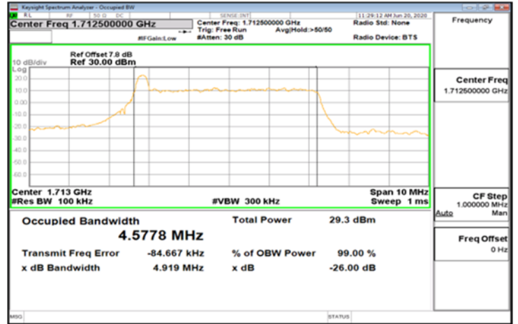
CP-OFDM_Band66_5MHz_QPSK_25_0_Main_LowCH342500-1712.5
