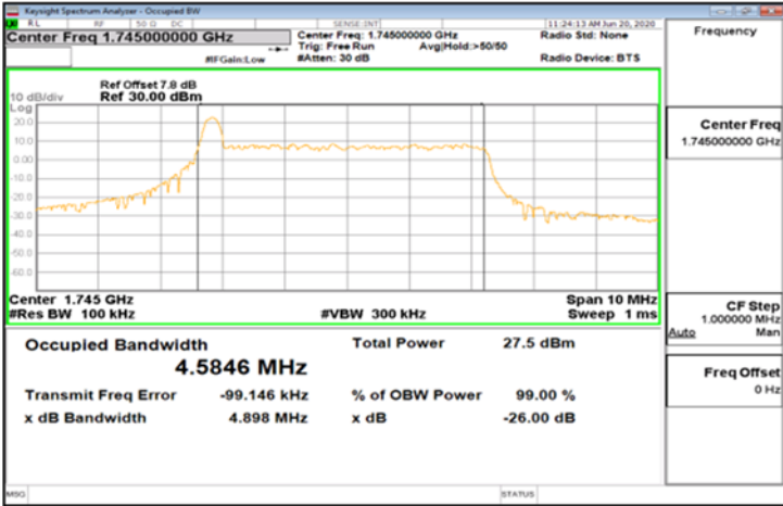
CP-OFDM_Band66_5MHz_256QAM_25_0_Main_MidCH349000-1745
