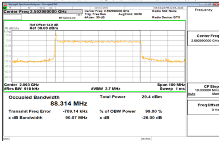
CP-OFDM_Band41_90MHz_QPSK_245_0_Main_MidCH518598
