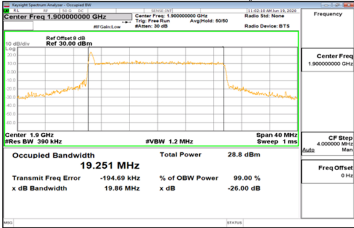
CP-OFDM_Band2_20MHz_QPSK_106_0_Main_HighCH38000-1900
