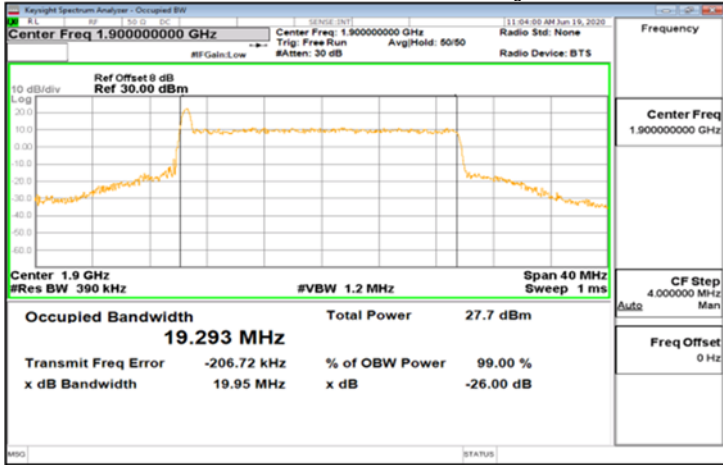
CP-OFDM_Band2_20MHz_64QAM_106_0_Main_HighCH38000-1900
