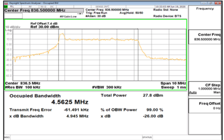
CP-OFDM_Band5_5MHz_64QAM_25_0_Main_MidCH167300-836.5
