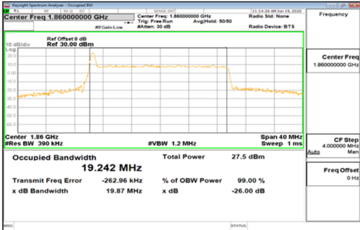
CP-OFDM_Band2_20MHz_256QAM_106_0_Main_LowCH372000-1860
