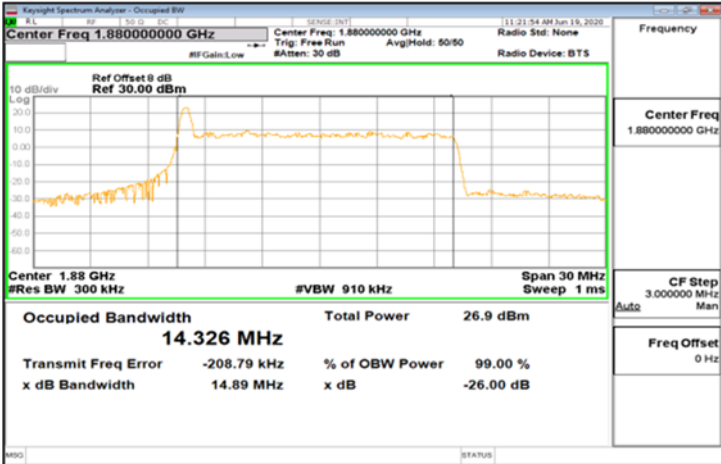
CP-OFDM_Band2_15MHz_256QAM_79_0_Main_MidCH376000-1880
