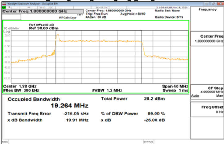
CP-OFDM_Band2_20MHz_16QAM_106_0_Main_MidCH37600-1880
