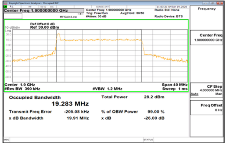
CP-OFDM_Band2_20MHz_16QAM_106_0_Main_HighCH38000-1900
