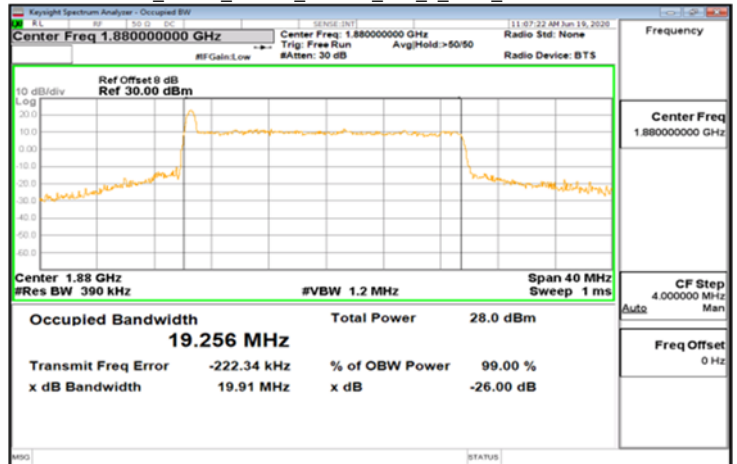
CP-OFDM_Band2_20MHz_64QAM_106_0_Main_MidCH37600-1880
