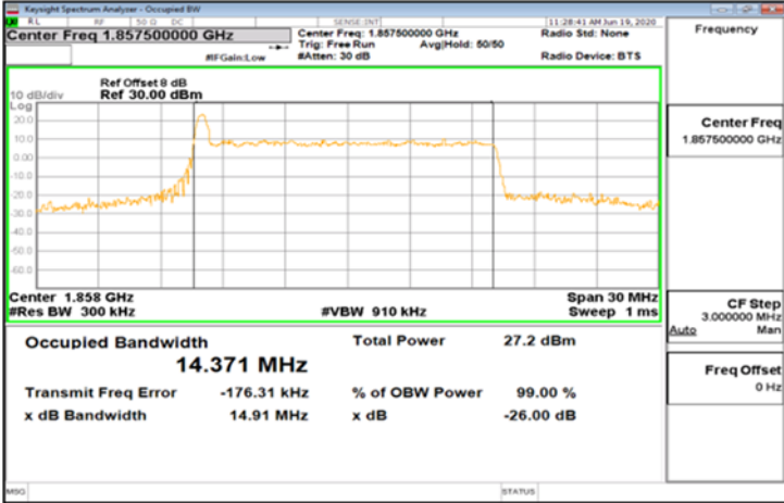
CP-OFDM_Band2_15MHz_256QAM_79_0_Main_LowCH371500-1857.5
