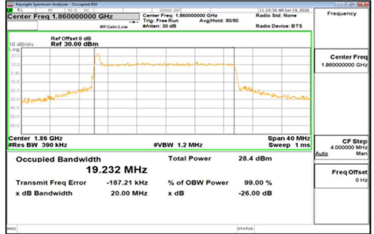
CP-OFDM_Band2_20MHz_QPSK_106_0_Main_LowCH372000-1860
