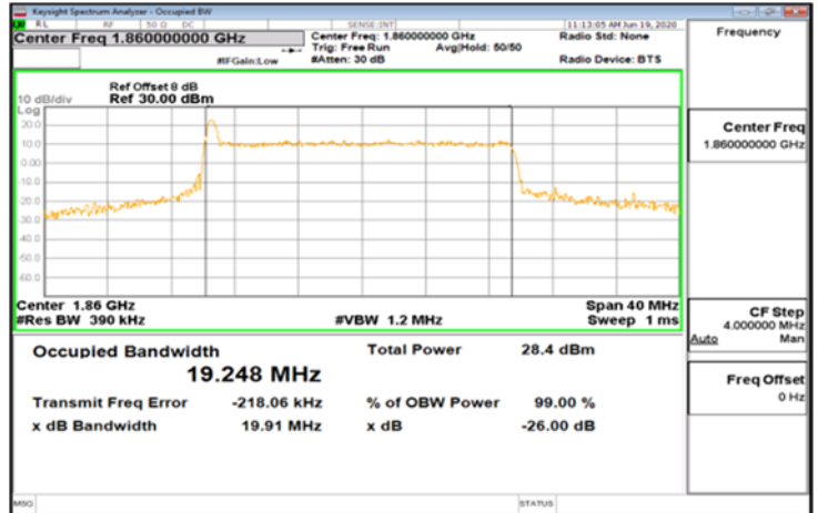
CP-OFDM_Band2_20MHz_64QAM_106_0_Main_LowCH37200-1860
