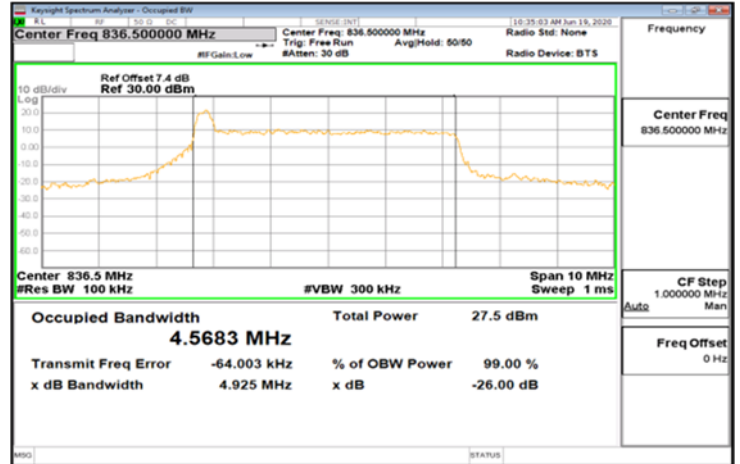
CP-OFDM_Band5_5MHz_QPSK_25_0_Main_MidCH167300-836.5
