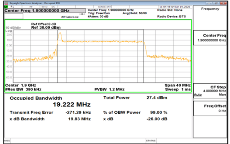
CP-OFDM_Band2_20MHz_256QAM_106_0_Main_HighCH38000-1900
