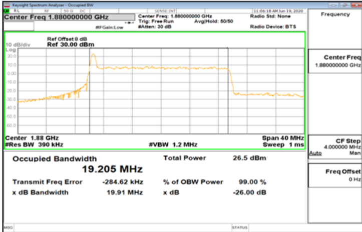
CP-OFDM_Band2_20MHz_256QAM_106_0_Main_MidCH376000-1880
