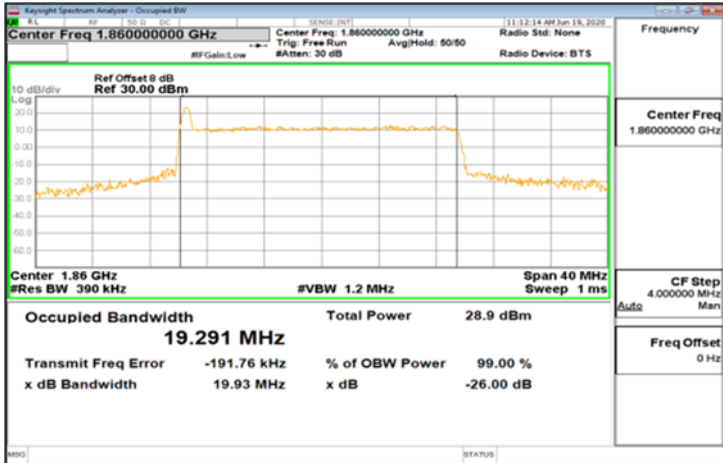
CP-OFDM_Band2_20MHz_16QAM_106_0_Main_LowCH37200-1860
