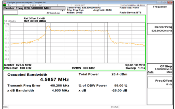
CP-OFDM_Band5_5MHz_QPSK_25_0_Main_LowCH165300-826.5
