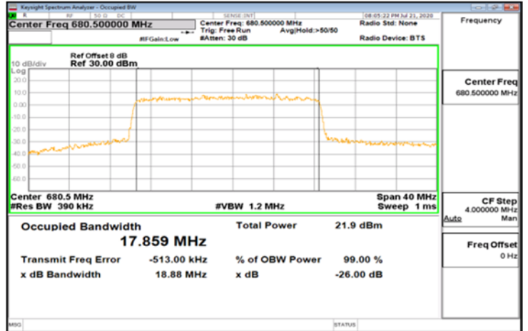
DFT-s-OFDM_Band71_20MHz_64QAM_100_0_Main_MidCH136100
