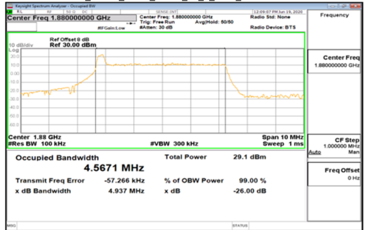
CP-OFDM_Band2_5MHz_QPSK_25_0_Main_MidCH376000-1880
