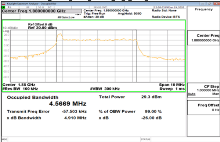
CP-OFDM_Band2_5MHz_16QAM_25_0_Main_MidCH376000-1880
