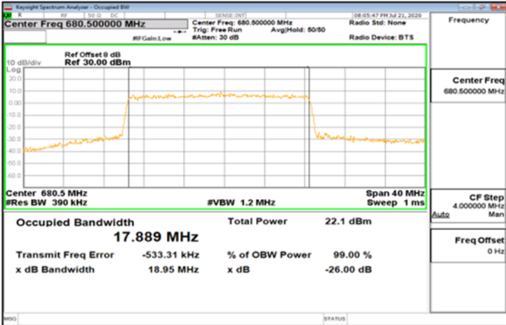
DFT-s-OFDM_Band71_20MHz_16QAM_100_0_Main_MidCH136100
