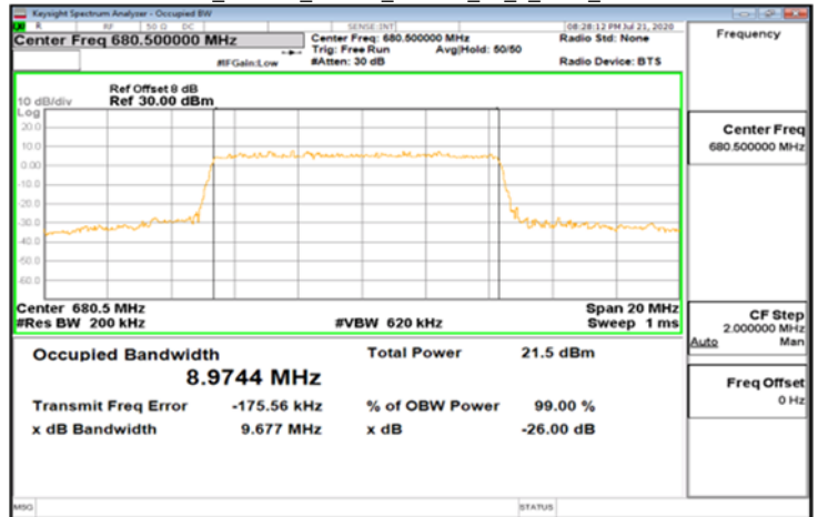
DFT-s-OFDM_Band71_10MHz_64QAM_50_0_Main_MidCH136100
