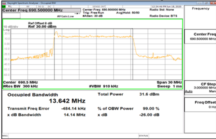
DFT-s-OFDM Pi/2_Band71_15MHz_BPSK_75_0_Main_HighCH138100-690.5
