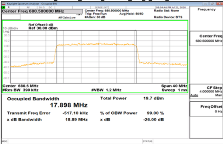
DFT-s-OFDM_Band71_20MHz_256QAM_100_0_Main_MidCH136100
