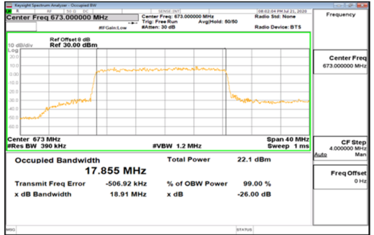
DFT-s-OFDM_Band71_20MHz_64QAM_100_0_Main_LowCH134600
