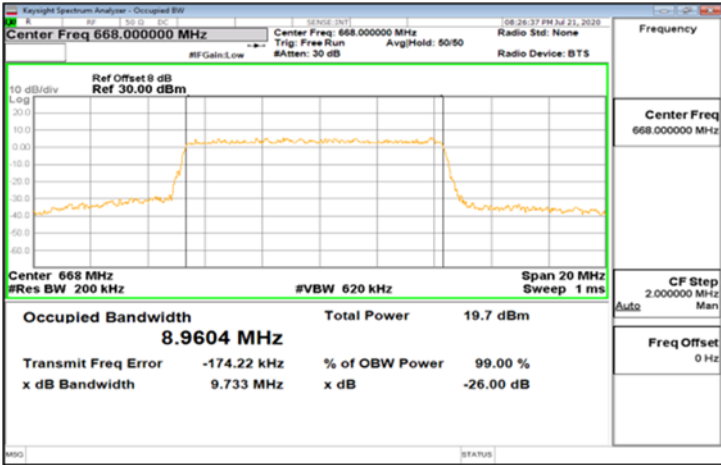
DFT-s-OFDM_Band71_10MHz_256QAM_50_0_Main_LowCH133600
