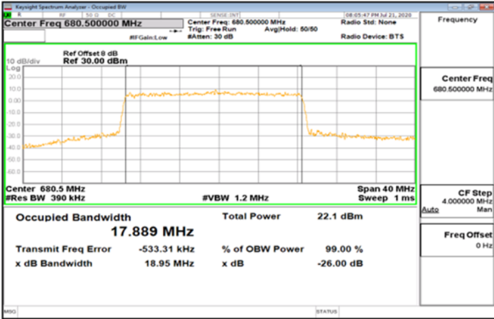
DFT-s-OFDM_Band71_20MHz_16QAM_100_0_Main_MidCH136100
