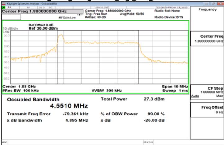
CP-OFDM_Band2_5MHz_256QAM_25_0_Main_MidCH376000-1880
