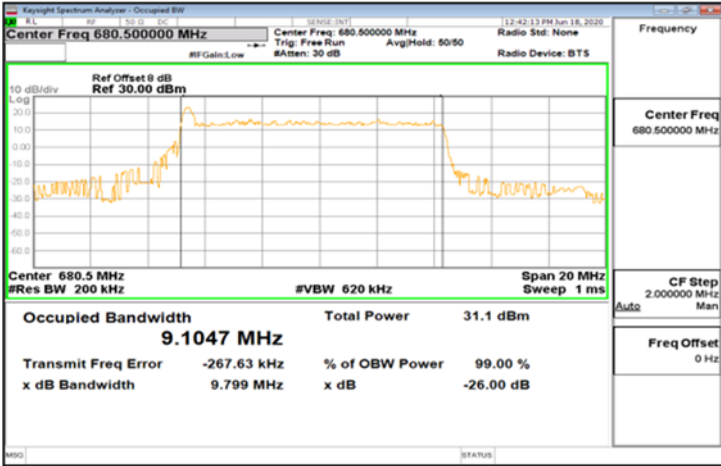
DFT-s-OFDM Pi/2_Band71_10MHz_BPSK_50_0_Main_MidCH136100-680.5
