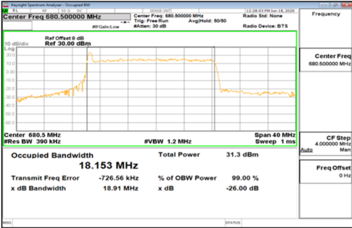
DFT-s-OFDM Pi/2_Band71_20MHz_BPSK_100_0_Main_MidCH136100-680.5
