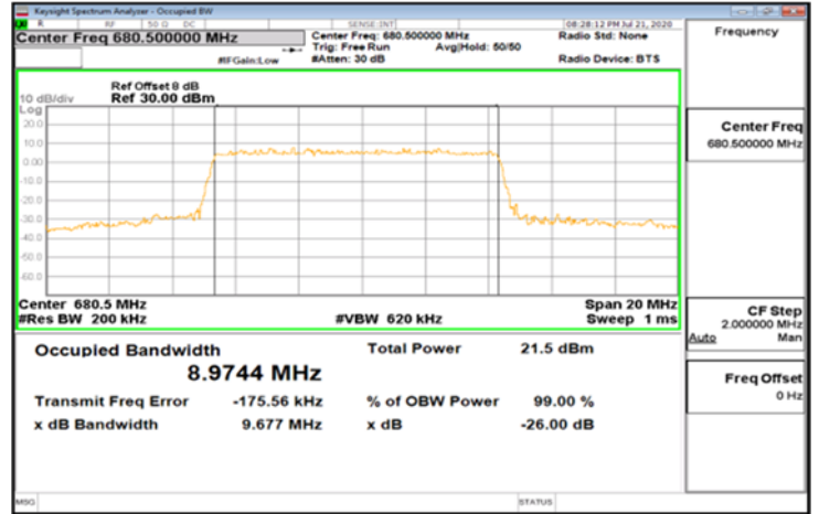
DFT-s-OFDM_Band71_10MHz_64QAM_50_0_Main_MidCH136100
