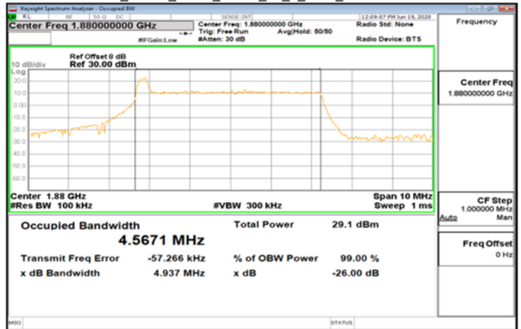
CP-OFDM_Band2_5MHz_QPSK_25_0_Main_MidCH376000-1880
