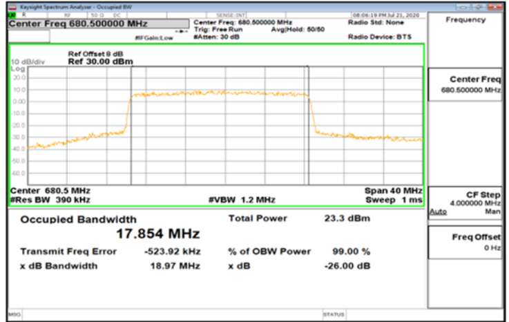
DFT-s-OFDM_Band71_20MHz_QPSK_100_0_Main_MidCH136100
