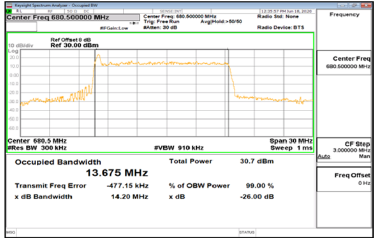
DFT-s-OFDM Pi/2_Band71_15MHz_BPSK_75_0_Main_MidCH136100-680.5
