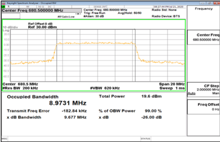
DFT-s-OFDM_Band71_10MHz_256QAM_50_0_Main_MidCH136100
