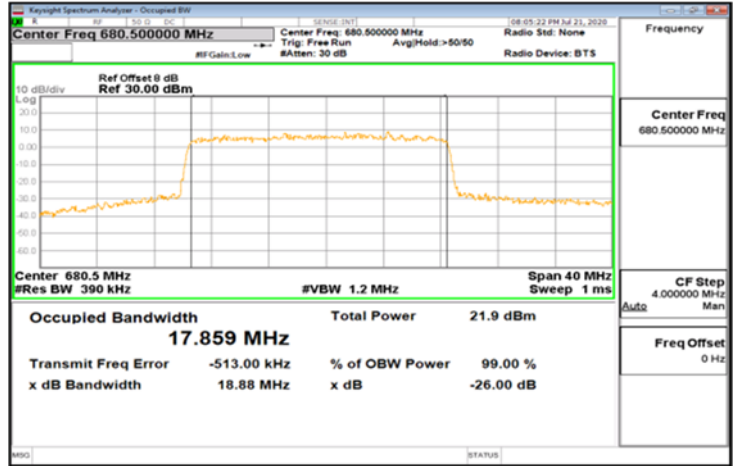
DFT-s-OFDM_Band71_20MHz_64QAM_100_0_Main_MidCH136100
