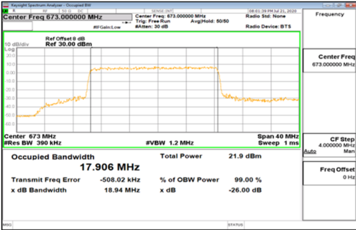
DFT-s-OFDM_Band71_20MHz_16QAM_100_0_Main_LowCH134600
