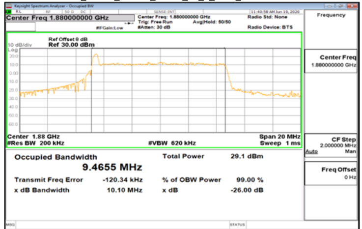
CP-OFDM_Band2_10MHz_QPSK_52_0_Main_MidCH376000-1880
