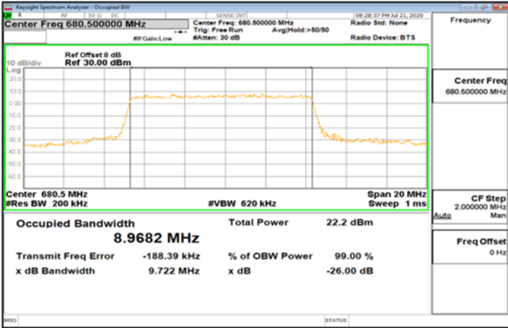
DFT-s-OFDM_Band71_10MHz_16QAM_50_0_Main_MidCH136100
