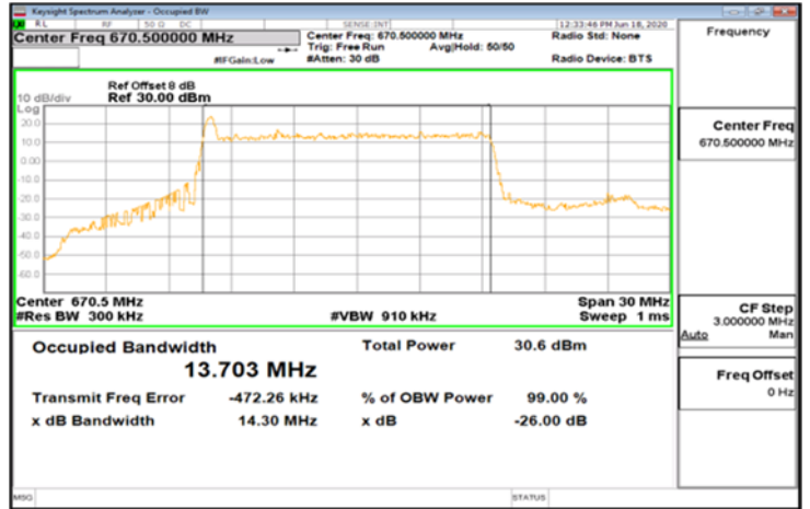
DFT-s-OFDM Pi/2_Band71_15MHz_BPSK_75_0_Main_LowCH134100-670.5
