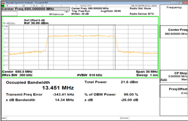
DFT-s-OFDM_Band71_15MHz_64QAM_75_0_Main_MidCH136100
