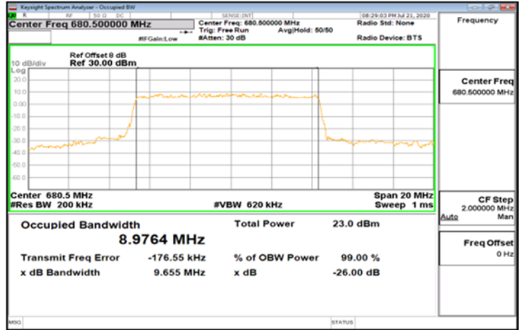
DFT-s-OFDM_Band71_10MHz_QPSK_50_0_Main_MidCH136100
