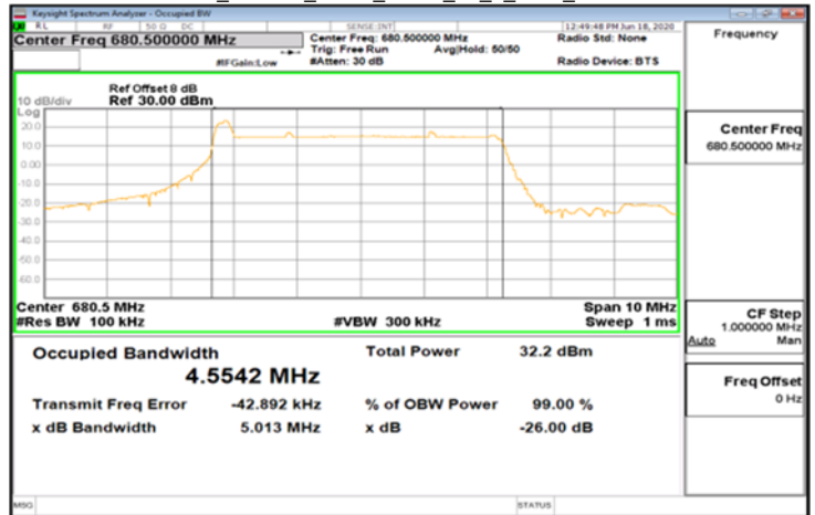
DFT-s-OFDM Pi/2_Band71_5MHz_BPSK_25_0_Main_MidCH136100-680.5
