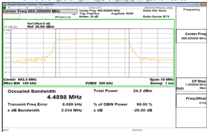
DFT-s-OFDM_Band71_5MHz_QPSK_25_0_Main_LowCH133100
