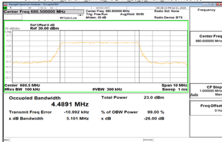
DFT-s-OFDM_Band71_5MHz_16QAM_25_0_Main_MidCH136100
