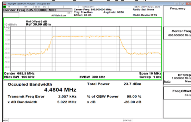
DFT-s-OFDM_Band71_5MHz_QPSK_25_0_Main_HighCH139100
