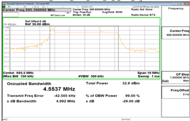
DFT-s-OFDM Pi/2_Band71_5MHz_BPSK_25_0_Main_HighCH139100-695.5
