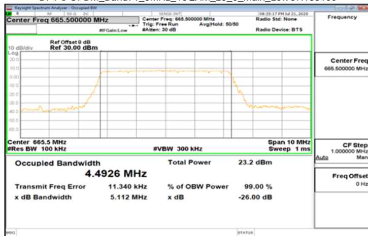
DFT-s-OFDM_Band71_5MHz_16QAM_25_0_Main_LowCH133100
