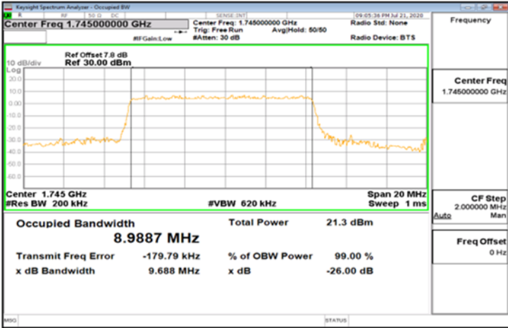
DFT-s-OFDM_Band66_10MHz_16QAM_50_0_Main_MidCH349000
