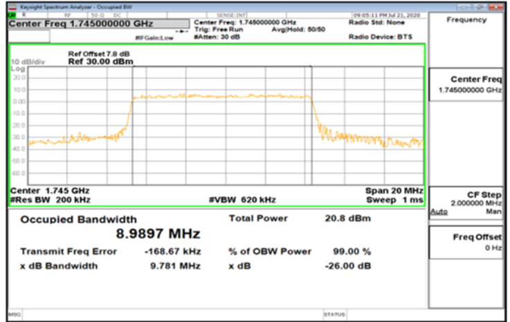
DFT-s-OFDM_Band66_10MHz_64QAM_50_0_Main_MidCH349000
