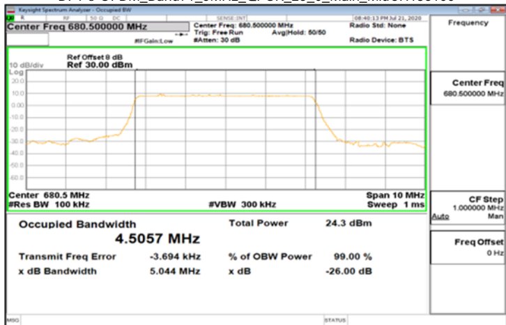
DFT-s-OFDM_Band71_5MHz_QPSK_25_0_Main_MidCH136100
