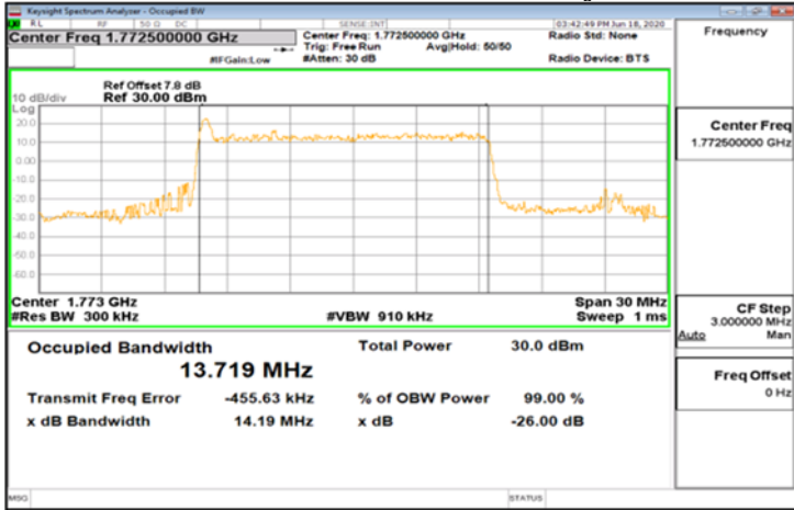
DFT-s-OFDM Pi/2_Band66_15MHz_BPSK_75_0_Main_HighCH354500-1772.5
