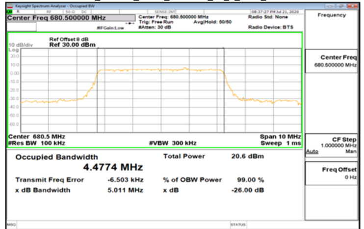
DFT-s-OFDM_Band71_5MHz_256QAM_25_0_Main_MidCH136100
