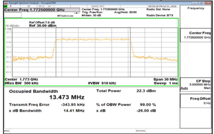
DFT-s-OFDM_Band66_15MHz_QPSK_75_0_Main_HighCH354500
