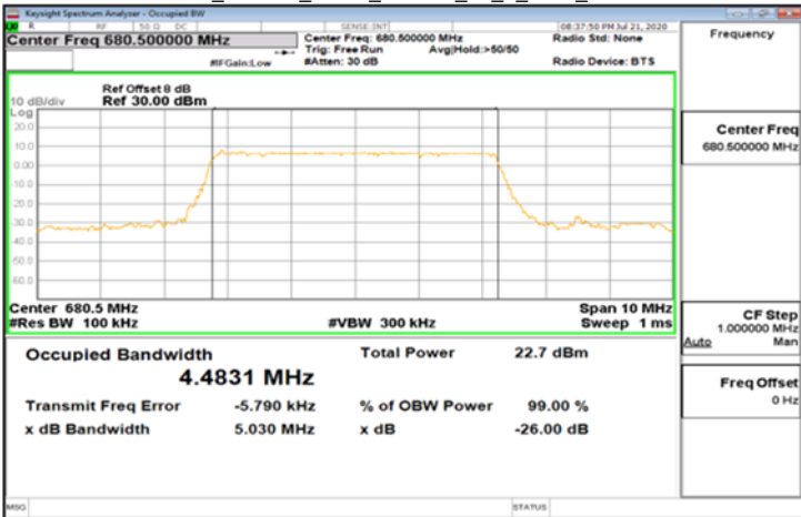
DFT-s-OFDM_Band71_5MHz_64QAM_25_0_Main_MidCH136100
