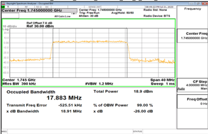
DFT-s-OFDM_Band66_20MHz_256QAM_100_0_Main_MidCH349000
