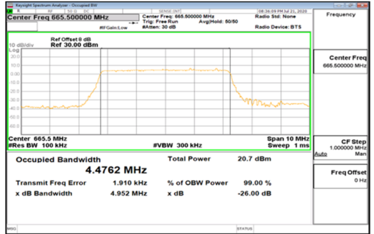
DFT-s-OFDM_Band71_5MHz_256QAM_25_0_Main_MidCH136100
