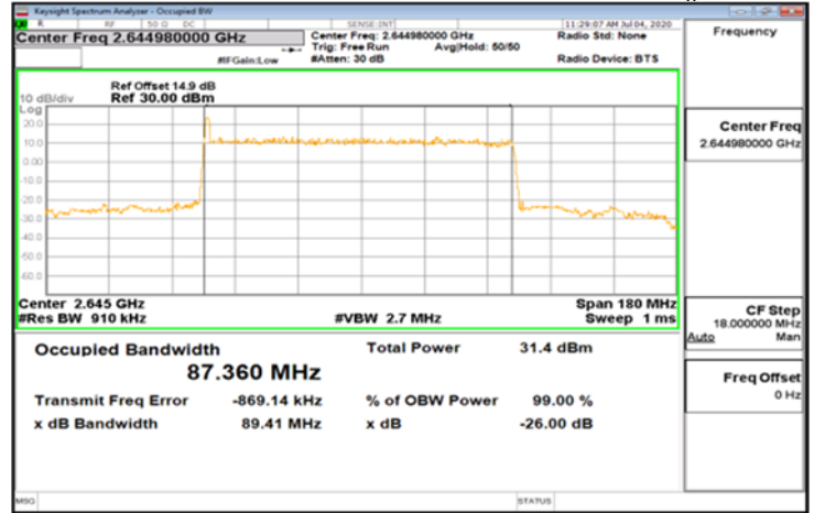
DFT-s-OFDM Pi/2_Band41_90MHz_BPSK_243_0_Main_High
