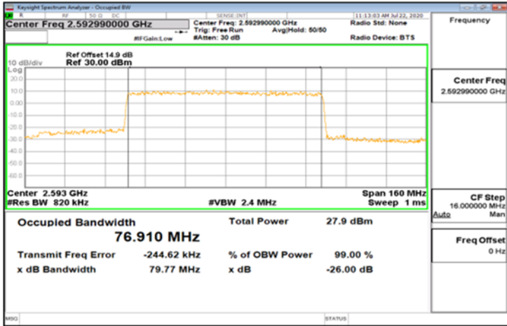
DFT-s-OFDM_Band41_80MHz_256QAM_216_0_Main_MidCH518598
