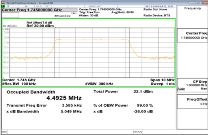
DFT-s-OFDM_Band66_5MHz_64QAM_25_0_Main_MidCH349000
