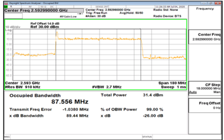
DFT-s-OFDM Pi/2_Band41_90MHz_BPSK_243_0_Main_MidCH518598-2592.99
