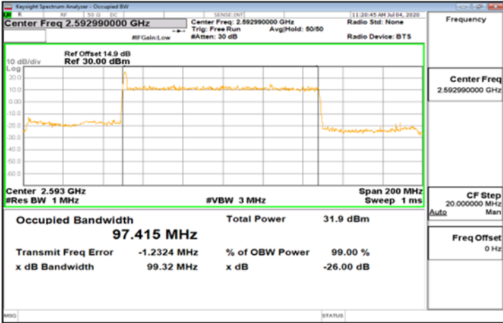
DFT-s-OFDM Pi/2_Band41_100MHz_BPSK_270_0_Main_MidCH518598-2592.99
