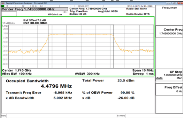
DFT-s-OFDM_Band66_5MHz_QPSK_25_0_Main_MidCH349000
