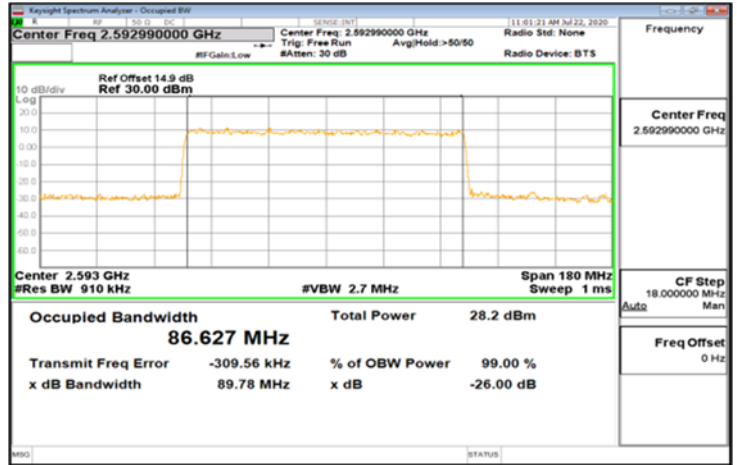
DFT-s-OFDM_Band41_90MHz_256QAM_243_0_Main_HighCH528996
