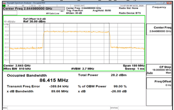
DFT-s-OFDM_Band41_90MHz_256QAM_243_0_Main_HighCH528996
