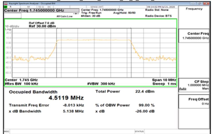
DFT-s-OFDM_Band66_5MHz_16QAM_25_0_Main_MidCH349000
