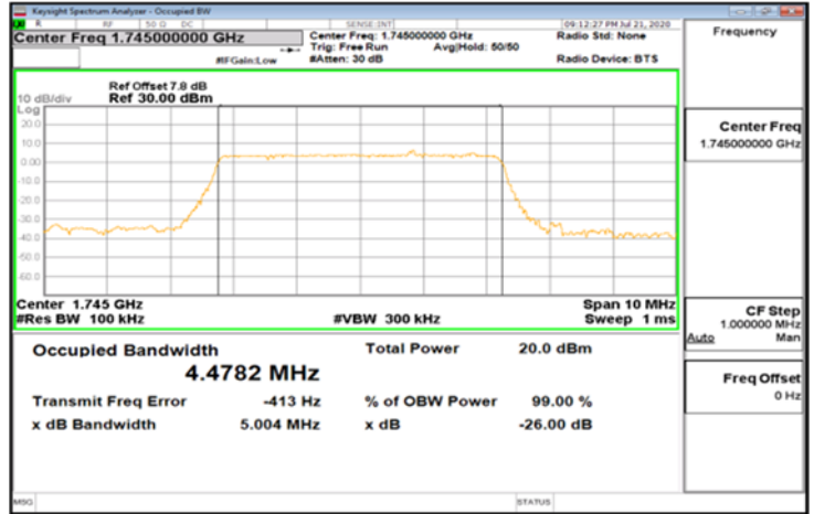
DFT-s-OFDM_Band66_5MHz_256QAM_25_0_Main_MidCH349000
