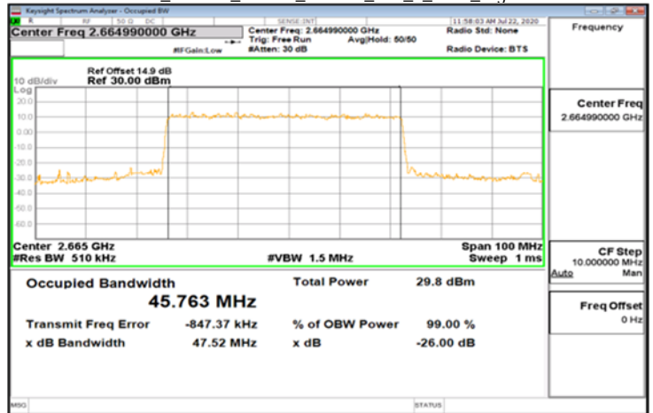
DFT-s-OFDM_Band41_50MHz_64QAM_128_0_Main_HighCH532998
