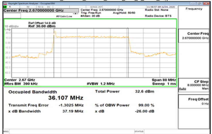
DFT-s-OFDM Pi/2_Band41_40MHz_BPSK_100_0_Main_HighCH534000
