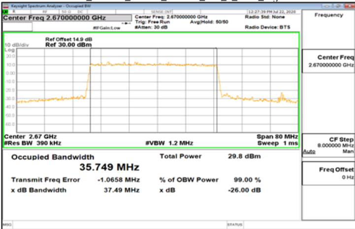
DFT-s-OFDM_Band41_40MHz_64QAM_100_0_Main_HighCH534000
