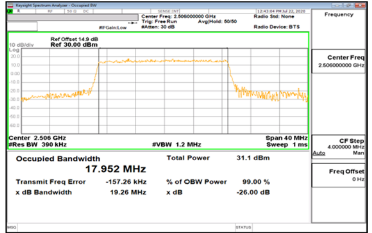
DFT-s-OFDM_Band41_20MHz_QPSK_50_0_Main_MidCH40620
