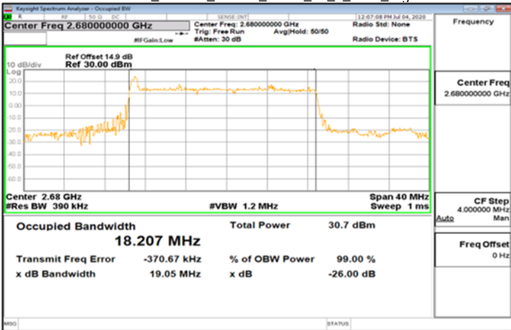
DFT-s-OFDM Pi/2_Band41_20MHz_BPSK_50_0_Main_HighCH41490
