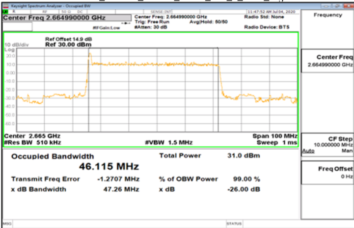
DFT-s-OFDM Pi/2_Band41_50MHz_BPSK_128_0_Main_HighCH532998
