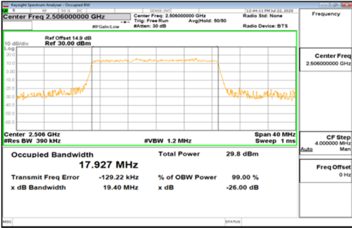
DFT-s-OFDM_Band41_20MHz_256QAM_50_0_Main_MidCH40620
