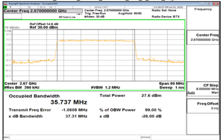
DFT-s-OFDM_Band41_40MHz_256QAM_100_0_Main_HighCH534000
