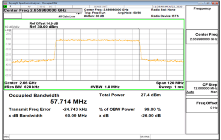
DFT-s-OFDM_Band41_60MHz_256QAM_162_0_Main_HighCH534996
