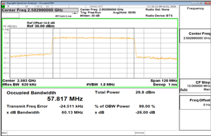
DFT-s-OFDM_Band41_60MHz_64QAM_162_0_Main_MidCH518598
