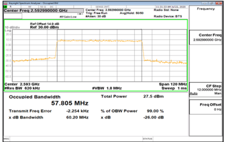
DFT-s-OFDM_Band41_60MHz_256QAM_162_0_Main_MidCH518598
