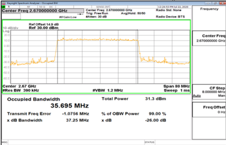
DFT-s-OFDM_Band41_40MHz_QPSK_100_0_Main_HighCH534000
