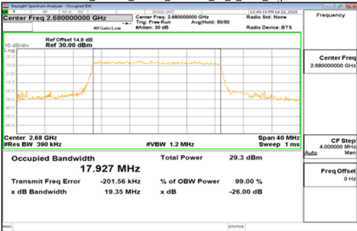
DFT-s-OFDM_Band41_20MHz_256QAM_50_0_Main_HighCH41490
