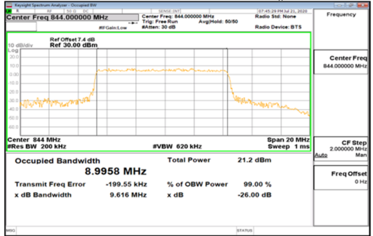
DFT-s-OFDM_Band5_10MHz_16QAM_50_0_Main_HighCH168800
