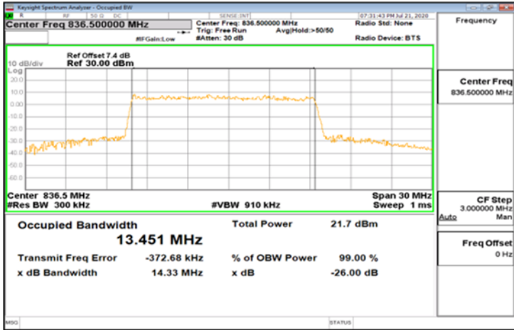
DFT-s-OFDM_Band5_15MHz_16QAM_75_0_Main_MidCH167300
