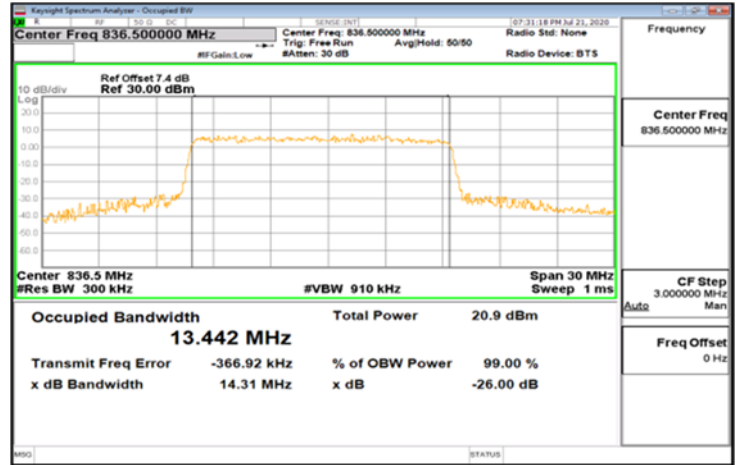
DFT-s-OFDM_Band5_15MHz_64QAM_75_0_Main_MidCH167300
