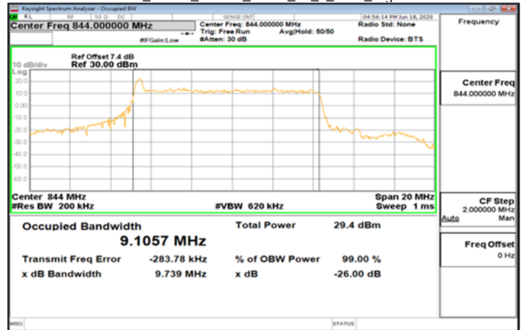
DFT-s-OFDM Pi/2_Band5_10MHz_BPSK_50_0_Main_HighCH168800-844
