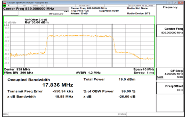
DFT-s-OFDM_Band5_20MHz_256QAM_100_0_Main_HighCH167800
