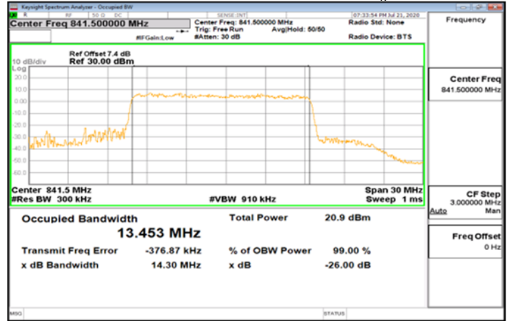
DFT-s-OFDM_Band5_15MHz_64QAM_75_0_Main_HighCH168300
