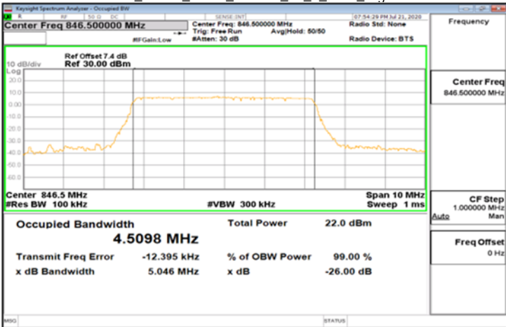
DFT-s-OFDM_Band5_5MHz_16QAM_25_0_Main_HighCH169300
