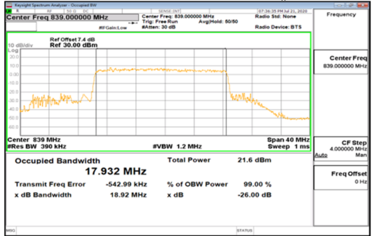
DFT-s-OFDM_Band5_20MHz_16QAM_100_0_Main_HighCH167800
