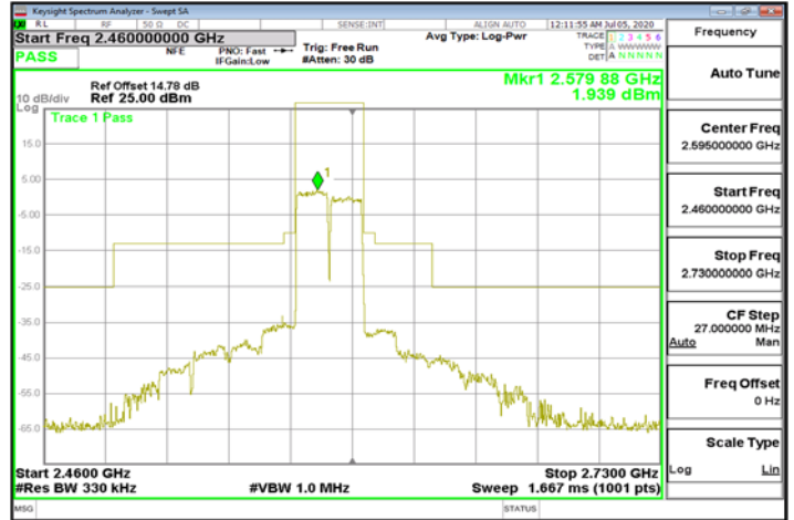
Mask_LTE\Band38_30MHzQPSK_1_0_1_74_CH_High_2605
