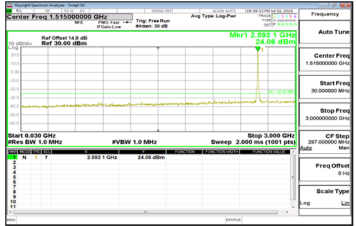
Emission_Band41_40MHz_OPSK_1_99_1_0_30MHz-3GHz_CH_High 2670
