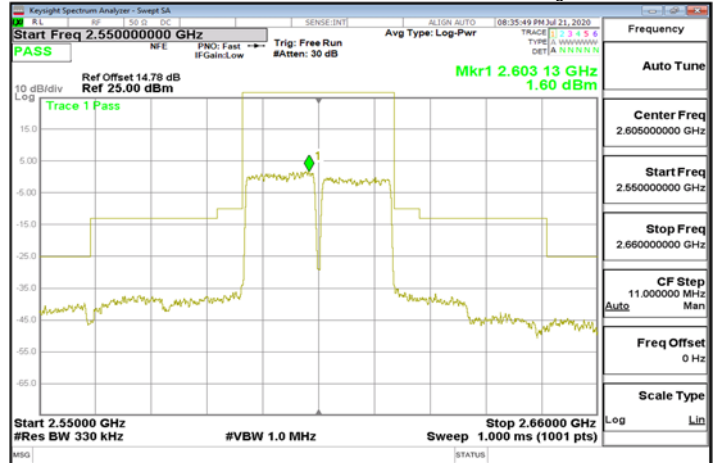
Mask_LTE\Band38_30MHzQPSK_75_0_75_0_CH_High_2605
