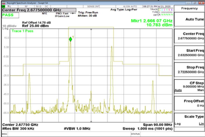
Mask_LTE\Band41_25MHz\QPSK_100_0_25_0_CH_High2677.5
