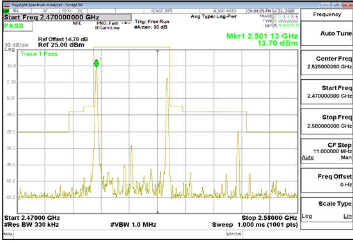
Mask_LTE\Band7_30MHz\QPSK_100_0_50_0_CH_Low 2515
