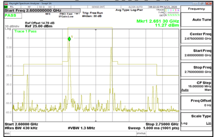
Mask_LTE\Band41_40MHz\QPSK_100_0_100_0_CH_High2670
