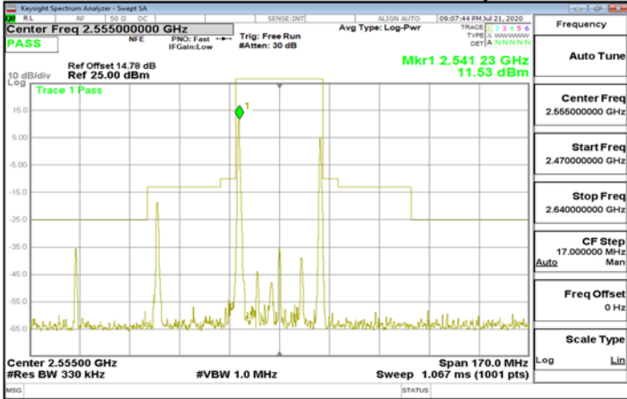
Mask_LTE\Band7_30MHz\QPSK_1_0_1_49_CH_High 2555
