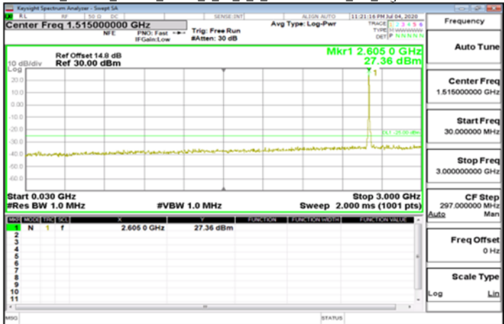
Emission_Band38_30MHz_QPSK_1_74_1_0_30MHz-3GHz_CH_HighCH38150-2610
