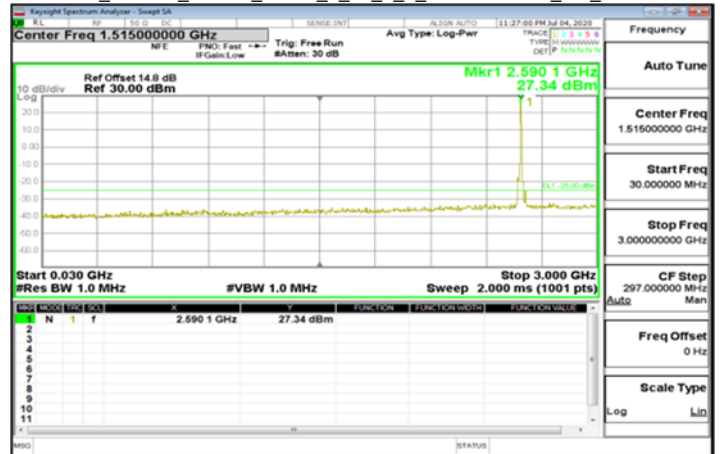
Emission_Band38_40MHz_QPSK_1_99_1_0_30MHz-3GHz_CH_Mid 2595
