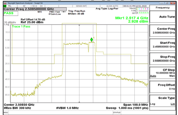
Mask_LTE\Band41_25MHz\QPSK_100_0_25_0_CH_Low 2508.5
