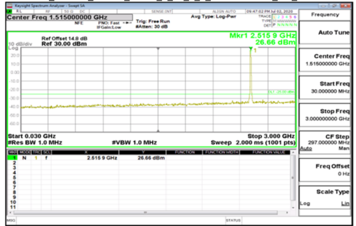
Emission_Band41_40MHz_OPSK_1_99_1_0_30MHz-3GHz_CH_Mid 2593
