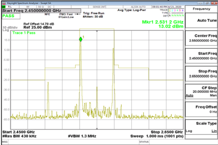
Mask_LTE\Band7_40MHzQPSK_100_0_100_0_CH_High_2550
