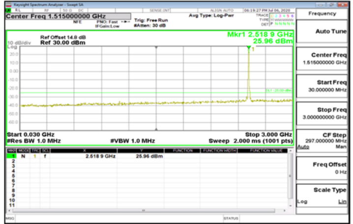
Emission_Band7_40MHz_QPSK_1_99_1_0_30MHz-3GHz_CH_Mid2535
