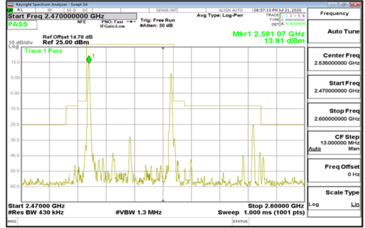
Mask_LTE\Band7_40MHz\QPSK_100_0_100_0_CH_Low 2520
