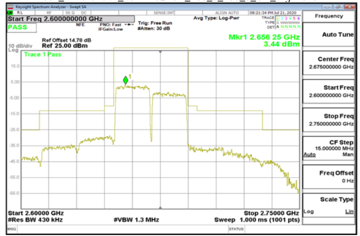
Mask_LTE\Band41_40MHz\QPSK_100_0_100_0_CH_High2670
