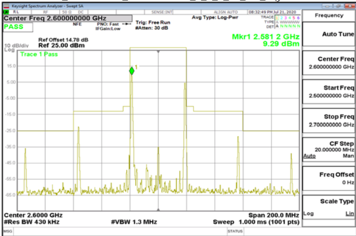
Mask_LTE\Band38_40MHz\QPSK_1_0_1_99_CH_High 2600
