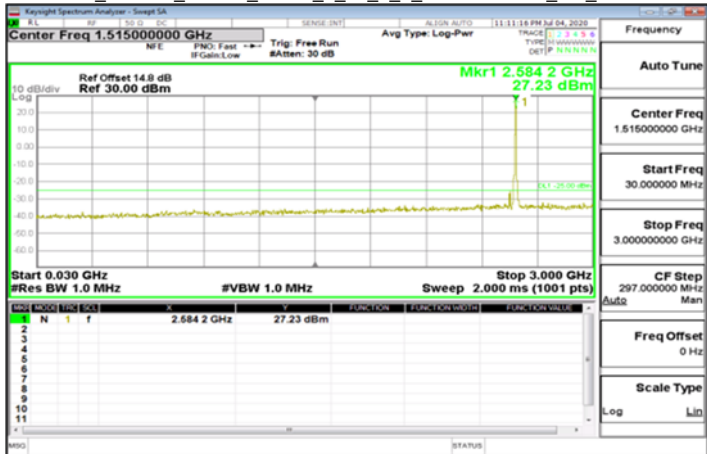
Emission_Band38_30MHz_QPSK_1_74_1_0_30MHz-3GHz_CH_Mid 2595
