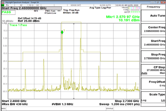
Mask_LTE\Band38_40MHz\QPSK_100_0_100_0_CH_Low 2590
