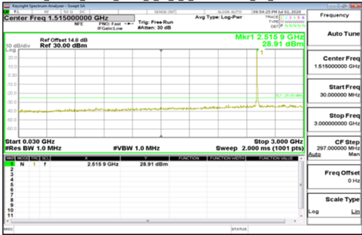
Emission_Band41_25MHz_OPSK_1_99_1_0_30MHz-3GHz_CH_Mid2593
