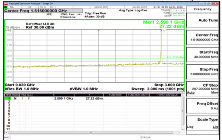
Emission_Band38_40MHz_QPSK_1_99_1_0_30MHz-3GHz_CH_High 2600
