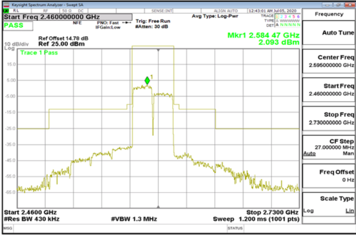
Mask_LTE\Band38_40MHz\QPSK_1_0_1_99_CH_High 2600
