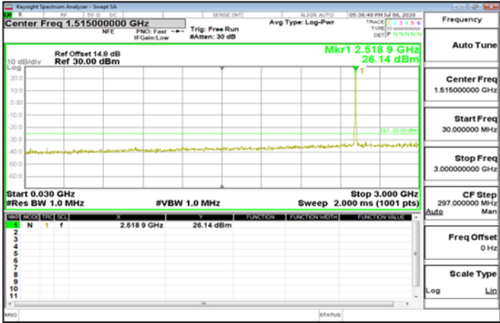
Emission_Band7_30MHz_QPSK_1_99_1_0_30MHz-3GHz_CH_Mid2535
