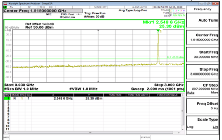
Emission_Band7_40MHz_QPSK_1_99_1_0_30MHz-3GHz_CH_High2550
