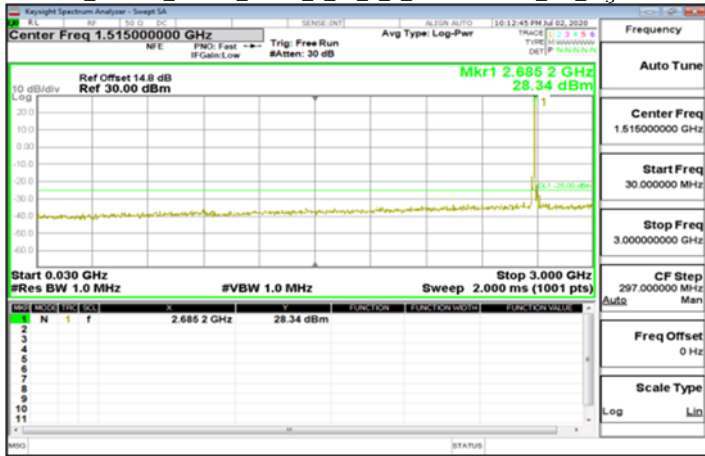
Emission_Band41_25MHz_OPSK_1_99_1_0_30MHz-3GHz_CH_High 2677.5
