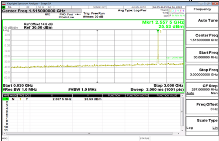
Emission_Band7_30MHz_QPSK_1_99_1_0_30MHz-3GHz_CH_High2555
