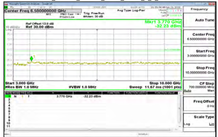
3GHz~10GHz_Band26_Part90s_5MHz_QPSK_1_0_MidCH26740-819
