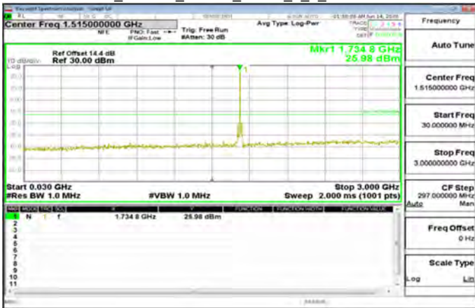
30MHz~3GHz_Band66_20MHz_QPSK_1_0_MidCH132322-1745
