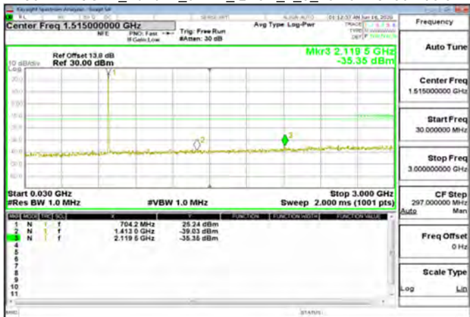
30MHz-3GHz_Band17_5MHz_QPSK_1_0_LowCH23755-706.5
