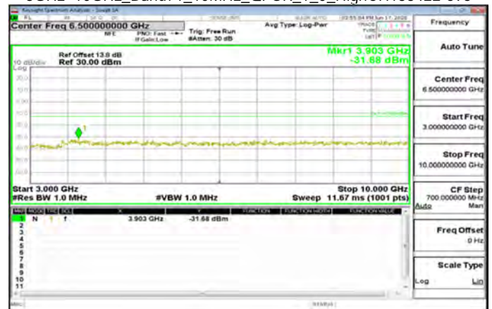
3GHz~10GHz_Band71_10MHz_QPSK_1_0_HighCH133422-693
