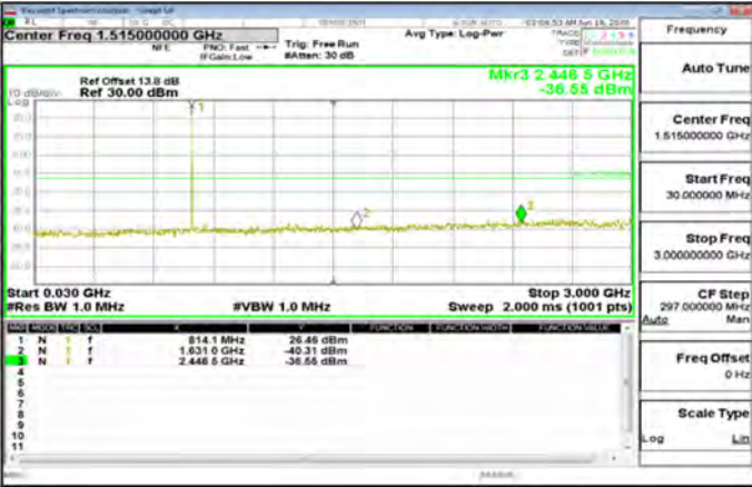
30MHz-3GHz_Band26_Part90s_3MHz_QPSK_1_0_LowCH26705-815.5
