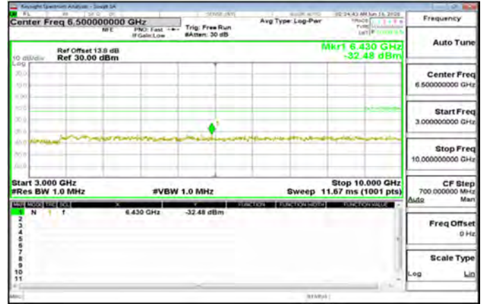
3GHz-10GHz_Band26_Part90s_1_4MHz_QPSK_1_0_MidCH26740-819
