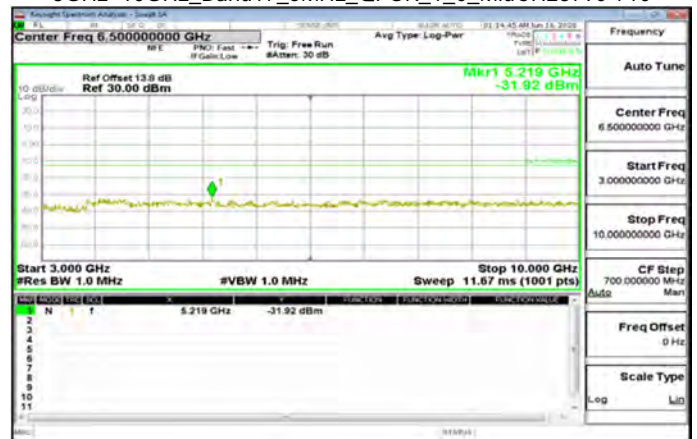
3GHz-10GHz_Band17_5MHz_QPSK_1_0_MidCH23790-710
