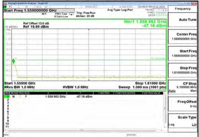
GPS_Band13_5MHz_QPSK_1_0_MidCH23230-782
