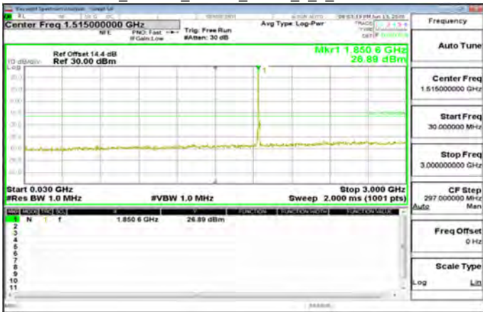
30MHz-3GHz_Band25_10MHz_QPSK_1_0_LowCH26090-1855
