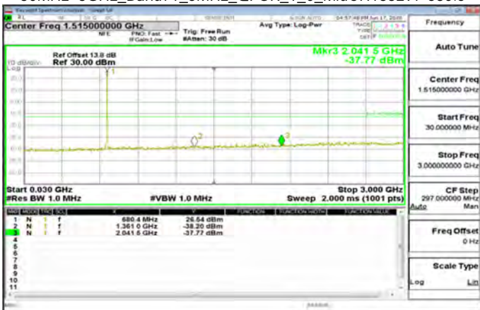
30MHz-3GHz_Band71_5MHz_QPSK_1_0_MidCH133297-680.5
