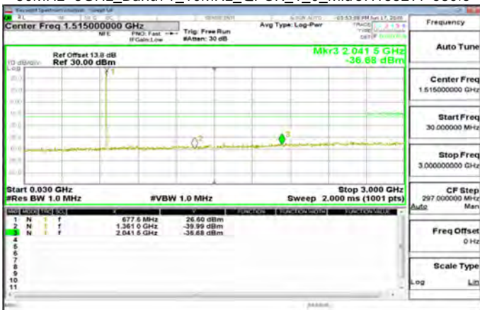
30MHz~3GHz_Band71_10MHz_QPSK_1_0_MidCH133297-680.5
