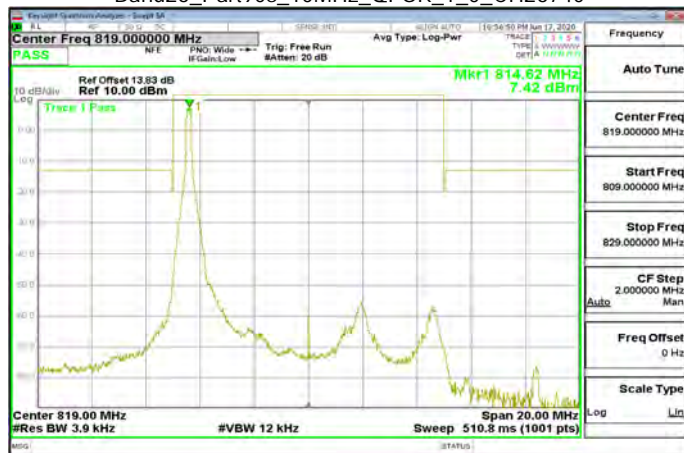
Band26_Part90s_10MHz_QPSK_1_0_CH26740
