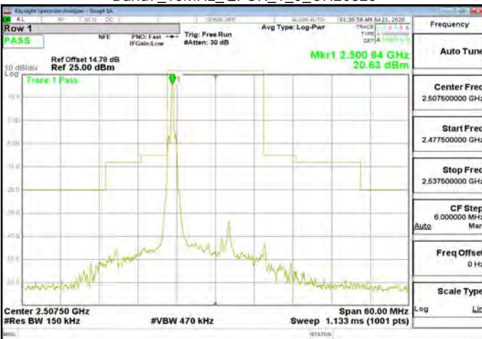
Band7_15MHz_QPSK_1_0_CH20825
