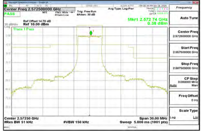
Band38_5MHz_QPSK_25_0_CH37775
