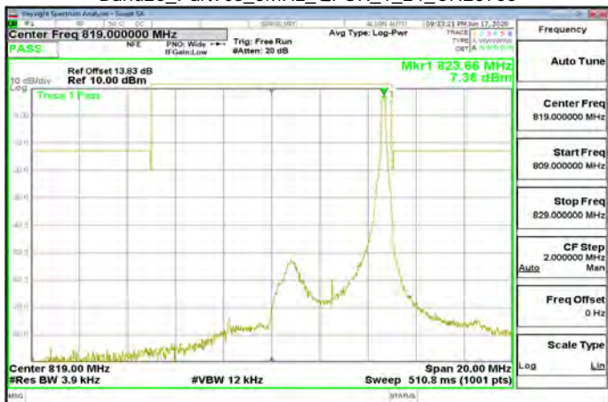
Band26_Part90s_5MHz_QPSK_1_24_CH26765
