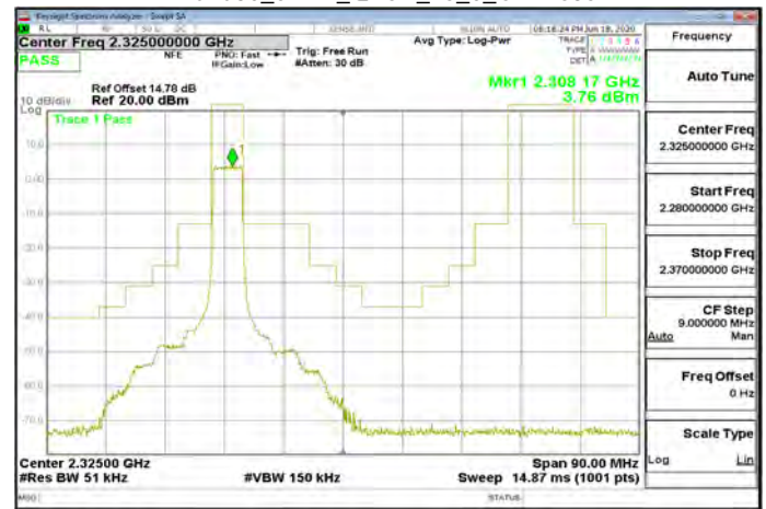
Band30_5MHz_QPSK_25_0_CH27735
