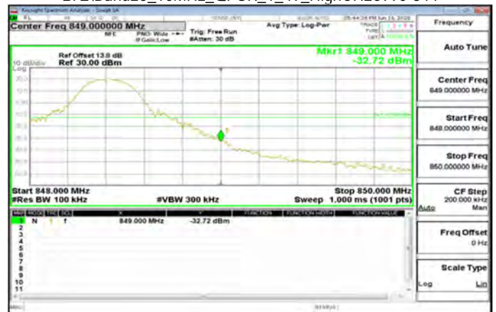
LTE\Band26_10MHz_QPSK_1_49_HighCH26990-844
