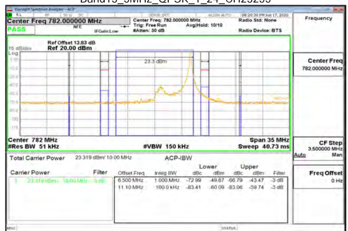
Band13_5MHz_QPSK_1_24_CH23255
