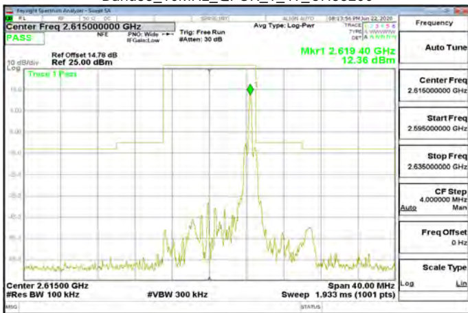
Band38_10MHz_QPSK_1_49_CH38200
