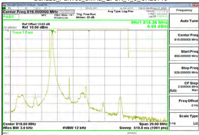
Band26_Part90s_5MHz_QPSK_1_24_CH26765
