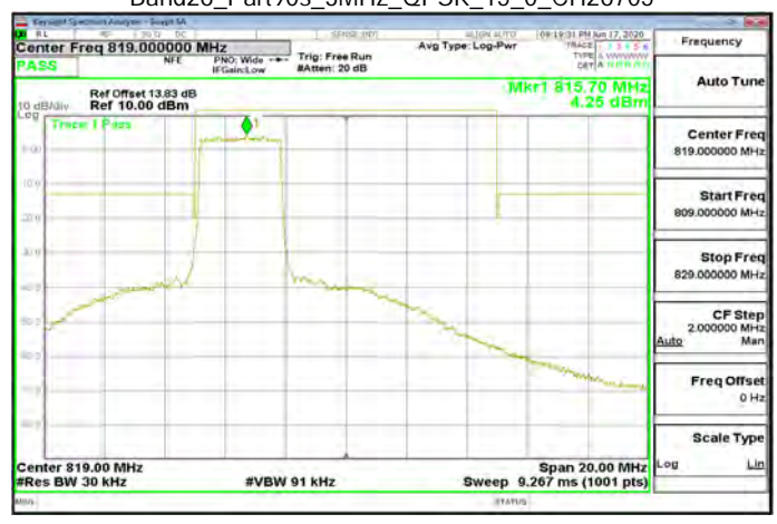
Band26_Part90s_3MHz_QPSK_15_0_CH26705
