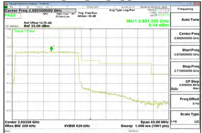
Band41_20MHz_QPSK_100_0_CH41490
