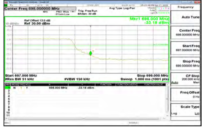
LTE\Band71_5MHz_QPSK_25_0_HighCH133447-695.5
