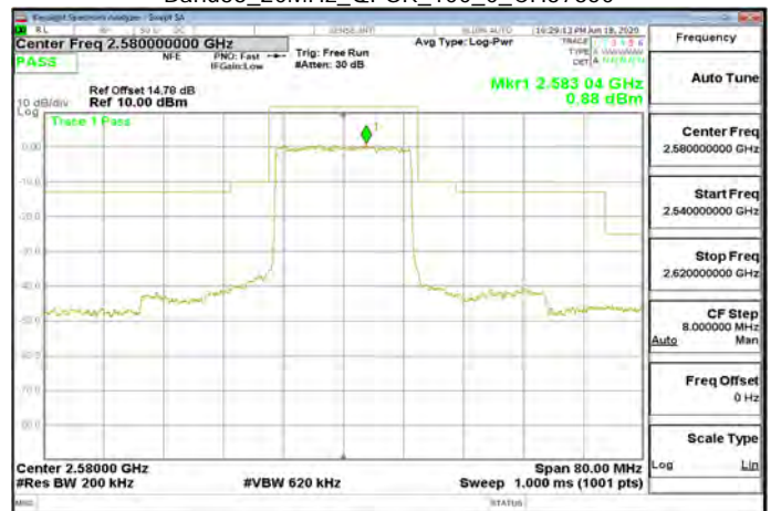
Band38_20MHz_QPSK_100_0_CH37850
