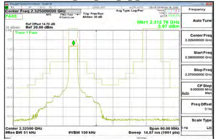
Band30_5MHz_QPSK_25_0_CH27735
