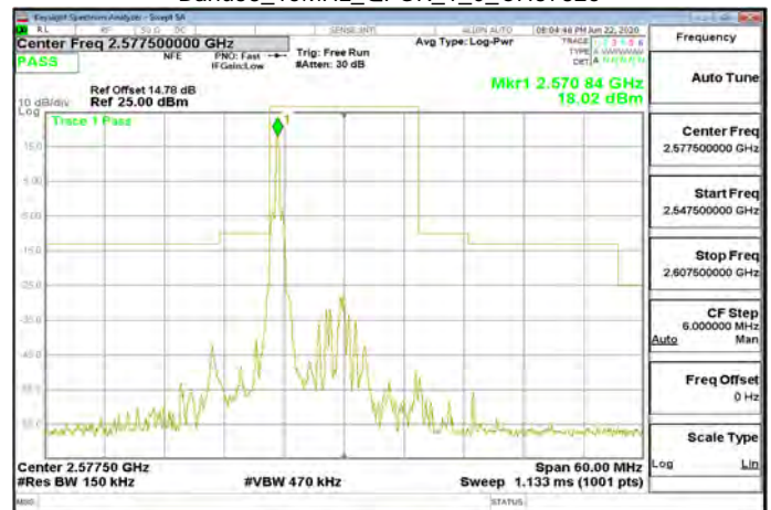
Band38_15MHz_QPSK_1_0_CH37825
