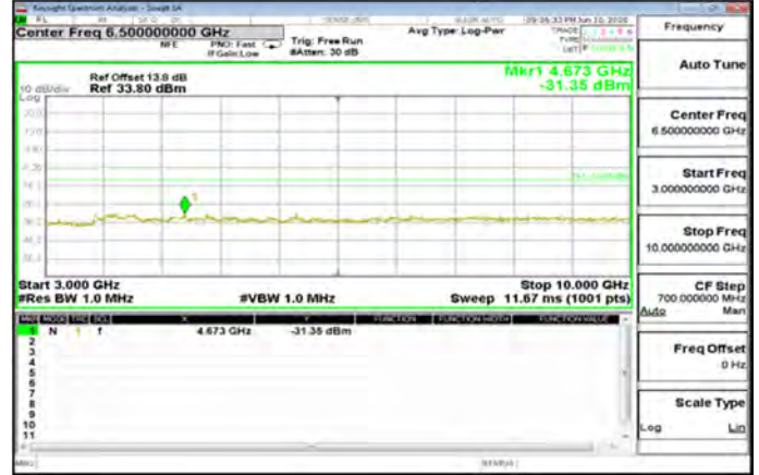
3GHz-10GHz_GSM_850MHz_HighCH251-848.8
