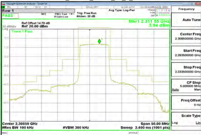
Band30_10MHz_QPSK_50_0_CH27710
