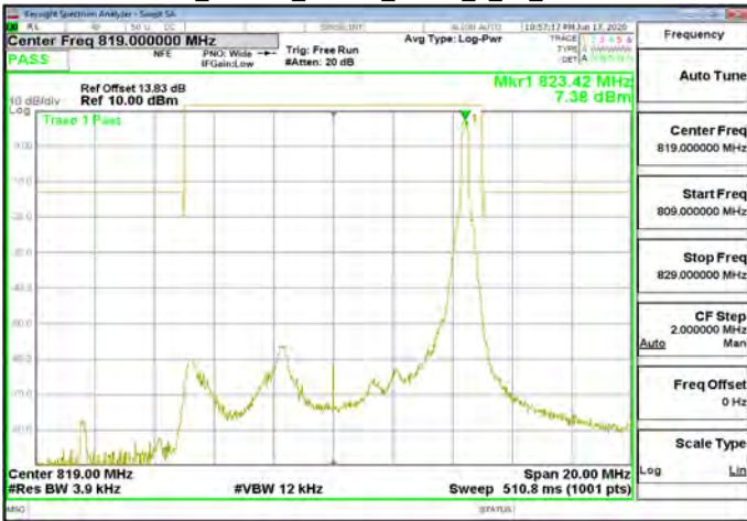
Band26_Part90s_10MHz_QPSK_50_0_CH26740
