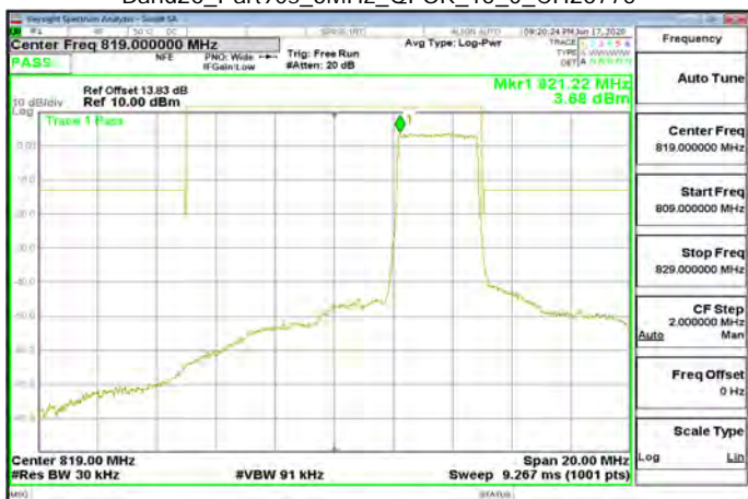
Band26_Part90s_5MHz_QPSK_1_0_CH26715
