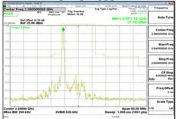
Band38_20MHz_QPSK_1_99_CH38150
