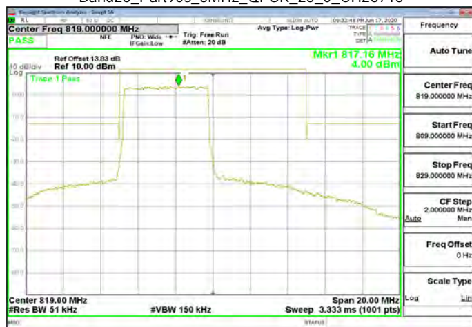
Band26_Part90s_5MHz_QPSK_25_0_CH26765
