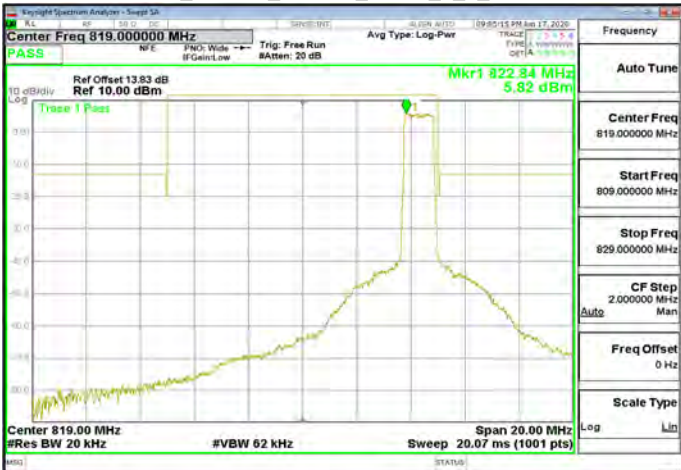
Band26_Part90s_1.4MHz_QPSK_6_0_CH26783
