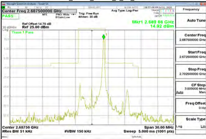
Band41_5MHz_QPSK_1_24_CH41565
