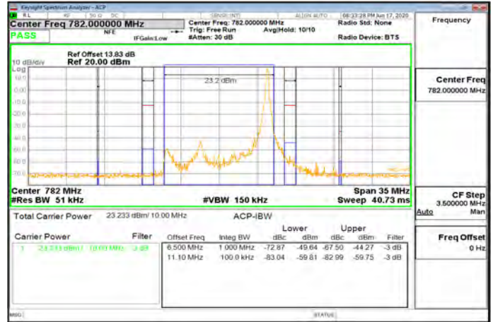
Band13_10MHz_QPSK_50_0_CH23230
