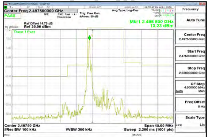
Band41_10MHz_QPSK_1_0_CH39700
