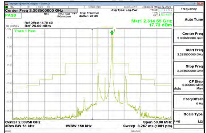
Band30_5MHz_QPSK_25_0_CH27685
