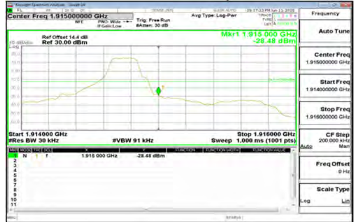
LTE\Band25_1_4MHz_QPSK_1_5_HighCH26683-1914.3
