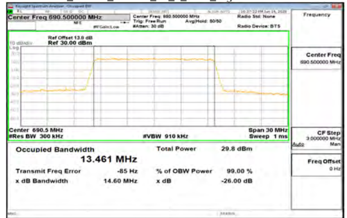
Band71_15MHz_16QAM_75_0_Main_HighCH133397-690.5
