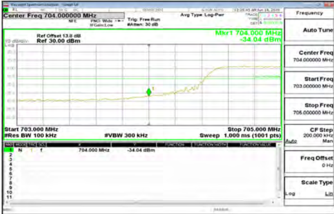
LTE\Band17_10MHz_QPSK_50_0_LowCH23780-709
