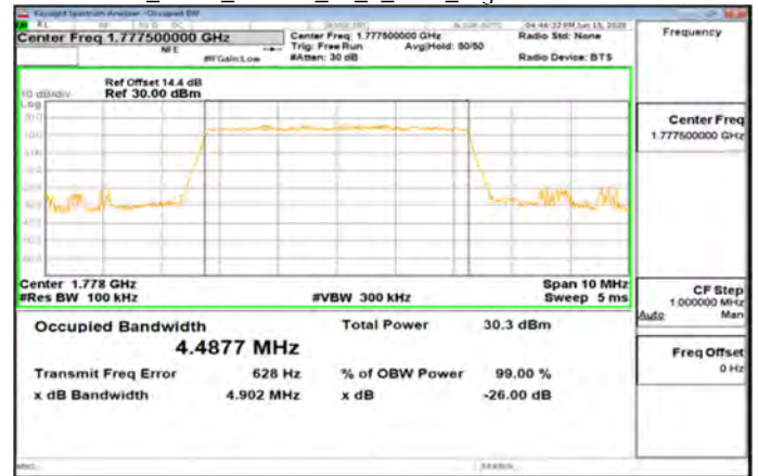
Band66_5MHz_16QAM_25_0_Main_HighCH132647-1777.5
