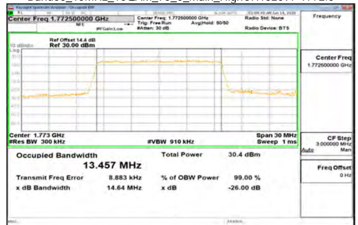
Band66_15MHz_16QAM_75_0_Main_HighCH132597-1772.5
