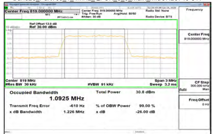
Band26_Part90s_1_4MHz_QPSK_6_0_Main_MidCH26740-819
