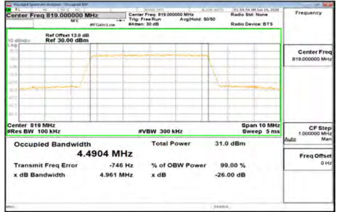
Band26_Part90s_5MHz_QPSK_25_0_Main_MidCH26740-819
