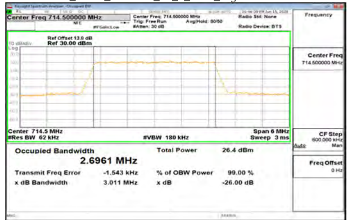
Band12_3MHz_256QAM_15_0_Main_HighCH23165-714.5
