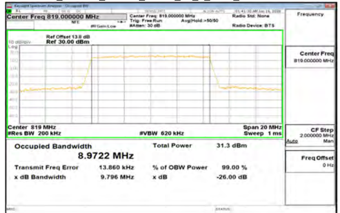
Band26_Part90s_10MHz_16QAM_50_0_Main_MidCH26740-819
