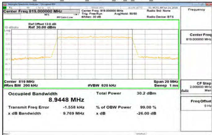
Band26_Part90s_10MHz_256QAM_50_0_Main_MidCH26740-819
