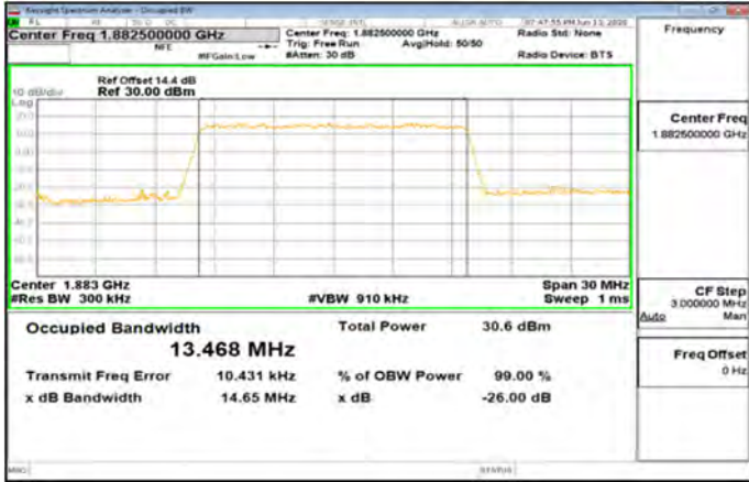
Band25_15MHz_16QAM_75_0_Main_MidCH26365-1882.5
