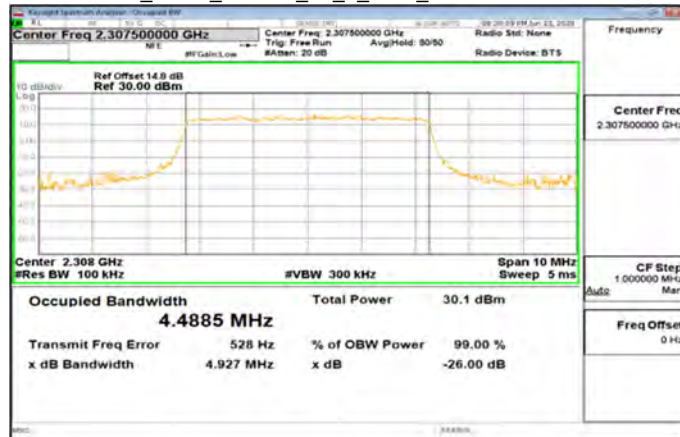
Band30_5MHz_16QAM_25_0_Main_LowCH27685-2307.5
