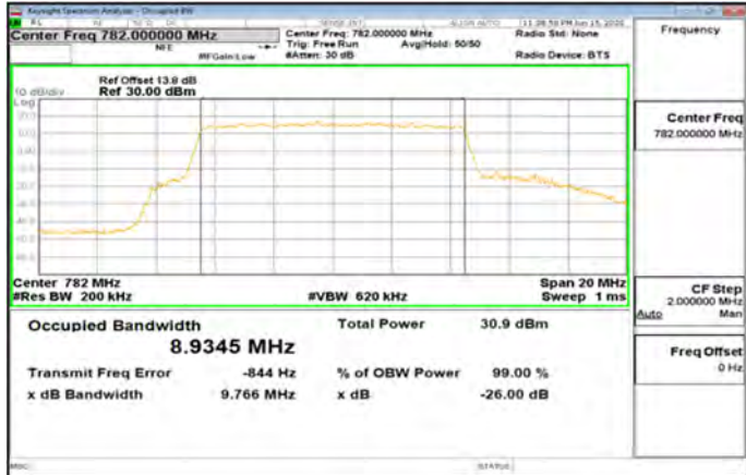
Band13_10MHz_64QAM_50_0_Main_MidCH23230-782
