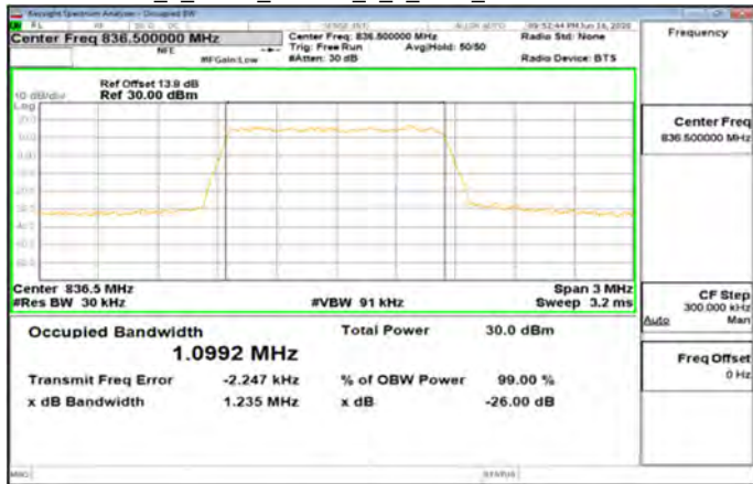
Band26_1_4MHz_16QAM_6_0_Main_MidCH26915-836.5
