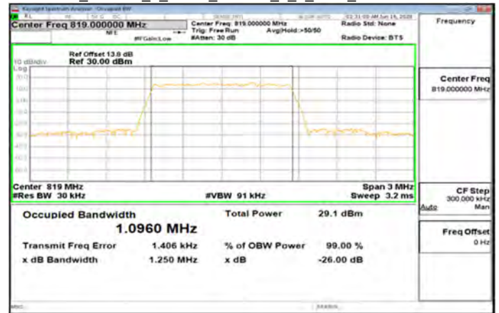
Band26_Part90s_1_4MHz_64QAM_6_0_Main_MidCH26740-819
