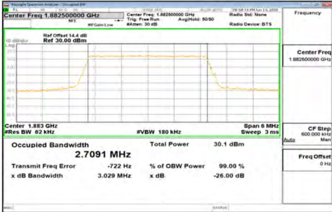
Band25_3MHz_16QAM_15_0_Main_MidCH26365-1882.5
