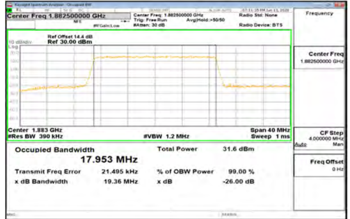
Band25_20MHz_QPSK_100_0_Main_MidCH26365-1882.5
