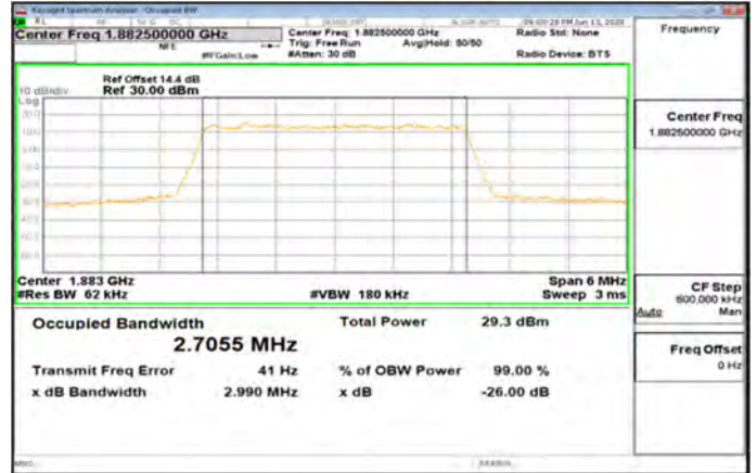
Band25_3MHz_64QAM_15_0_Main_MidCH26365-1882.5
