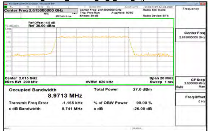
Band38_10MHz_256QAM_50_0_Main_HighCH38200-2615
