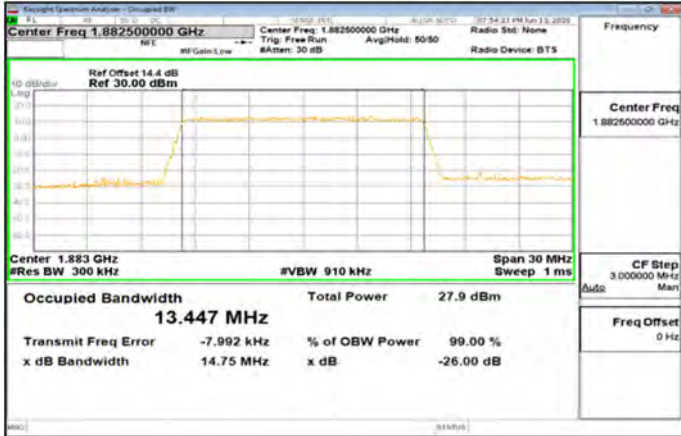
Band25_15MHz_256QAM_75_0_Main_MidCH26365-1882.5
