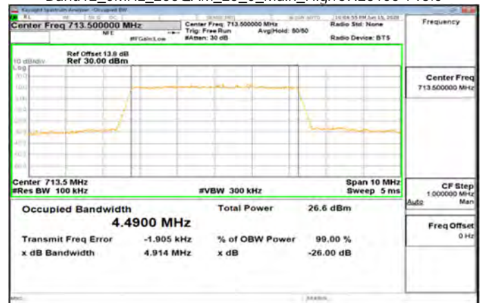
Band12_5MHz_256QAM_25_0_Main_HighCH23155-713.5
