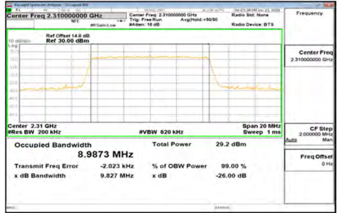
Band30_10MHz_256QAM_50_0_Main_MidCH27710-2310
