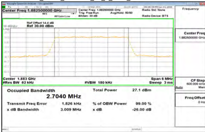
Band25_3MHz_256QAM_15_0_Main_MidCH26365-1882.5
