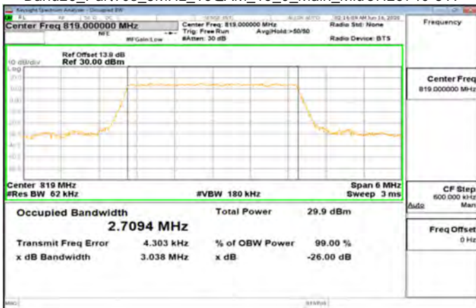
Band26_Part90s_3MHz_16QAM_15_0_Main_MidCH26740-819
