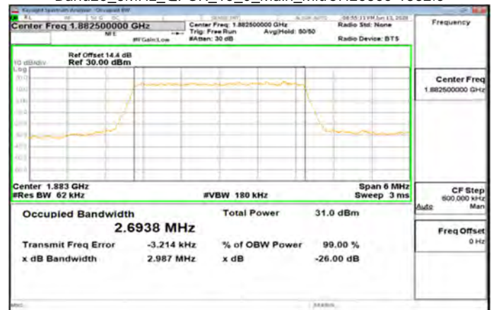
Band25_3MHz_QPSK_15_0_Main_MidCH26365-1882.5
