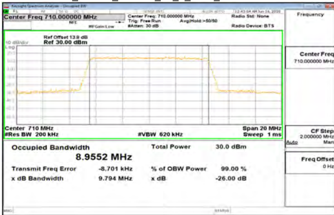
Band17_10MHz_16QAM_50_0_Main_MidCH23790-710
