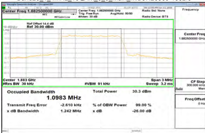
Band25_1_4MHz_16QAM_6_0_Main_MidCH26365-1882.5
