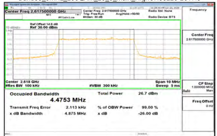
Band38_5MHz_256QAM_25_0_Main_HighCH38225-2617.5
