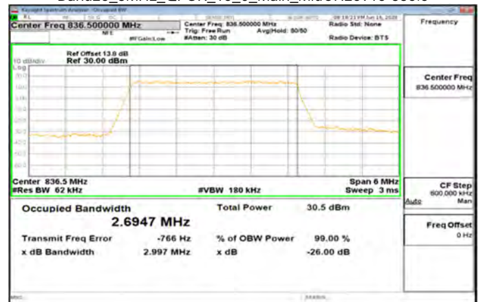
Band26_3MHz_QPSK_15_0_Main_MidCH26915-836.5
