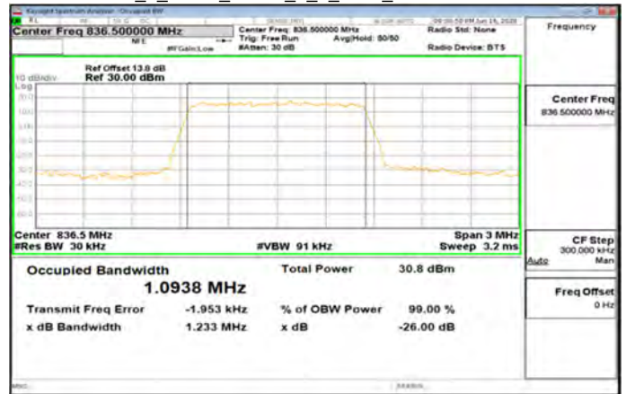
Band26_1_4MHz_QPSK_6_0_Main_MidCH26915-836.5
