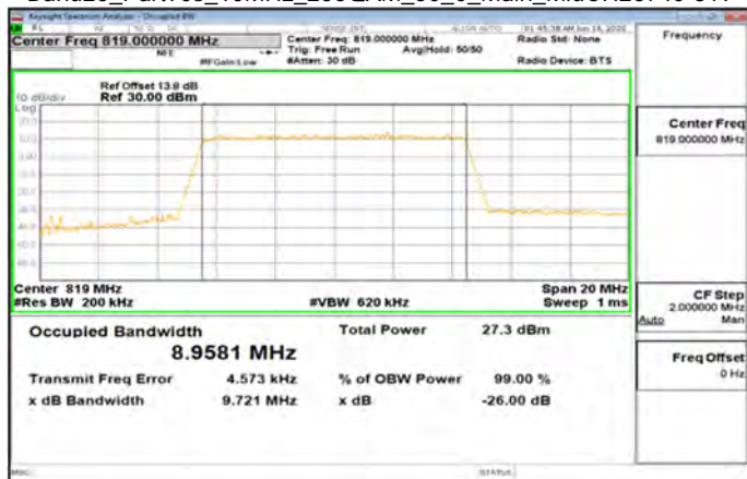
Band26_Part90s_10MHz_256QAM_50_0_Main_MidCH26740-819
