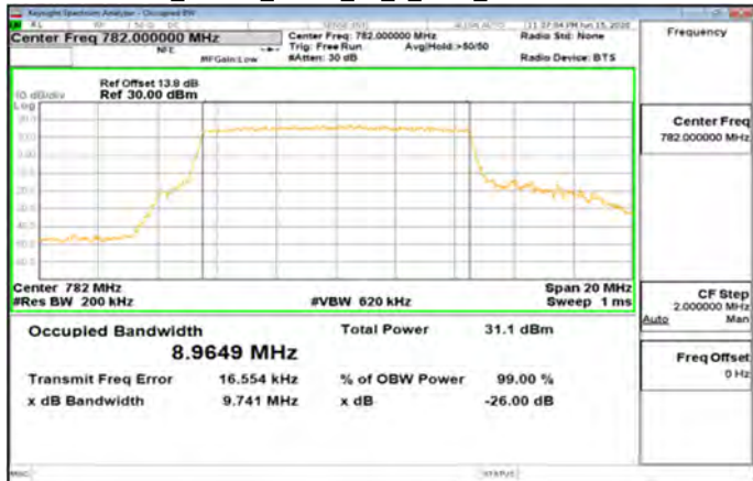
Band13_10MHz_16QAM_50_0_Main_MidCH23230-782
