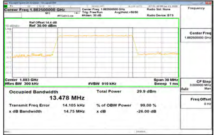
Band25_15MHz_64QAM_75_0_Main_MidCH26365-1882.5
