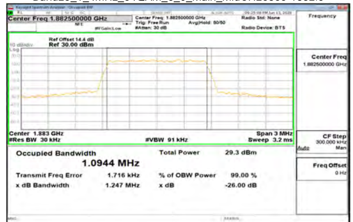
Band25_1_4MHz_64QAM_6_0_Main_MidCH26365-1882.5
