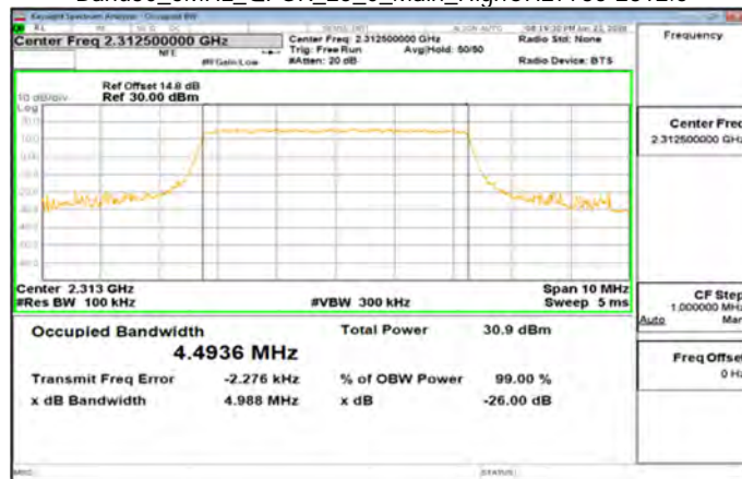
Band30_5MHz_QPSK_25_0_Main_HighCH27735-2312.5
