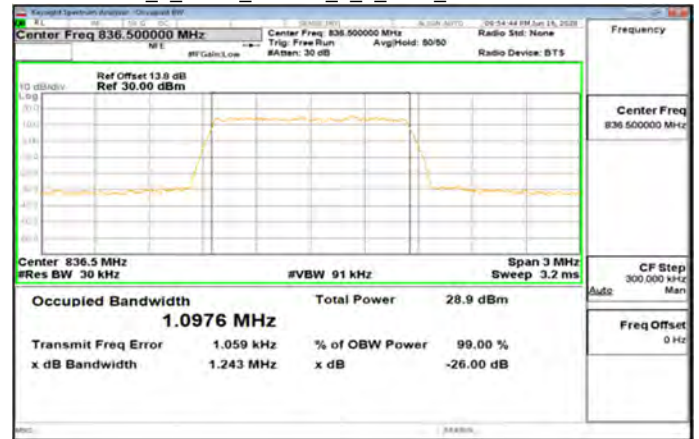
Band26_1_4MHz_64QAM_6_0_Main_MidCH26915-836.5
