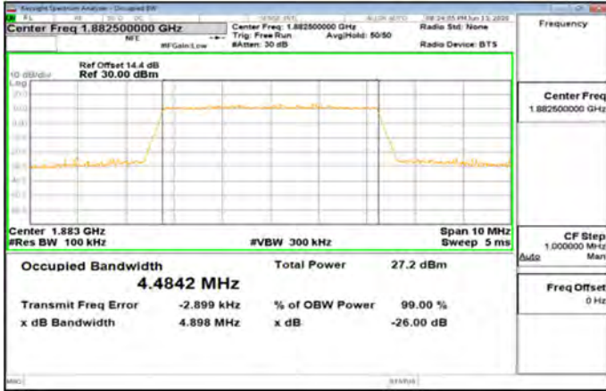
Band25_5MHz_256QAM_25_0_Main_MidCH26365-1882.5
