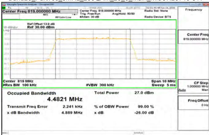
Band26_Part90s_5MHz_256QAM_25_0_Main_MidCH26740-819
