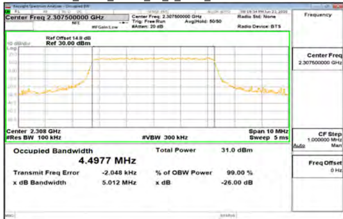
Band30_5MHz_QPSK_25_0_Main_LowCH27685-2307.5
