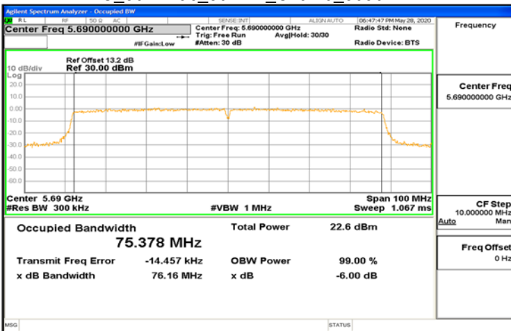
IC_802.11ac_80MHz_Chain0_5690MHz
