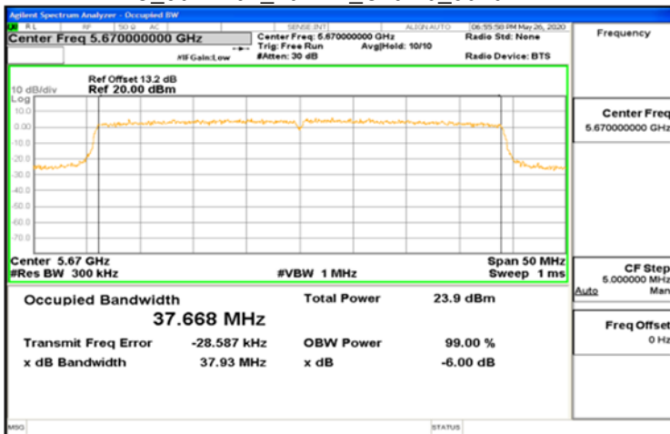
IC_802.11ax_40MHz_Chain0_5670MHz
