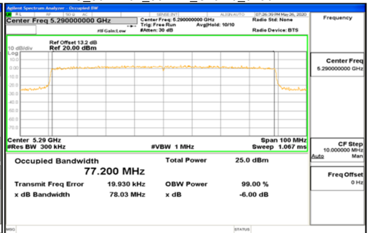
IC_802.11ax_80MHz_Chain0_5290MHz
