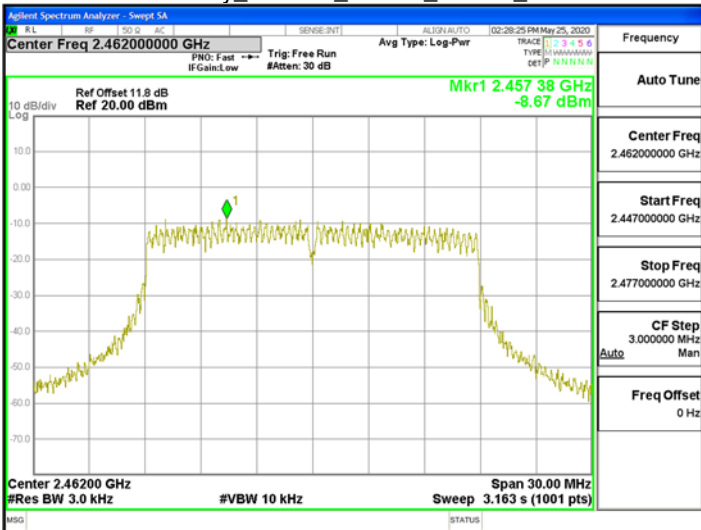
Power Density_802.11n_20MHz_Chain0_2462MHz
