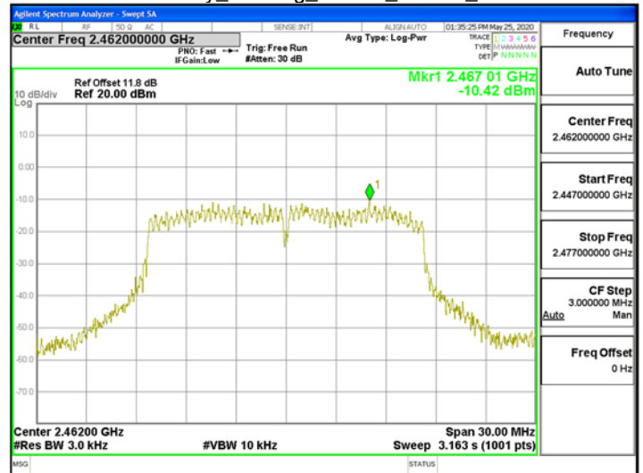
Power Density_802.11g_20MHz_Chain1_2462MHz
