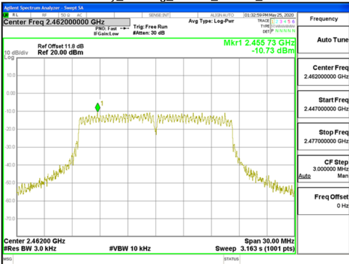
Power Density_802.11g_20MHz_Chain0_2462MHz
