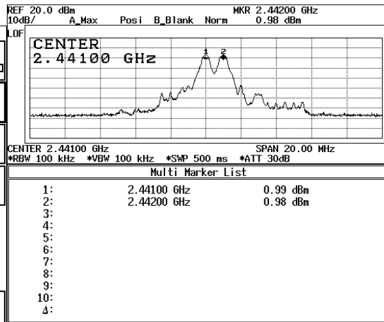
Channel 39 2441MHz
