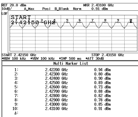
2422-2431MHz
