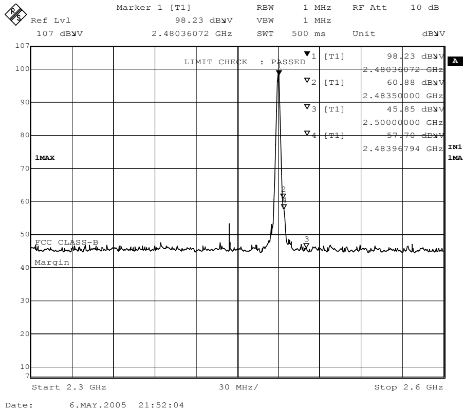
Figure Channel 78: (Horizontal)
