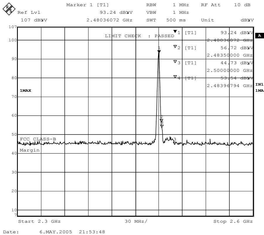
Figure Channel 78: (Vertical)
