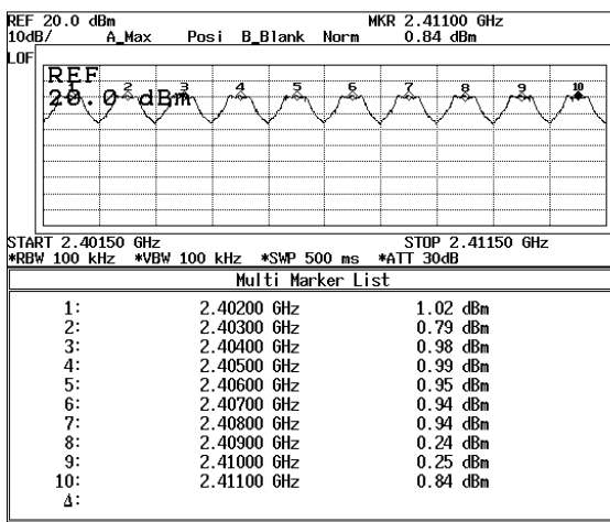
2402-2411MHz
