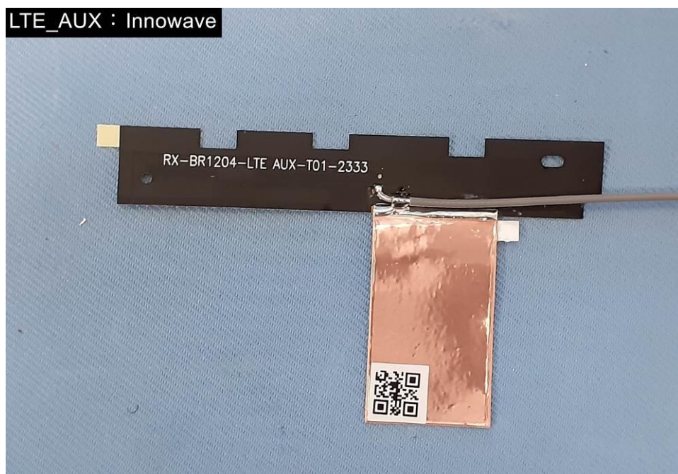
EUT Photo (42)
