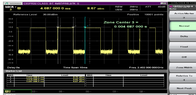
Time-domain Plot for Bluetooth Antenna-1 Transmission
