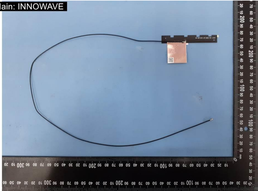
EUT Photo (42) WWAN antenna Main : INNOWAVE
