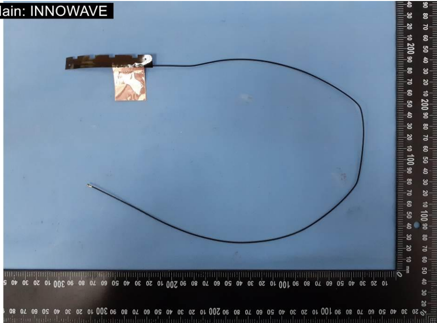
EUT Photo (44) WWAN antenna Main : INNOWAVE
