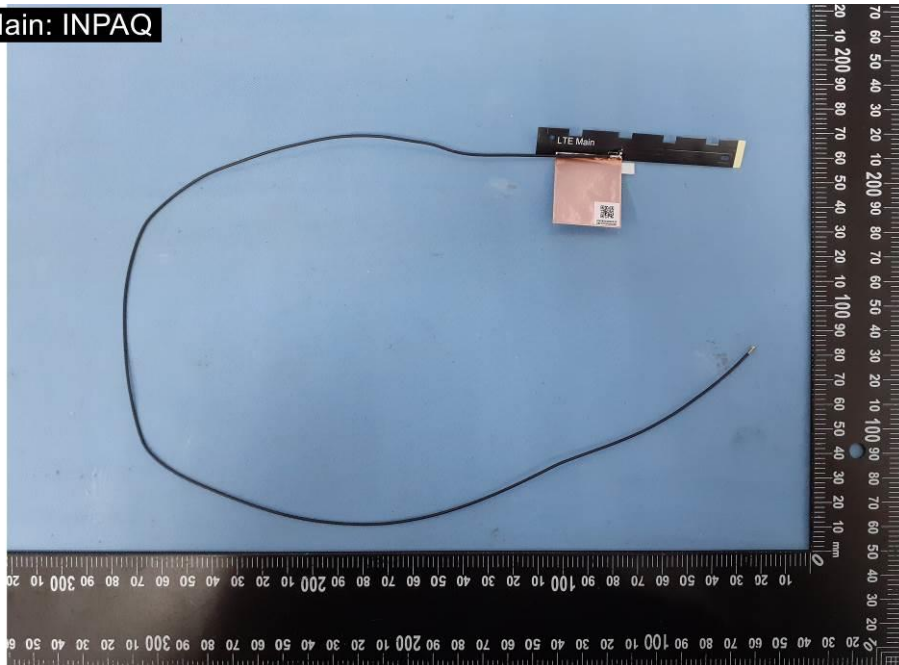
EUT Photo (26) WWAN antenna Main : INPAQ
