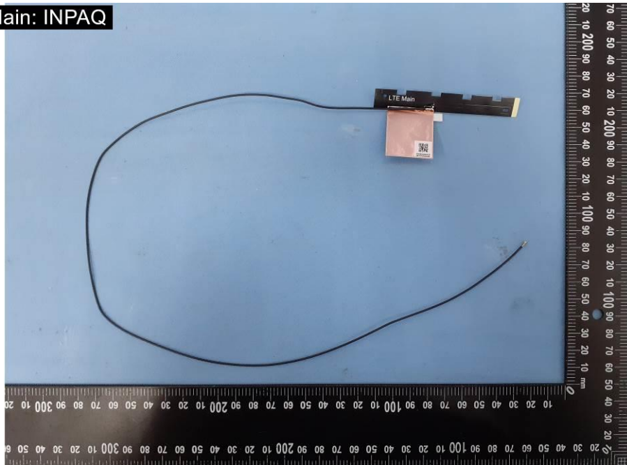
EUT Photo (26) WWAN antenna Main : INPAQ
