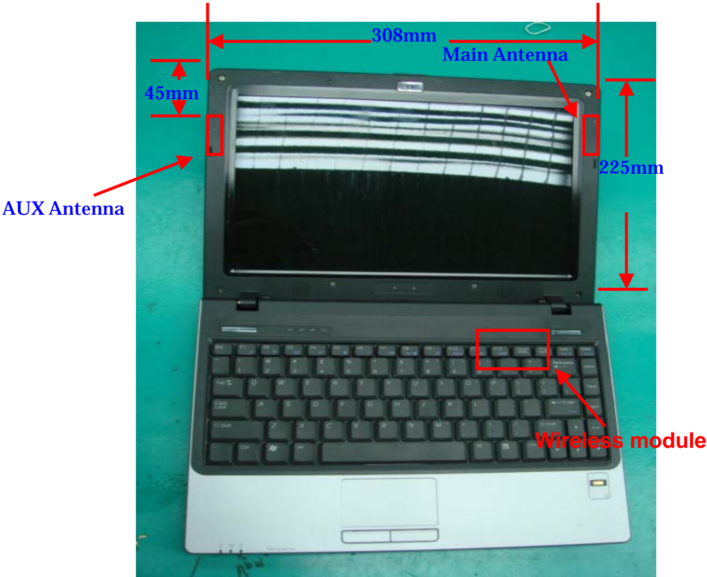
Main(side right) antenna
