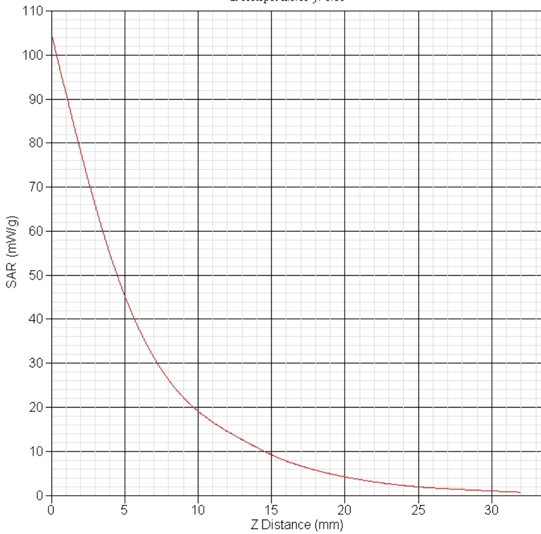
SAR-Z Axis at Hotspot x:0.05 y:-0.01
