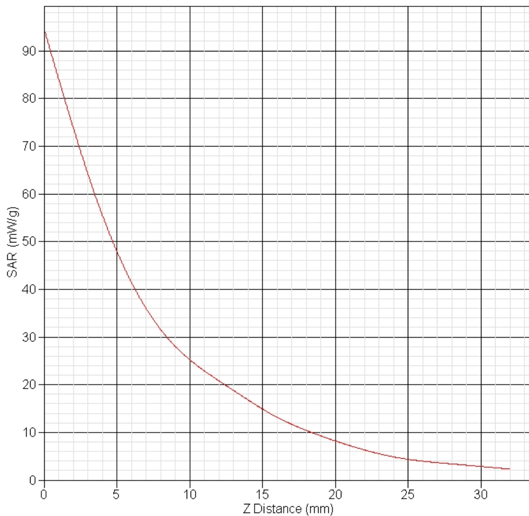
SAR-Z Axis at Hotspot x:0.12 y:-0.01
