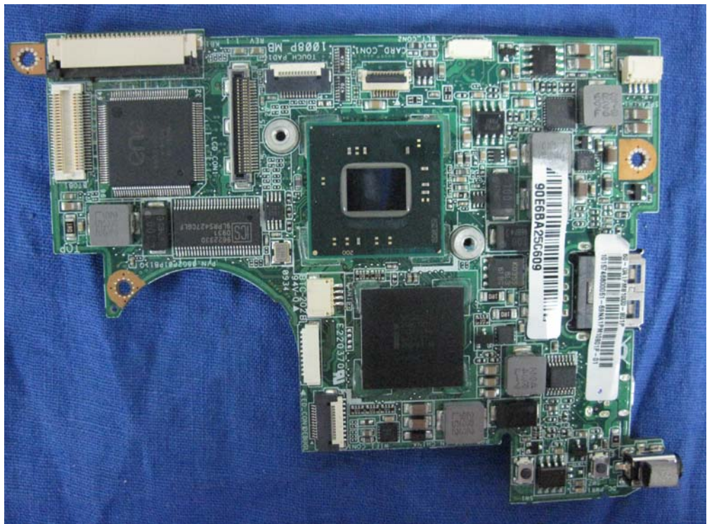
(11) EUT Photo
