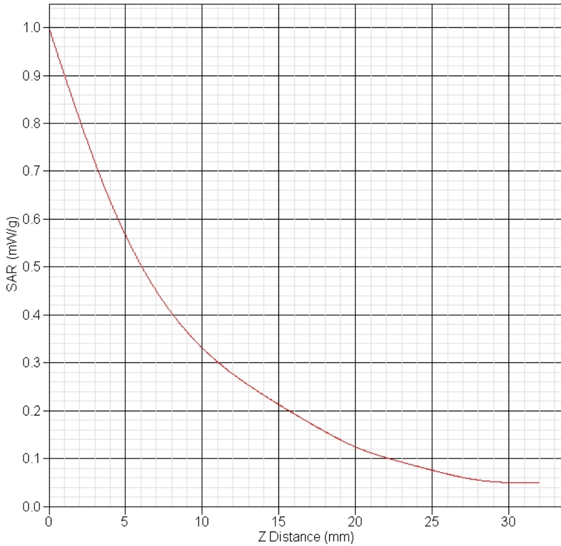
SAR-Z Axis at Hotspot x:37.07 y:-0.01
