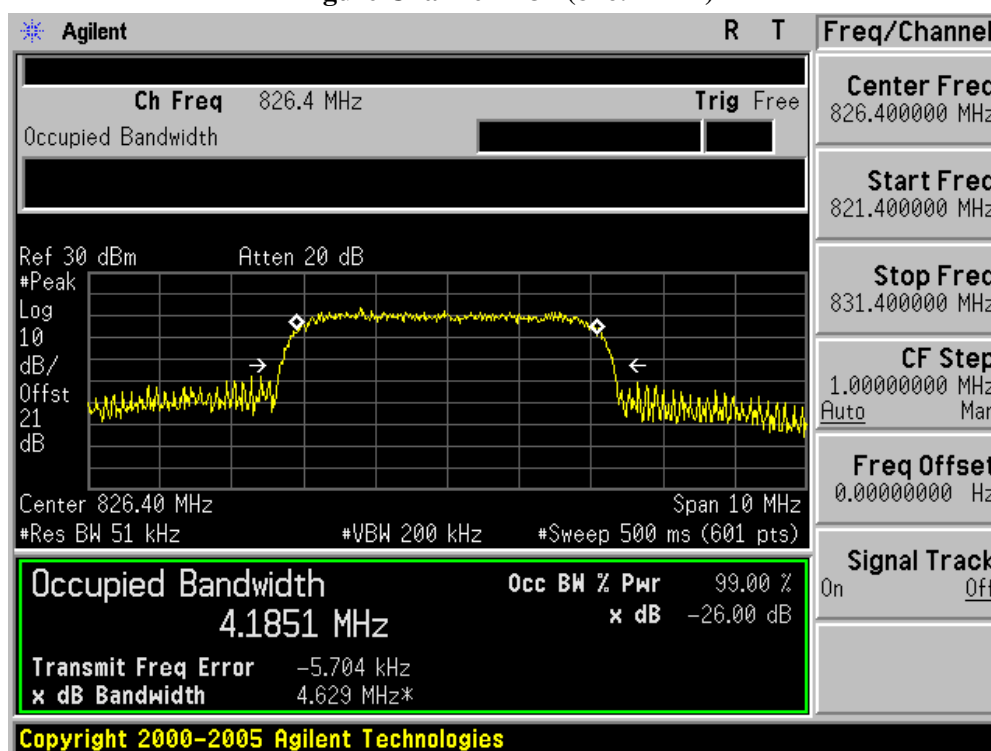
Figure Channel 4132 (826.4MHz)
