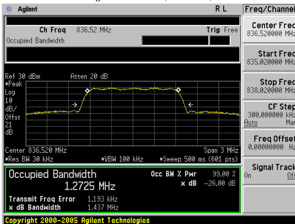
Figure Channel 384 (836.52MHz)
