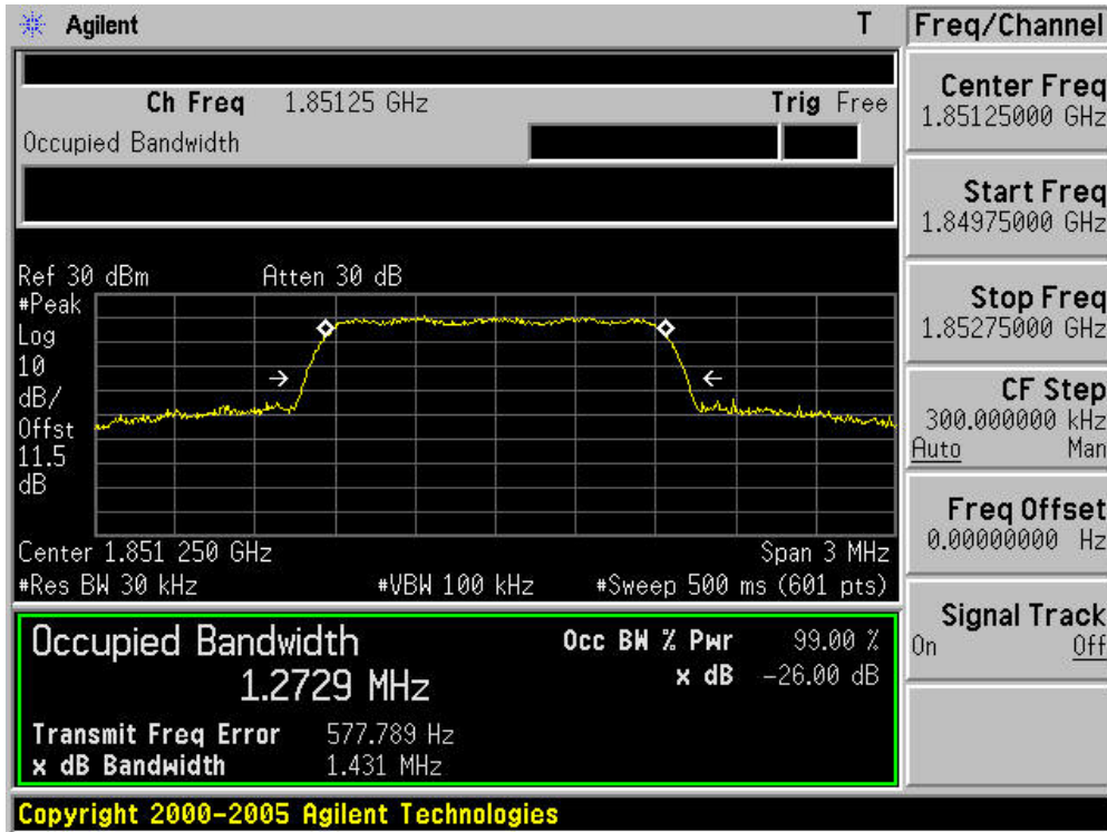
Figure Channel 25 (1851.25MHz)
