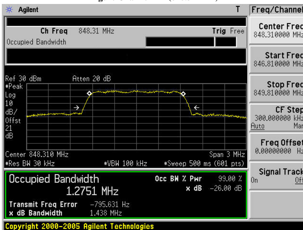
Figure Channel 777 (848.31MHz)
