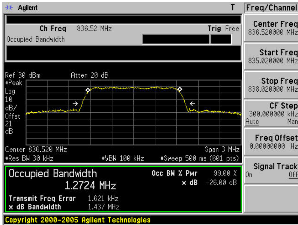
Figure Channel 384 (836.52MHz)
