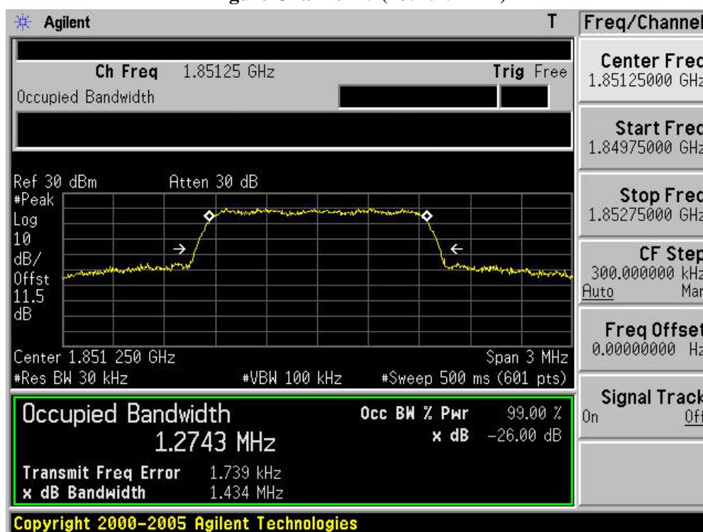
Figure Channel 25 (1851.25MHz)
