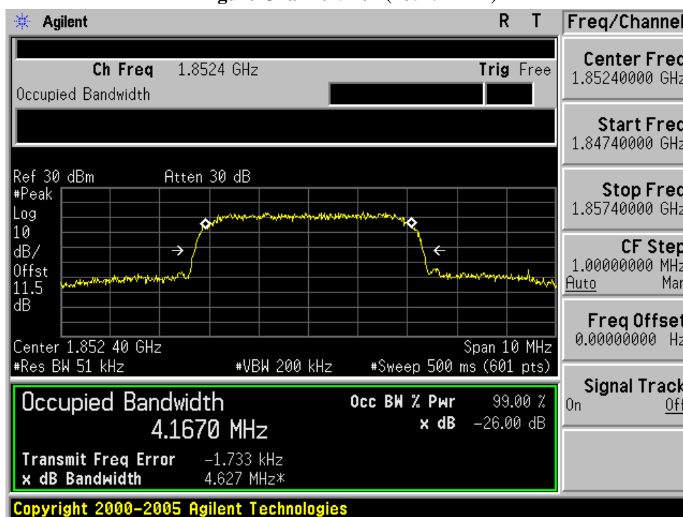
Figure Channel 9262 (1852.4MHz)
