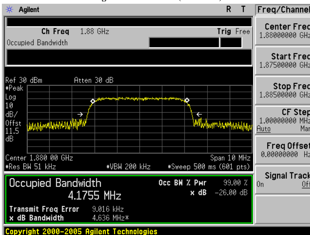
Figure Channel 9400 (1880MHz)
