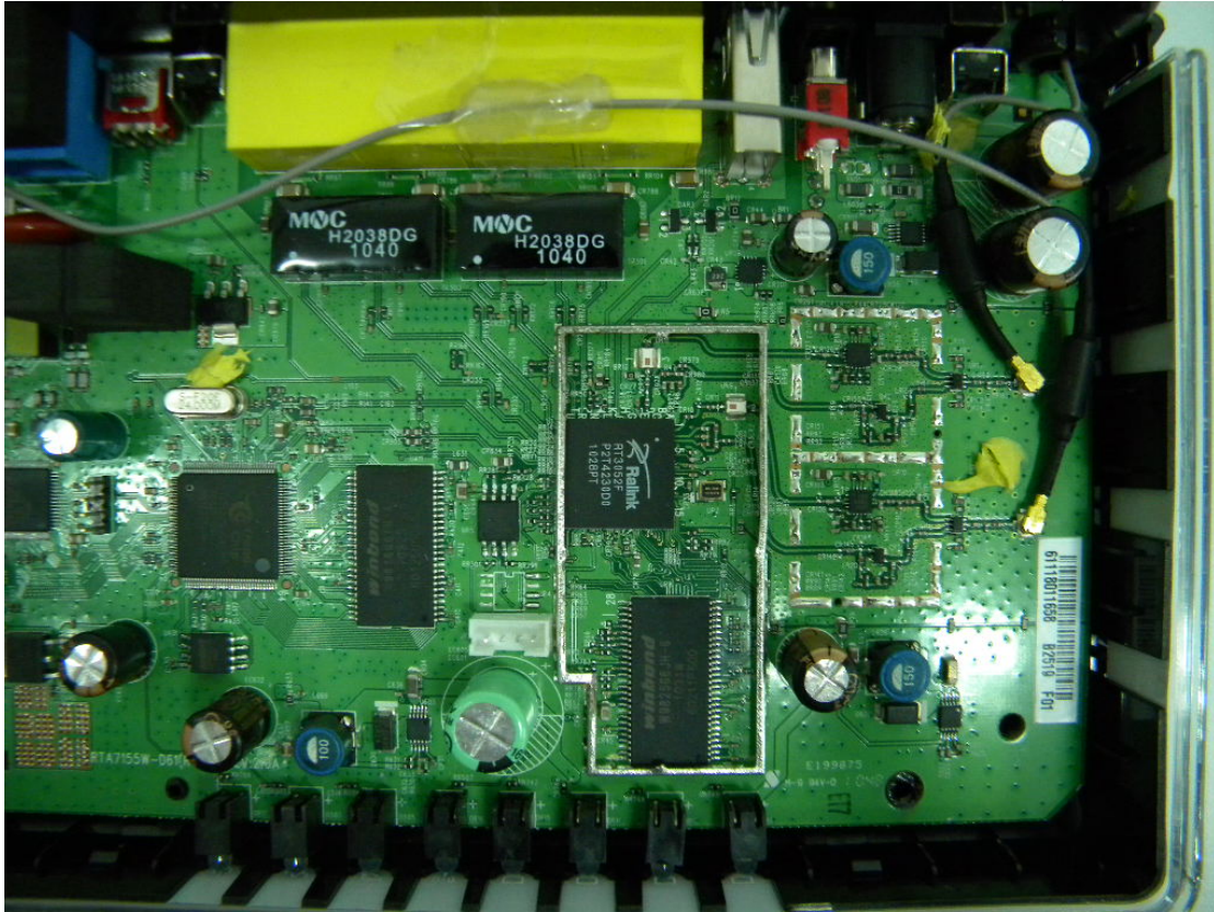
FIGURE 5 Main Board (Remove Shielding)
