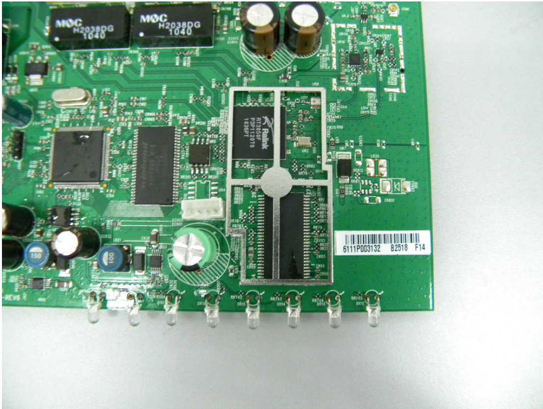
FIGURE 5 Remove Shielding
