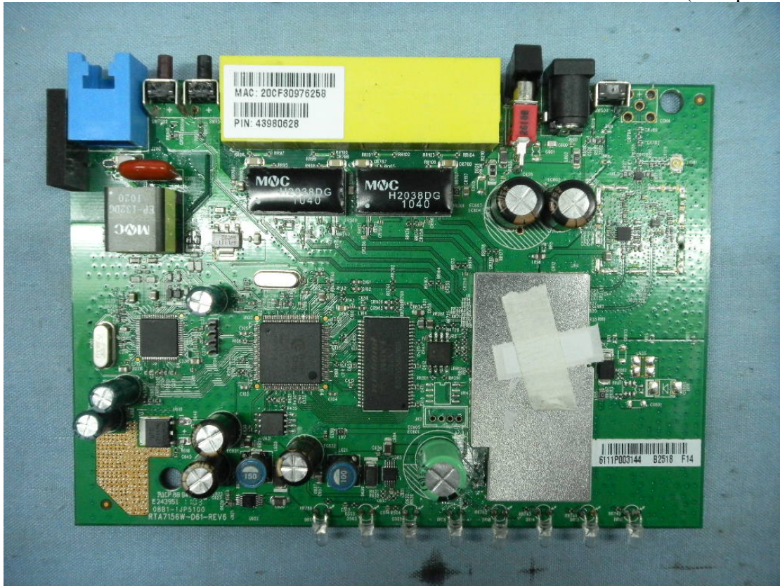
FIGURE 3 Main Board (Component View)
