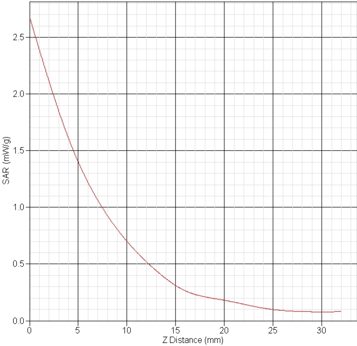
SAR-Z Axis at Hotspot x:0.10 y:-6.01
