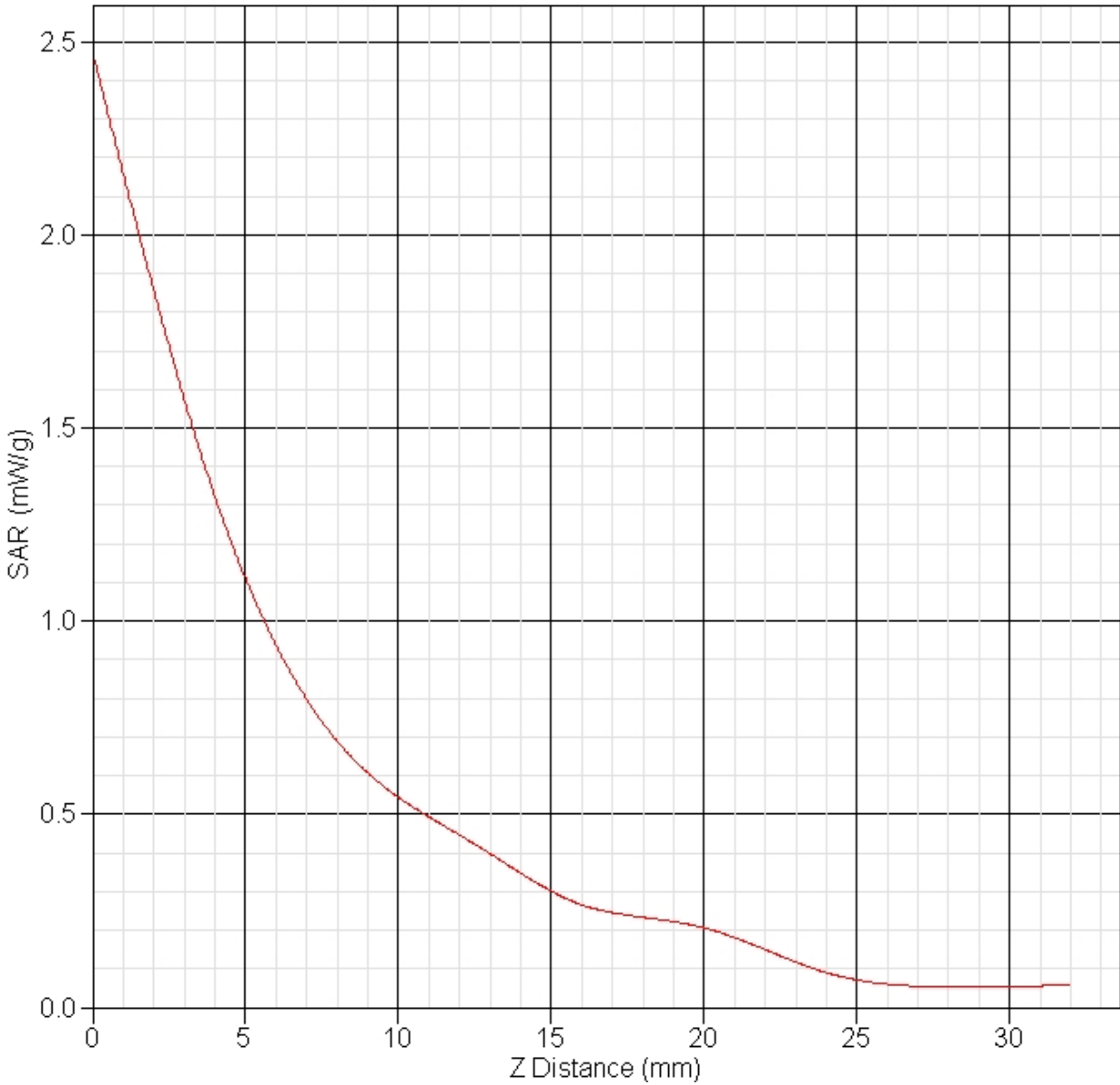
SAR-Z Axis at Hotspot x:0.08 y:-6.01
