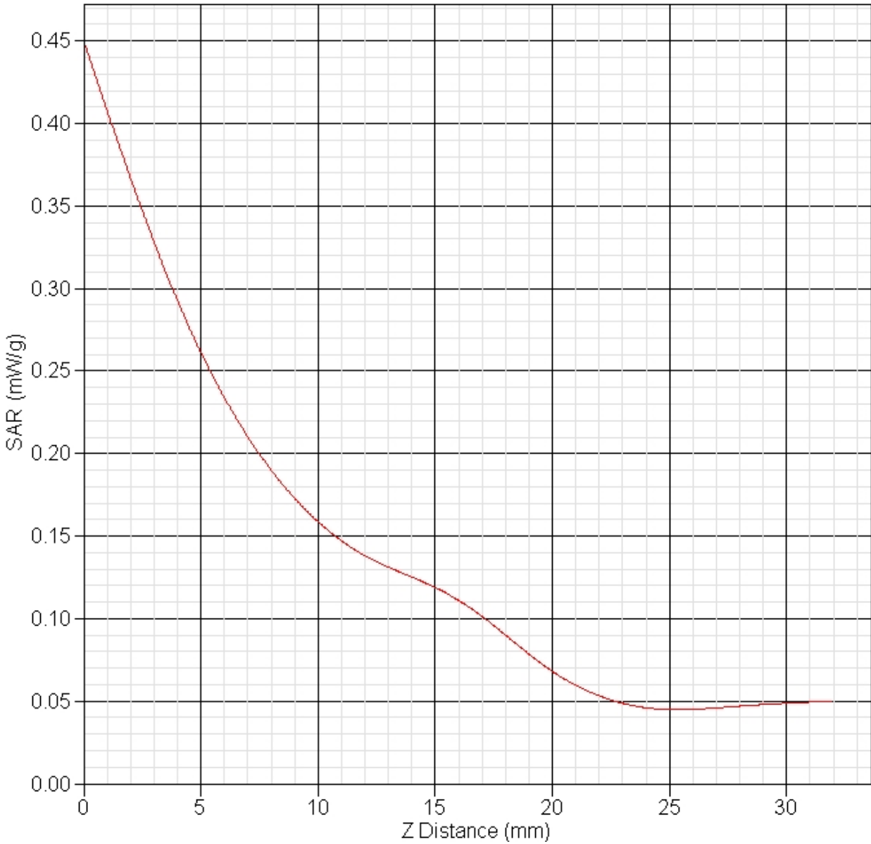
SAR-Z Axis at Hotspot x:4.14 y:9.83
