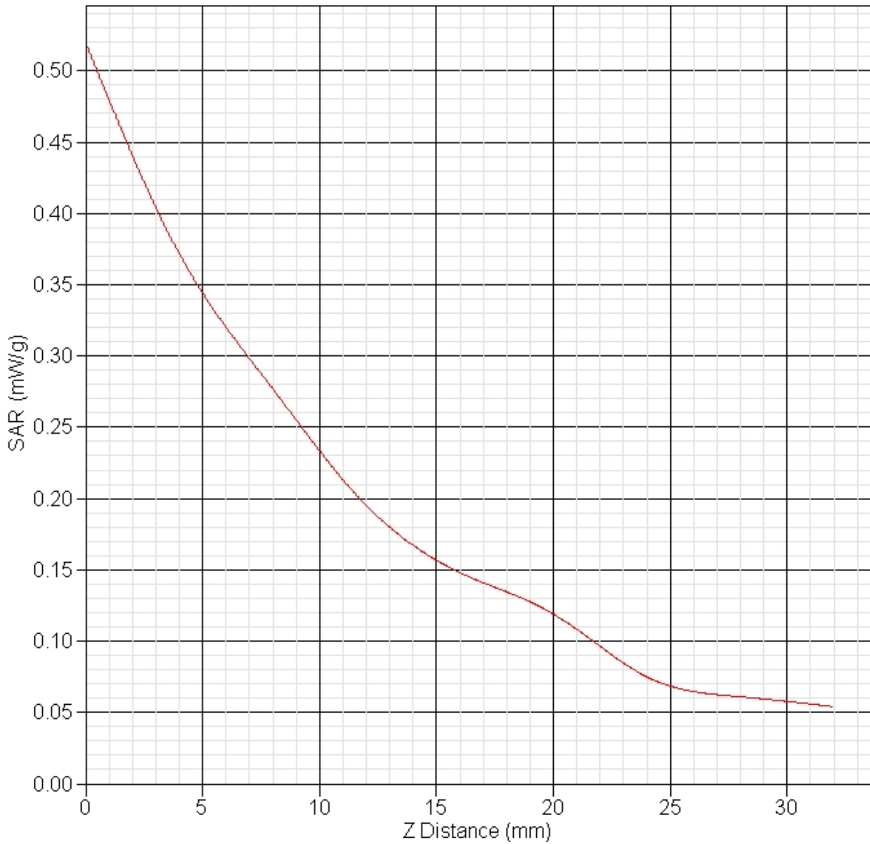
SAR-Z Axis at Hotspot x:12.04 y:-6.01
