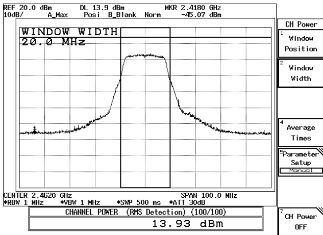
54Mbps-CH11
