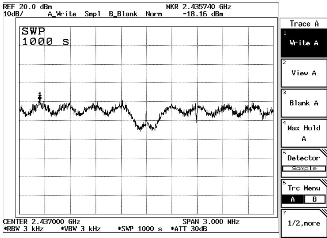
Figure Channel 6: 54Mbps
