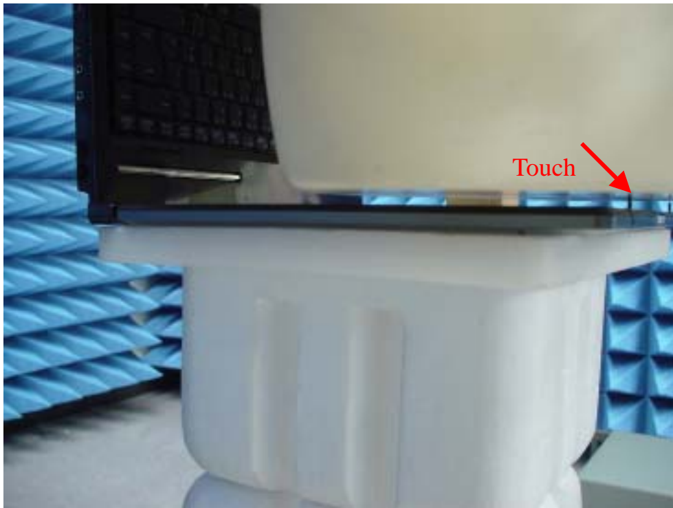
Fig.3 Photograph of the LCD Panel of Main Antenna contact to the flat phantom; and at a distance of 0.0 cm from the base of the phantom.
