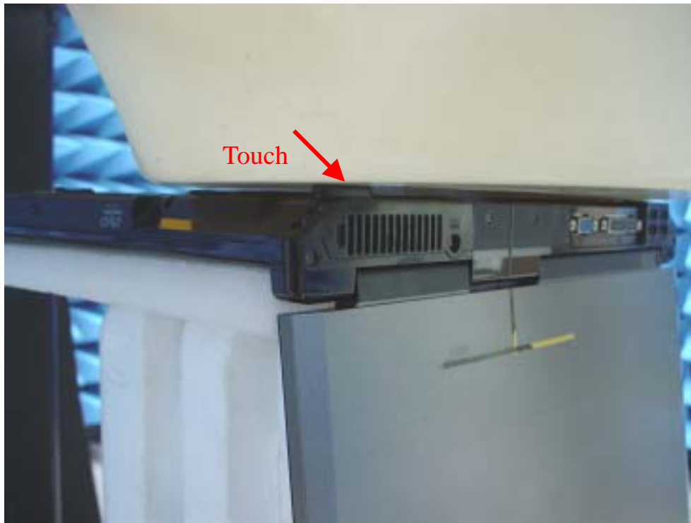
Fig.7 Photograph of the Bottom face of Auxiliary Antenna contact to the flat phantom; and at a distance of 0.0 cm from the base of the phantom.
