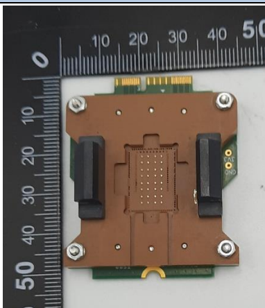
Socket Front
