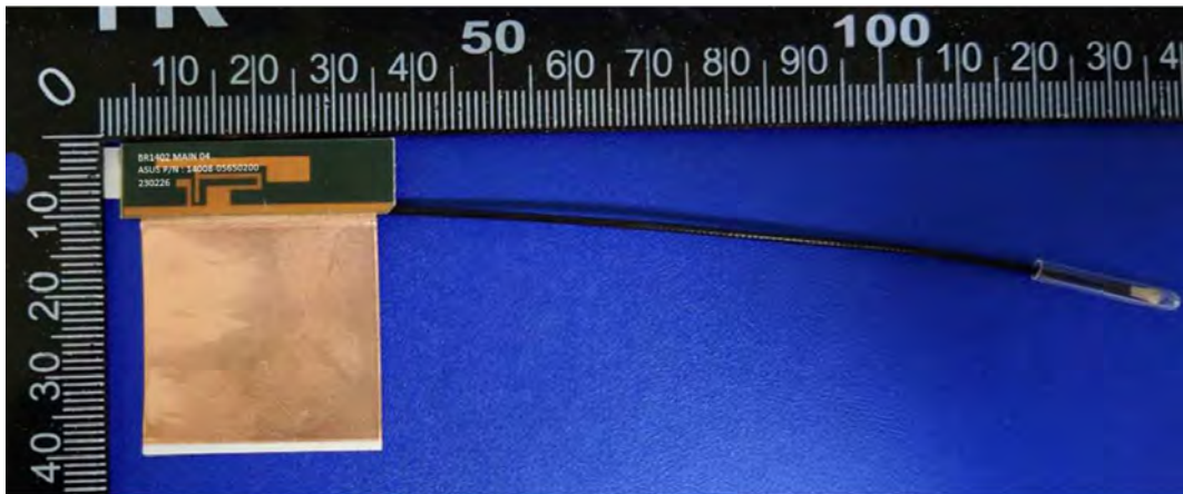
(30) EUT Photo (Manufacturer: PULSE, M/N: TZ2486E)
