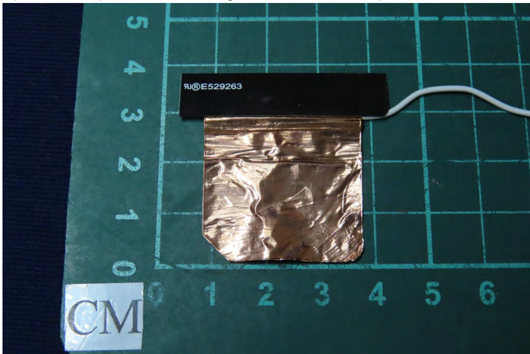
(28) EUT Photo (Manufacturer: INPAQ, M/N: WA-P-LE-01-045)
