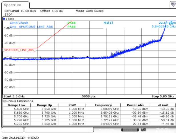
BE-NR-LOW, SISO-A, 802.11a20-6Mbps, Ch169
