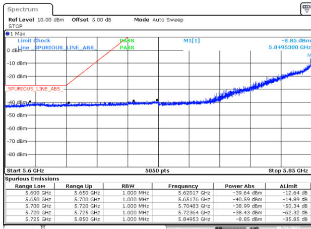
-BE-NR-LOW, SISO-A, 802.11n20-HT0, Ch173
