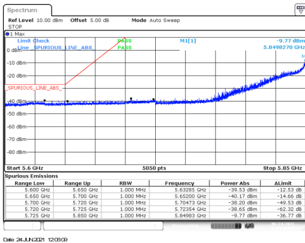
-BE-NR-LOW, SISO-A, 802.11a20-6Mbps, Ch173
