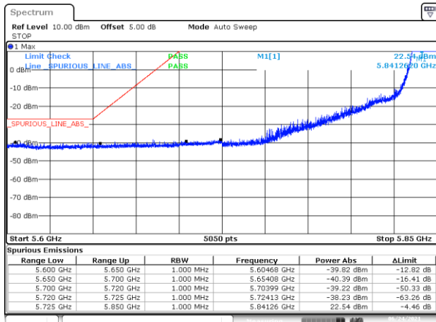
-BE-NR-LOW, SISO-A, 802.11n20-HT0, Ch169
