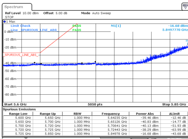
-BE-NR-LOW, SISO-A, 802.11n20-HT0, Ch177
